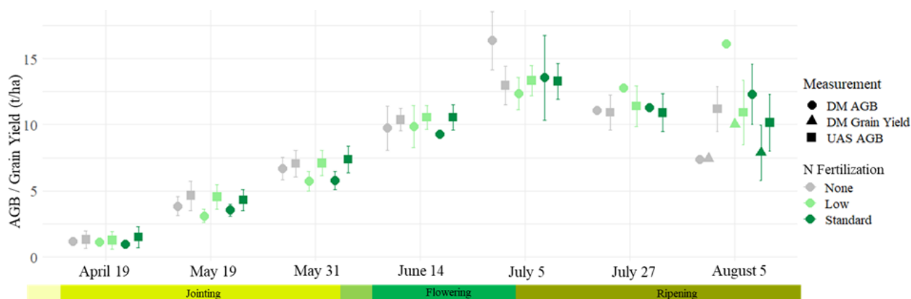
Figure 15. Comparison of UAV-derived above-ground biomass (AGB), destructive AGB measurements, and grain yield across nitrogen fertilization treatments throughout the winter wheat growing season. UAV estimates were generated using the combined crop height (CH), 5 layer gap fraction (GF), and field-normalized LiDAR intensity (INT) model and represent the entire treatment plots, whereas destructive AGB measurements were obtained from discrete subplot sampling locations. Error bars indicate \pm SD within each nitrogen treatment. The figure illustrates the ability of UAV observations to capture seasonal biomass dynamics and nitrogen treatment responses while providing spatially continuous estimates beyond the limited destructive sampling locations.
