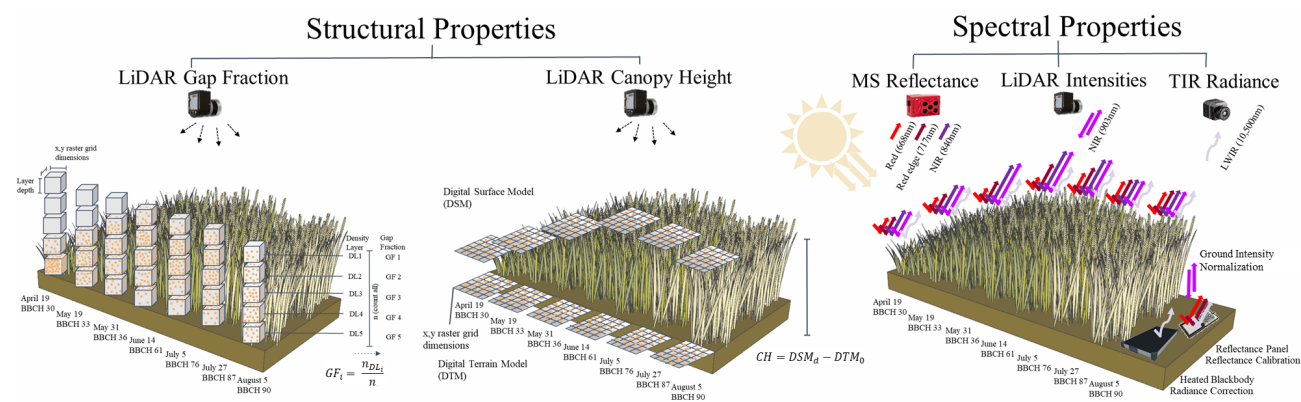
Figure 5. Conceptual representation of the UAV-derived feature groups evaluated in this study. LiDAR gap fraction and crop height represent predominantly structural canopy properties, whereas multispectral reflectance, normalized LiDAR intensity, and thermal radiance provide complementary wavelength-dependent responses influenced by both canopy structure and vegetation surface properties.
