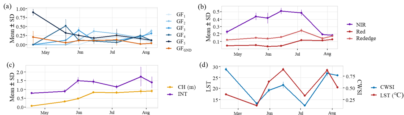
Figure B2. Temporal evolution of UAV-derived canopy features throughout the winter wheat growing season. Mean values ( \pm SD) are shown for (a) the five 20 cm LiDAR multi-layer gap fraction layers ( GF_1 – GF_5 ) together with the conventional ground-based gap fraction ( GF_{GND} ), (b) multispectral reflectance bands (Red, Red-edge, and NIR), (c) LiDAR maximum crop height (CH) and normalized LiDAR intensity (INT), and (d) thermal products including the Crop Water Stress Index (CWSI) and land surface temperature (LST). The temporal trajectories illustrate changes in canopy structure, spectral response, LiDAR intensity, and thermal status across the growing season, providing context for the observed phenological shifts in sensor contributions to above-ground biomass estimation.
