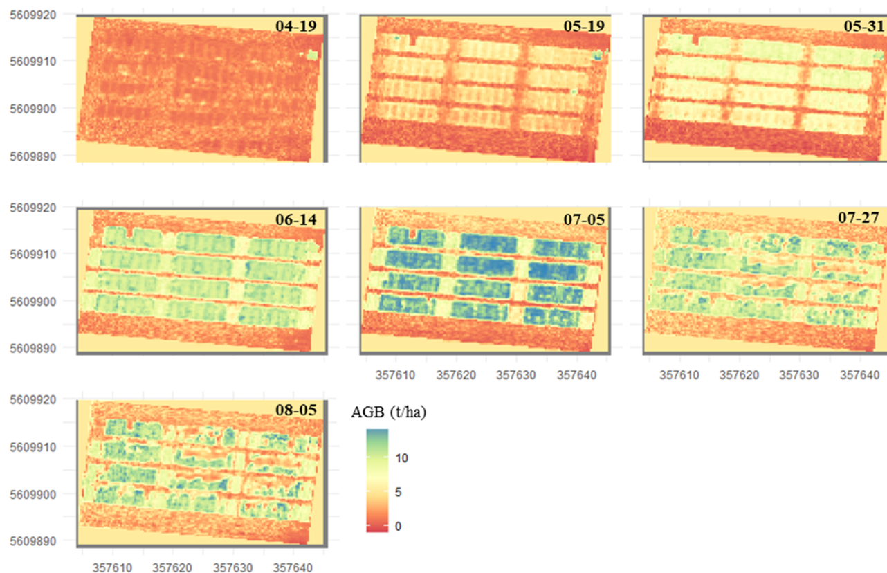
Figure B11. AGB maps generated for each UAV acquisition date using the combined LiDAR-derived crop height (CH), 5 layer gap fraction (GF; 20 cm layer depth), and field-normalized LiDAR intensity (INT) ANN model. Values are displayed on a common color scale ( \text{t ha}^{-1} ), illustrating the temporal progression of spatial variability in biomass accumulation. The high-resolution maps demonstrate the capability of UAV LiDAR features to provide spatially continuous biomass estimates beyond the discrete locations available from destructive sampling.
