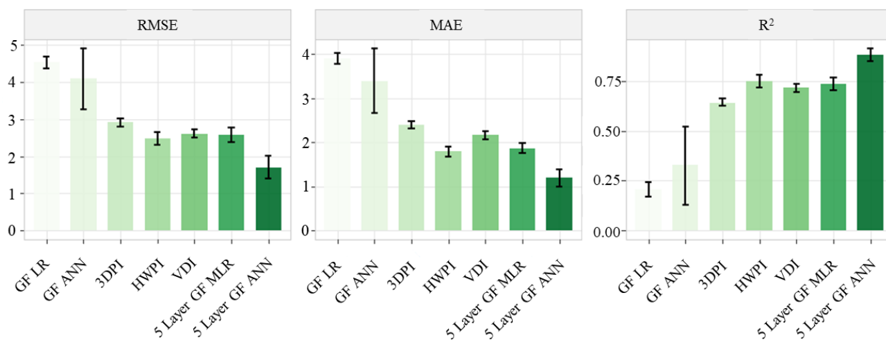
Figure 8. Comparison of cross-validation (10-fold) performance for LiDAR canopy density methods using the optimal GF parameterization identified in Fig. 7 (five 20 cm vertical layers and 30 cm GSD). Conventional single layer ground gap fraction (GF LR) was used as the baseline and compared with ANN using single GF (GF ANN), engineered multi-layer density indices (3DPI, HWPI, and VDI), multiple linear regression using the 5 layer GF (DL MLR), and the proposed 5 layer GF ANN approach. Bars represent mean performance across folds and error bars indicate variability among folds.
