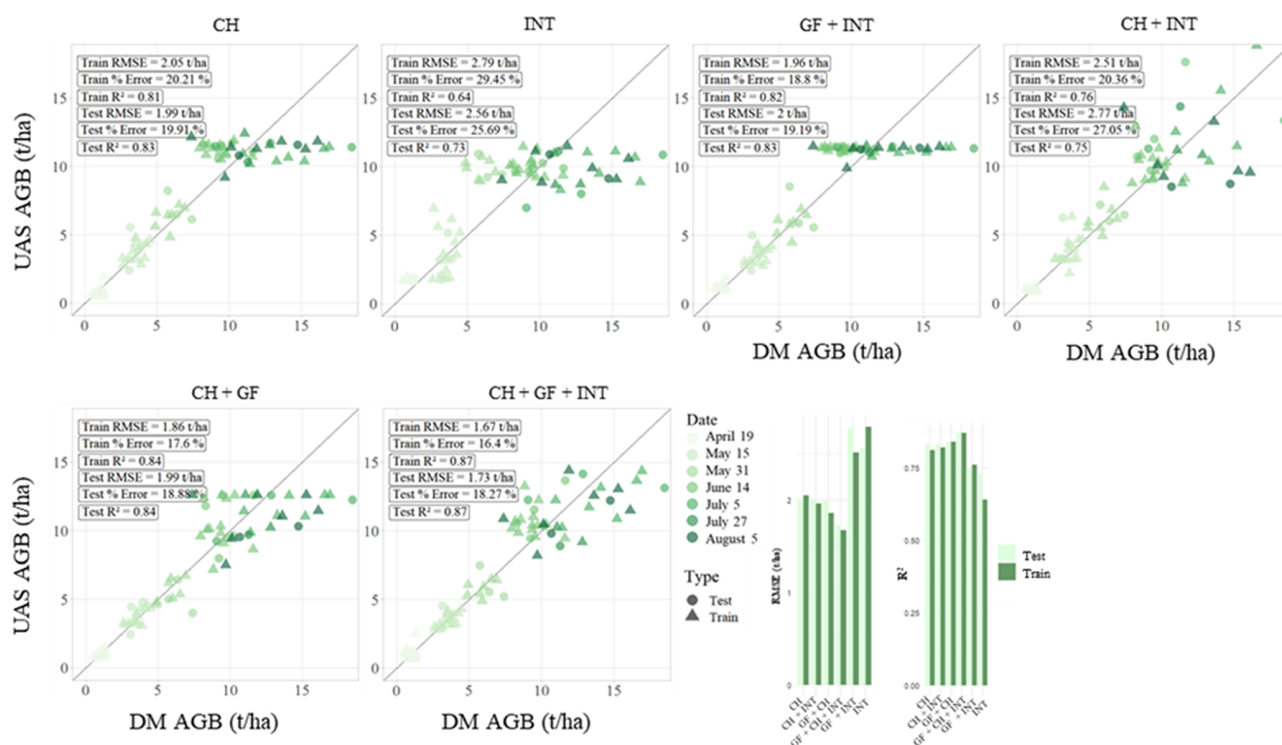
Figure B7. Observed versus predicted above-ground biomass (AGB) for ANN models using different combinations of LiDAR-derived crop height (CH), 5 layer gap fraction (GF) (20 cm layer depth), and field-normalized LiDAR intensity (INT). All models were generated using the optimal 30 cm ground sampling distance (GSD) identified in the GF sensitivity analysis. Marker color indicates acquisition date and marker shape distinguishes training and testing samples. Training and testing RMSE, relative error, and R^2 are reported within each panel. The accompanying summary plots compare testing RMSE and R^2 across the evaluated LiDAR feature combinations, illustrating the progressive improvement obtained by incorporating complementary canopy density and normalized intensity information alongside crop height.
