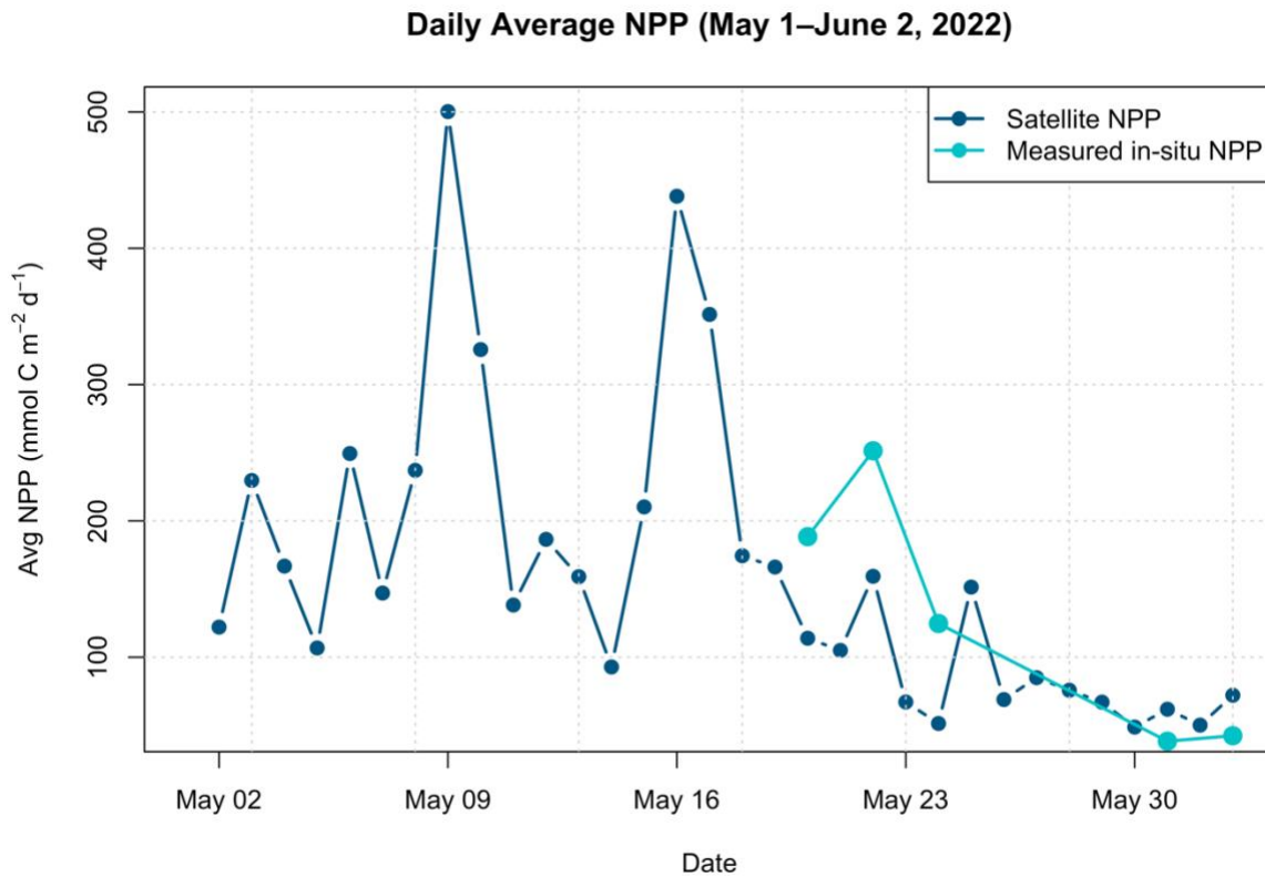
Fig. S5. Satellite net primary production (NPP) and measured in situ NPP in the Eastern Grid area from 2 May to 2 June 2022. Satellite NPP data was supplied by the Satellite Ocean colour and Phytoplankton Ecology group (SOPhyE) at the Bedford Institute of Oceanography, reported in Devred et al. (2025). Measured in situ NPP reflects the NPP integrated rates (from 13 C incubations) measured during the BELAS-1 expedition (see Fig. 3). Satellite NPP reflects integrated NPP down to the depth of 1% surface photosynthetic active radiation, while measured in situ NPP reflects integrated NPP down to the base of the primary production zone (Owens et al., 2015).
