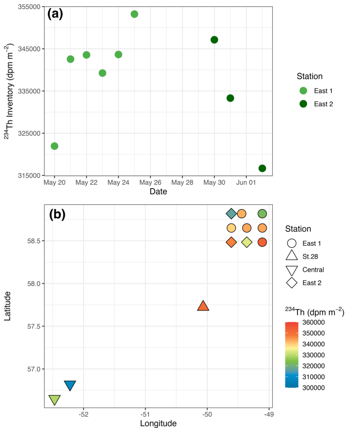
Fig. S3. ^{234}\text{Th} inventories in the upper 150 m of the water column in the Eastern Grid vs. time (a) and across all stations sampled during the BELAS-1 expedition (b).
