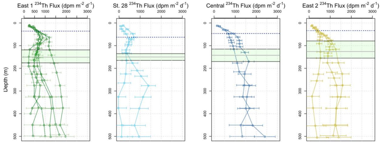
Fig. S6. Profiles of steady state ^{234}\text{Th} flux across regions. The base of the primary production zone is shown with green shading (grey solid line indicates the average, black solid lines indicate the minimum and maximum) and the average base of the mixed layer is shown with a blue dashed line.
