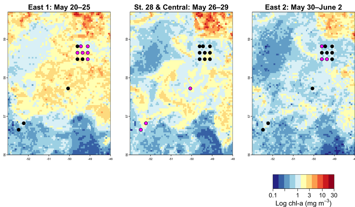
Figure 2. Satellite-derived chlorophyll a (chl a ) concentrations (Devred et al., 2025) at the time of sampling of East 1 stations (left panel), Station 28 and central stations (middle panel), and East 2 stations (right panel).
