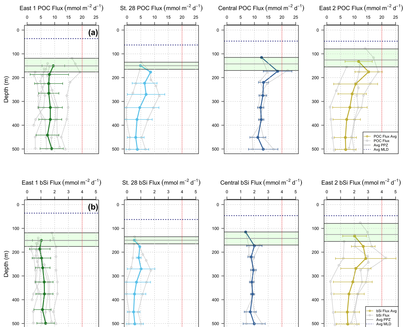
Figure 6. Profiles of particulate organic carbon (POC, panel a ) and biogenic silica (bSi, panel b ) flux across regions. Fluxes measured at individual stations are shown in grey, whereas averages are shown in color (green for East 1, light blue for St. 28, dark blue for Central, yellow for East 2). The vertical red lines at 20 \text{ mmol C m}^{-2} \text{ d}^{-1} for POC and 4 \text{ mmol Si m}^{-2} \text{ d}^{-1} for bSi are for visual reference. The base of the primary production zone (PPZ) is shown with green shading (grey solid line indicates the average, black solid lines indicate the minimum and maximum) and the average base of the mixed layer (MLD) is shown with a blue dashed line.
