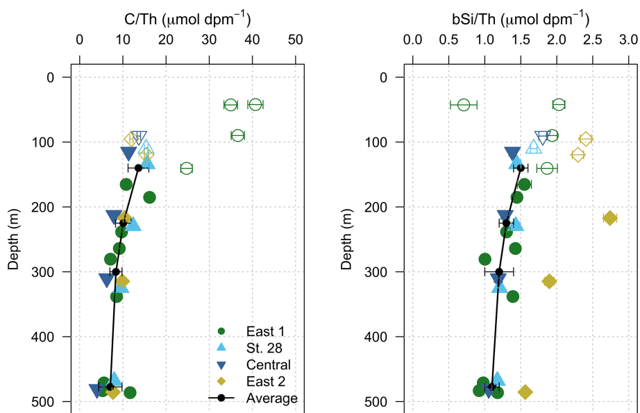
Figure 5. Profiles of POC / ^{234}\text{Th} (C / Th) and bSi / ^{234}\text{Th} (bSi / Th) ratios in >51\ \mu\text{m} particles across regions. Black symbols denote average C / Th ratios (all stations) and average bSi / Th ratios (all stations except East 2) for the following depth horizons: 115–185, 210–240, 260–340, 465–490 m. Empty symbols denote samples collected within the primary production zone. Analytical uncertainties are represented by horizontal bars and uncertainties less than \sim 3\ \mu\text{mol dpm}^{-1} are not visible against filled symbols. POC = particulate organic carbon, bSi = biogenic silica.
