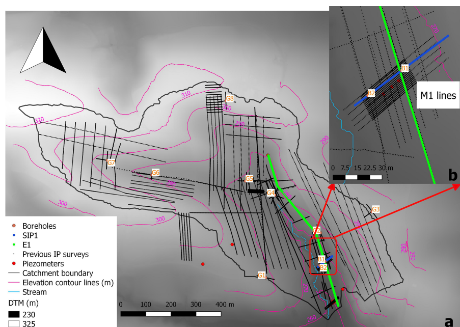
Figure B1. Existing surface and subsurface information at the HOAL: (a) The topography changes are indicated in the grey tones and the isolines (pink lines), available CC measurements (black lines) and boreholes (G1 to G8). The embedded plot (b) highlights the orientation of the CC lines presented in this study: exploration results (E1 with the green line), the multi-frequency measurements (SIP1 with the blue line) and mapping measurements (M1 indicated with the black lines) as well as the boreholes B1 and B2 drilled for sampling and geochemical analysis of soil samples in the electrical anomaly.
