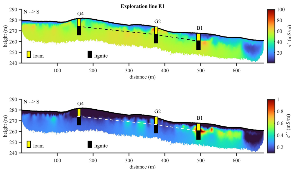
Figure 1. CC imaging results obtained for the Exploration line E1, expressed in terms of the conductivity ( \sigma' ) and polarization ( \sigma'' ). The information about lithological changes observed in soil samples extracted from existing boreholes G4 and G2, as well as the drilled borehole for this study (B1), is imposed on the electrical images for comparison. The dashed line represents the depth to the lignite layer from the linear interpolation of the borehole data.
