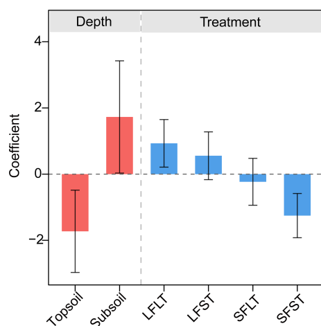
Figure 6. The effects of DOC on R_s . Bars show the random-slope deviations of the DOC effect on R_s relative to the overall fixed slope, based on the linear mixed-effects model R_s \sim \text{DOC} + (1 + \text{DOC} | \text{Treatment}) + (1 + \text{DOC} | \text{depth}) , where DOC denotes mean-centred DOC. The model was fitted using all observations collected during the thawing phases throughout the entire freeze-thaw incubation period ( n = 168 ). Positive values indicate a stronger DOC– R_s relationship than the overall average, whereas negative values indicate a weaker relationship. Error bars represent 95 % confidence interval.
