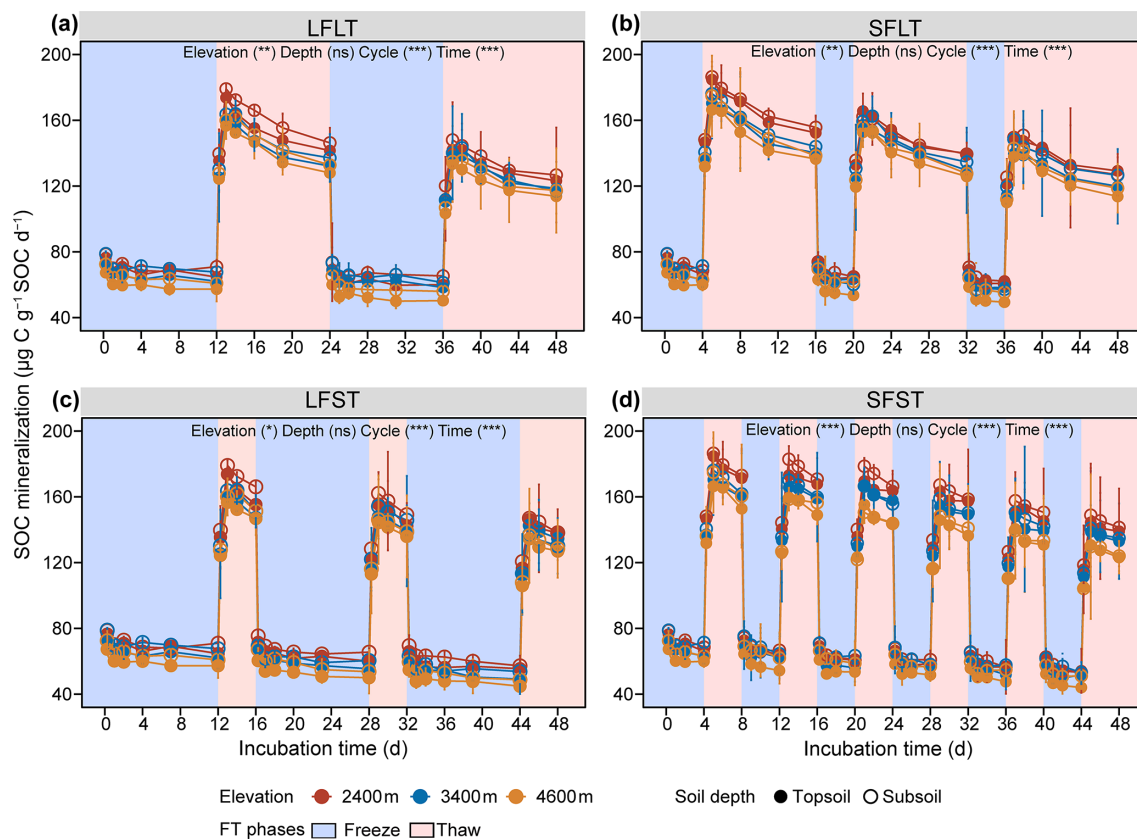
Figure 1. Soil organic carbon (SOC) mineralization rate during freeze-thaw cycle incubation. Soil was incubated for 48 d under two temperature conditions: −10 °C (Freeze) and 10 °C (Thaw). Four distinct freeze-thaw cycle patterns were designed to address knowledge gaps in previous studies, based on two cycle durations: 12 d (long) and 4 d (short). Panels (a)–(d) show the temporal dynamics of SOC mineralization under the four freeze-thaw regimes: (a) long freeze-long thaw (LFLT), (b) short freeze-long thaw (SFLT), (c) long freeze-short thaw (LFST), and (d) short freeze-short thaw (SFST). The blue and red background areas denote freezing (−10 °C) and thawing (10 °C) phases, respectively. Data points represent treatment means \pm 1 SE ( n = 3 ). Significance tests compare elevations, soil depths, cycle number, and incubation time during thaw periods (* p < 0.05 ; ** p < 0.01 ; *** p < 0.001 ).
