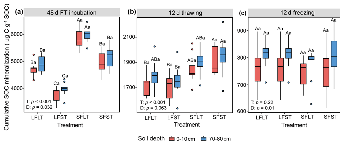
Figure 2. Cumulative soil organic carbon (SOC) mineralization under different freeze-thaw regimes and soil depths. (a) Cumulative SOC mineralization over the full 48 d freeze-thaw incubation. (b) SOC mineralization over the same 12 cumulative thaw days. (c) SOC mineralization over the same 12 cumulative freeze days. Bars represent cumulative SOC mineralization for topsoil (0–10 cm) and subsoil (70–80 cm) under each freeze-thaw treatment. Error bars indicate \pm 1 SE ( n = 18 ). Uppercase letters denote significant differences among treatments within a given depth (Tukey's HSD), and lowercase letters indicate significant differences between depths within a given treatment.
