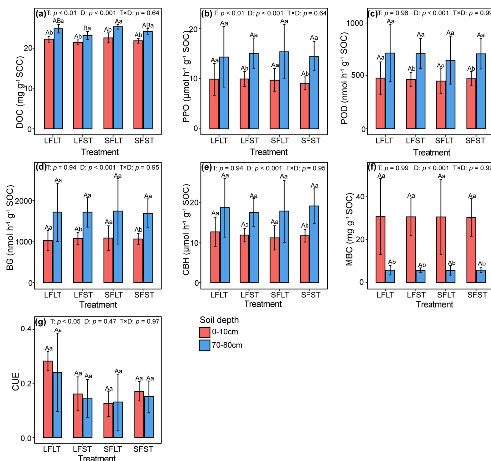
Figure 3. Effects of freeze-thaw regimes on dissolved organic, enzyme activities, and microbial properties across two soil depths. Panels (a)–(g) show dissolved organic carbon (DOC), polyphenol oxidase activity (PPO), peroxidase activity (POD), \beta -glucosidase activity (BG), cellobiohydrolase activity (CBH), microbial biomass carbon (MBC), and carbon use efficiency (CUE), respectively. Error bars indicate the variability among the repeated observations used to calculate each treatment mean, rather than independent biological replication among separate jars. Specifically, for the LFLT and SFLT treatments, n = 3 corresponds to measurements taken on the first day of thawing in the first freeze-thaw cycle, whereas for the LFST and SFST treatments, n = 9 corresponds to measurements taken on the first day of thawing across the first to third freeze-thaw cycles. Different uppercase letters indicate significant differences among treatments within the same soil depth, whereas different lowercase letters indicate significant differences between soil depths within the same treatment (Tukey's multiple comparison test).
