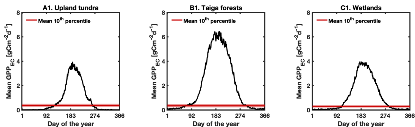
Figure B2. Mean seasonal cycle of daily averaged eddy covariance (EC) gross primary production ( \text{GPP}_{\text{EC}} ) for upland tundra, taiga forests and wetlands. The horizontal red line indicates the estimated separation between dormant and transitional periods with active photosynthetic periods (i.e., the growing season) using a percentile-based \text{GPP}_{\text{EC}} threshold (Sect. 4.2). This threshold corresponds to the mean 10th percentile computed across EC towers, with the 5th and 15th percentiles shown as variability bounds.
