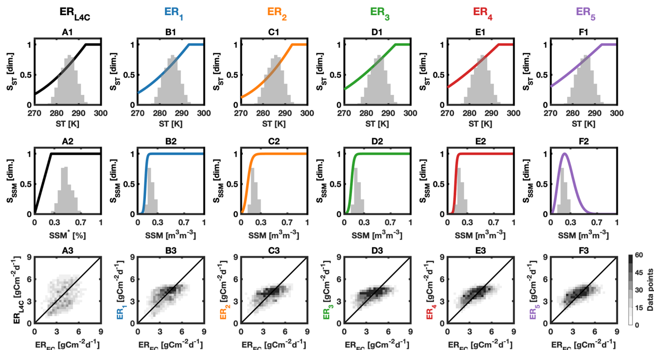
Figure 6. Same as Fig. 5, but for taiga forests . The spatiotemporal comparison includes all available ER_{EC} data points for taiga forests after filtering, including those used for calibration (4632 data points; Sect. 4.3). GPP_5 was used as input for ER_1 through ER_5 (Sect. 5.2.2).
