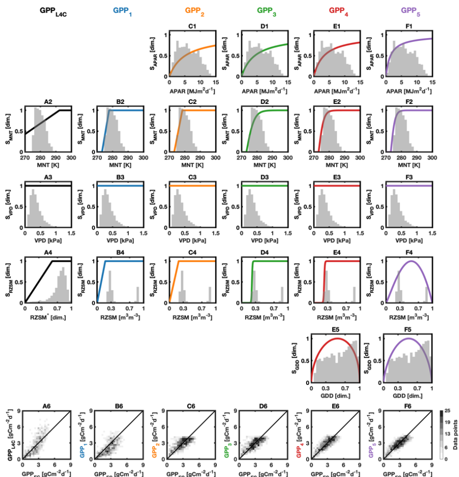
Figure 2. Ecosystem responses used to compute modeled gross primary production ( GPP ) from the L4C model ( GPP_{L4C} , column A) and from the Arctic-Subarctic (AS) adapted formulations ( GPP_1 through GPP_5 , columns B–F) in upland tundra during the growing season. The ecosystem responses are expressed as stress scalars, S_x , for each environmental variable x , where x represents absorbed photosynthetically active radiation (APAR), minimum air temperature (MNT), vapor pressure deficit (VPD), root zone soil moisture (RZSM), and normalized growing degree days (GDD). In the background of each subplot, the histogram of the corresponding environmental variable is shown in light grey. All ecosystem responses of a given model formulation are calibrated jointly using eddy covariance GPP ( GPP_{EC} ) as reference, and not based on the histogram values. In subplot A4, RZSM* refers to the normalized RZSM used as input in the original L4C model. Subplots A1 and B1 are omitted because APAR is used as a direct input, rather than through a stress scalar, in GPP_{L4C} and GPP_1 formulations. Similarly, subplots A5–D5 are omitted because GDD is not used as input in the GPP_{L4C} , GPP_1 , GPP_2 , and GPP_3 formulations. Refer to Sects. 3 and 4.1 for a detailed description of each model formulation. The last row displays scatter plots between modeled GPP against GPP_{EC} . It is a spatiotemporal comparison, accounting for both temporal and spatial variability. It includes all available GPP_{EC} data points for upland tundra after filtering, including those used for calibration (1650 data points; Sect. 4.3).
