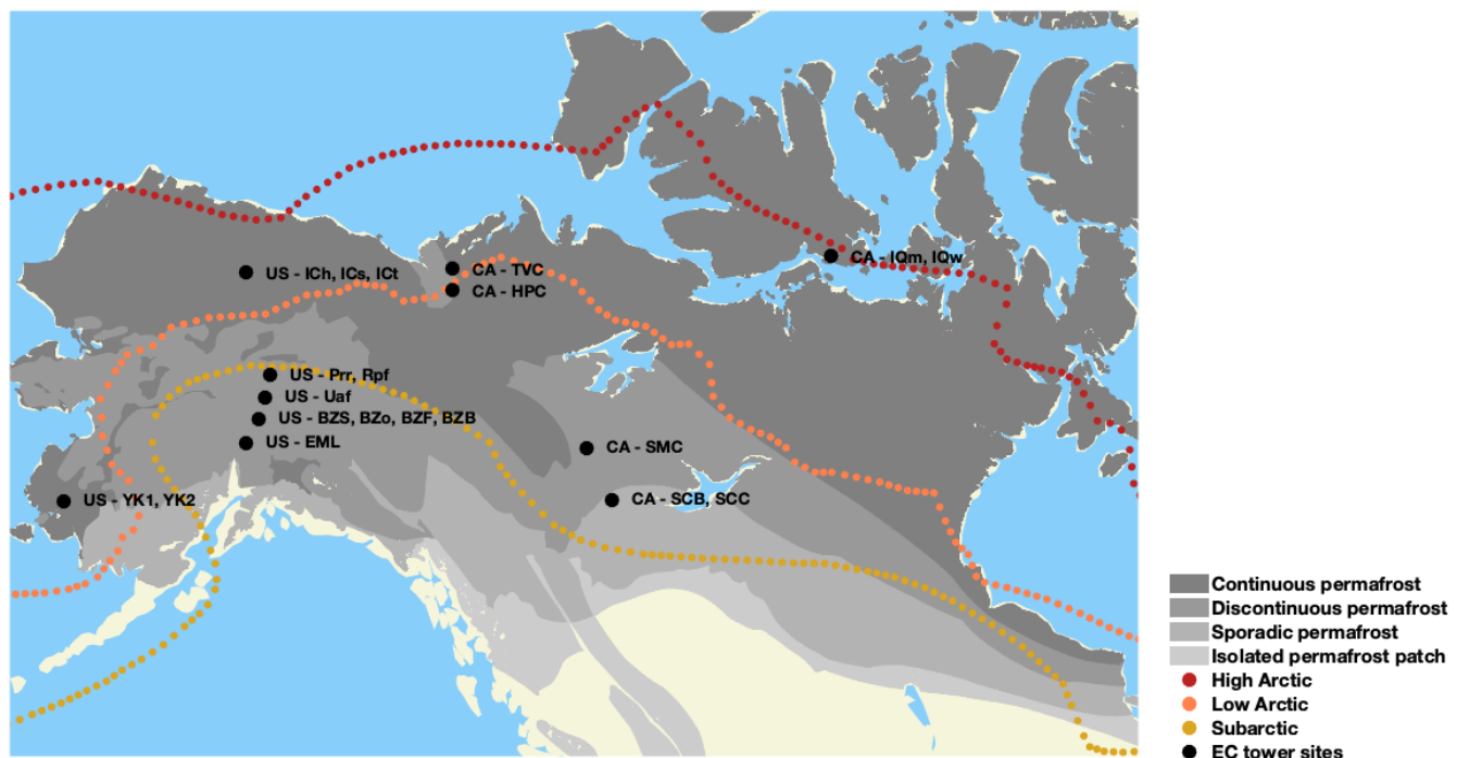
Figure 1. Locations of the 20 eddy covariance (EC) towers providing measurements of net ecosystem CO 2 exchange (NEE EC ), NEE-derived gross primary production (GPP EC ) and ecosystem respiration (ER EC ) from April 2015 to December 2022. The High Arctic, Low Arctic and Subarctic zones were delineated following the Conservation of Arctic Flora and Fauna (CAFF) working group of the Arctic Council, using Moderate Resolution Imaging Spectroradiometer (MODIS) and Landsat imagery (Potapov et al., 2008). The permafrost extent is estimated in percent areal coverage (Brown et al., 2002): continuous (> 90 %–100 % areal extent), discontinuous (> 50 %–90 %), sporadic (10 %–50 %) and isolated patches (< 10 %). Due to overlapping, a single color dot may represent up to four EC towers on the map. Information for each EC tower is listed in Table 1. The figure was inspired by Madelon et al. (2025) and Mavrovic et al. (2023a).
