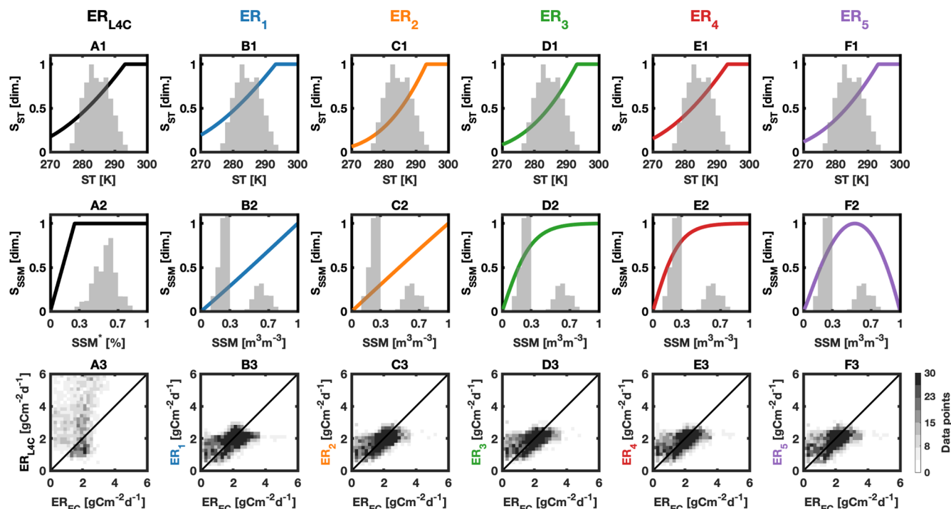
Figure 7. Same as Fig. 5, but for wetlands . The spatiotemporal comparison includes all available ER_{EC} data points for wetlands after filtering, including those used for calibration (3653 data points; Sect. 4.3). GPP_4 was used as input for ER_1 through ER_5 (Sect. 5.2.3).
