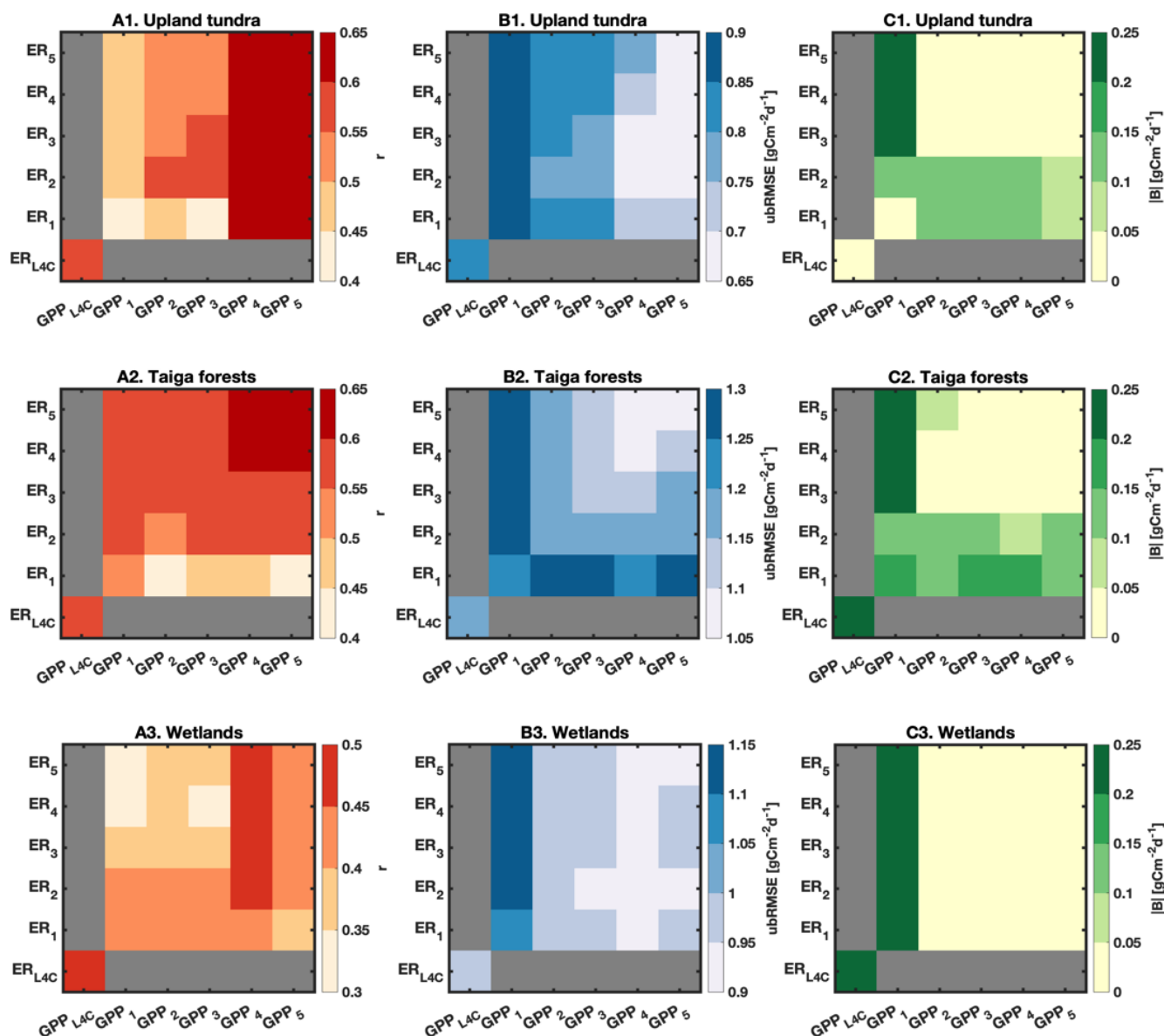
Figure 8. Spatiotemporal performance of modeled net ecosystem \text{CO}_2 exchange (NEE) against daily-averaged eddy covariance NEE ( \text{NEE}_{\text{EC}} ) for upland tundra, taiga forests, and wetlands during the growing season. NEE is computed as the difference between ecosystem respiration (ER) and gross primary production (GPP). \text{GPP}_{\text{L4C}} and \text{ER}_{\text{L4C}} refer to outputs from the original L4C model, while \text{GPP}_1 through \text{GPP}_5 and \text{ER}_1 through \text{ER}_5 correspond to the Arctic–Subarctic (AS) adapted formulations (Sects. 3 and 4.1). The (\text{ER}_i, \text{GPP}_j) grid cell corresponds to the \text{NEE}_{i,j} configuration. The Pearson correlation coefficient is denoted by r (dimensionless), and ubRMSE and |B| denote the unbiased root mean square error and absolute bias, respectively (in \text{gCm}^{-2}\text{d}^{-1} ). Spatiotemporal metrics were derived from 100 random splits (70 % training, 30 % testing), accounting for both spatial and temporal variability. The total number of data points used for training (testing) is 1155 (495) for upland tundra, 3243 (1389) for taiga forests, and 2557 (1096) for wetlands (Sect. 4.3). Reported values correspond to median metrics computed over the testing splits (Tables E1–E5).
