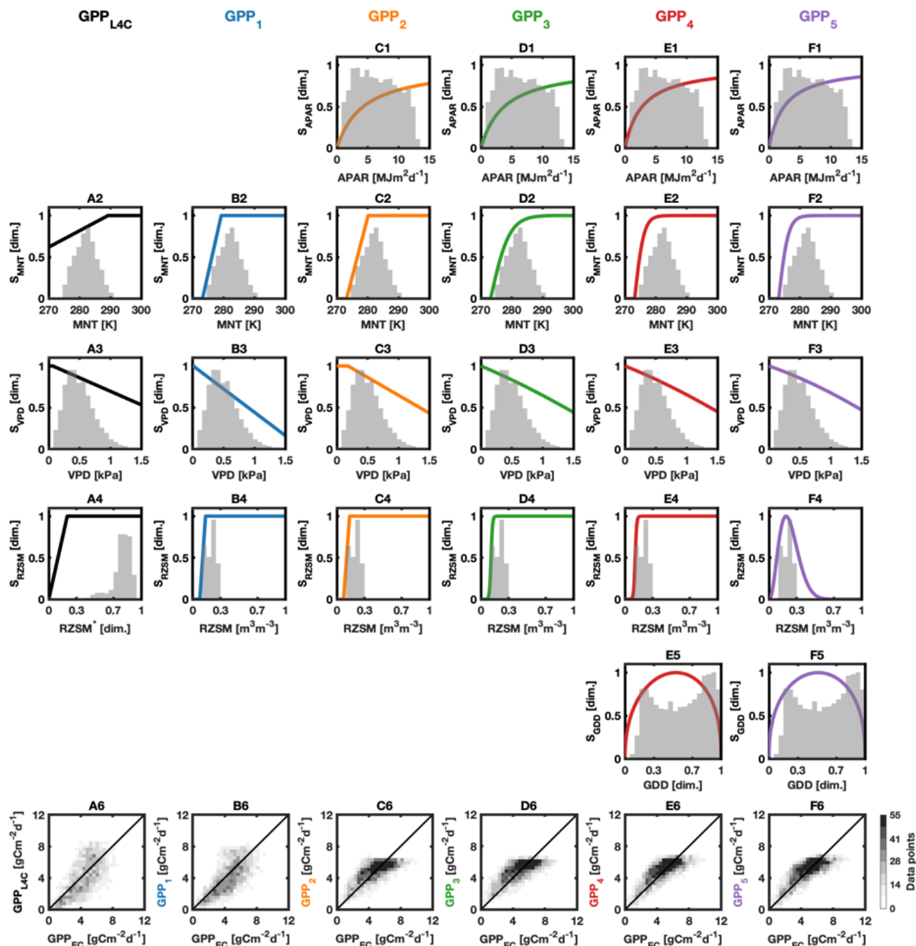
Figure 3. Same as Fig. 2, but for taiga forests . The spatiotemporal comparison includes all available \text{GPP}_{\text{EC}} data points for taiga forests after filtering, including those used for calibration (4632 data points; Sect. 4.3).
