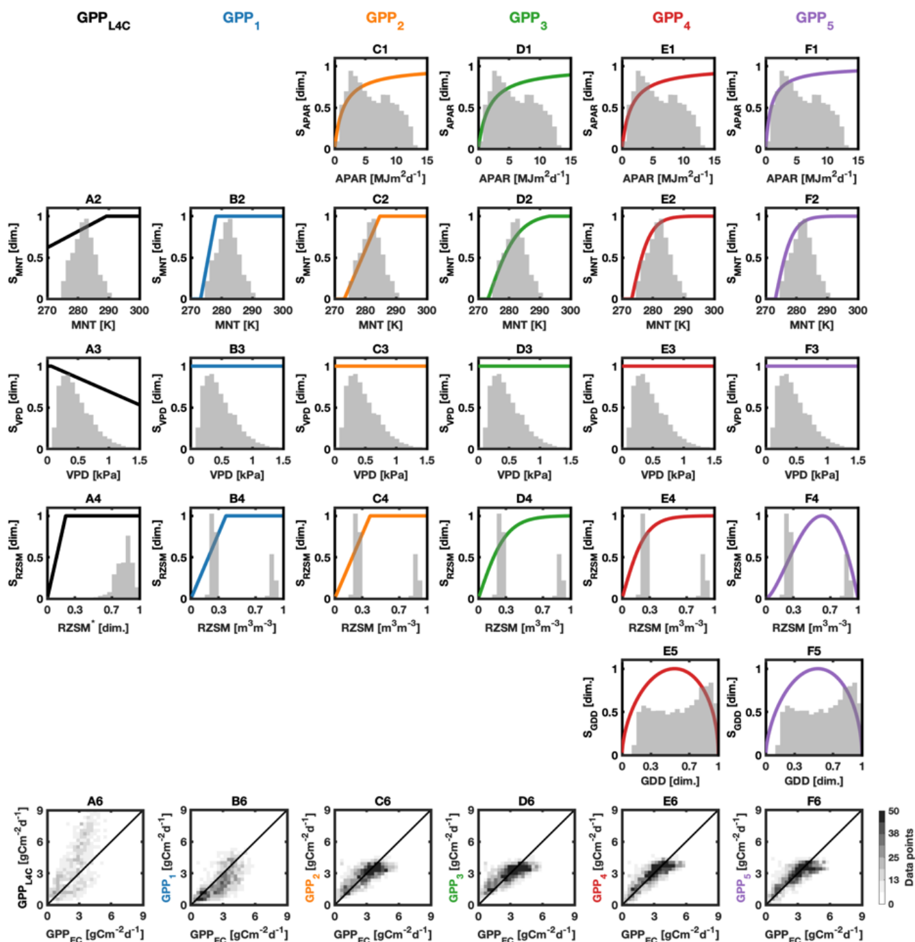
Figure 4. Same as Fig. 2, but for wetlands . The spatiotemporal comparison includes all available \text{GPP}_{\text{EC}} data points for wetlands after filtering, including those used for calibration (3653 data points; Sect. 4.3).
