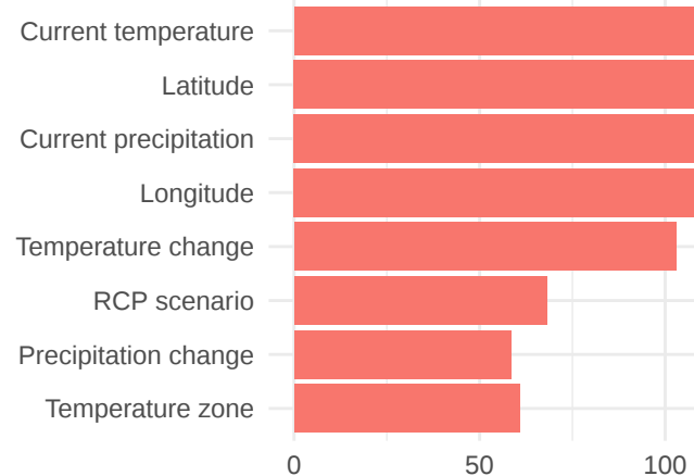
RCP6.0
