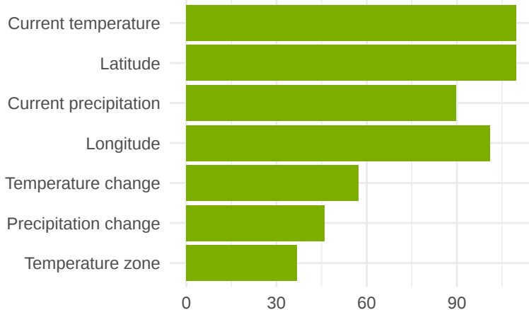
RCP8.5
