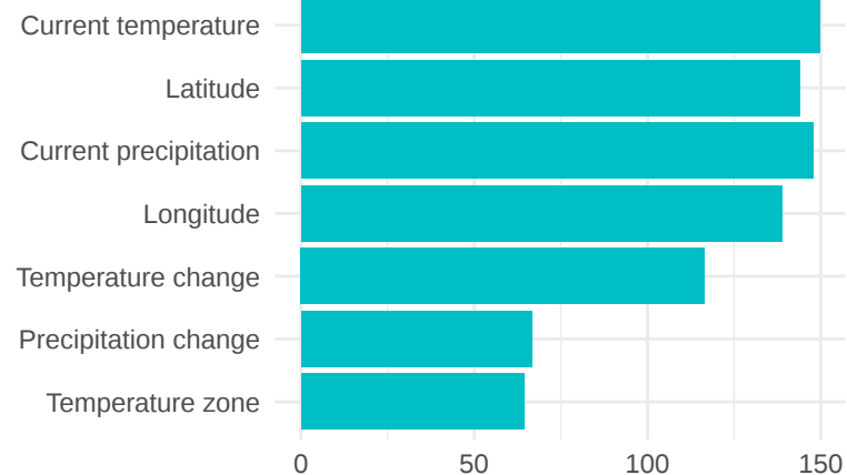
RCP6.0
