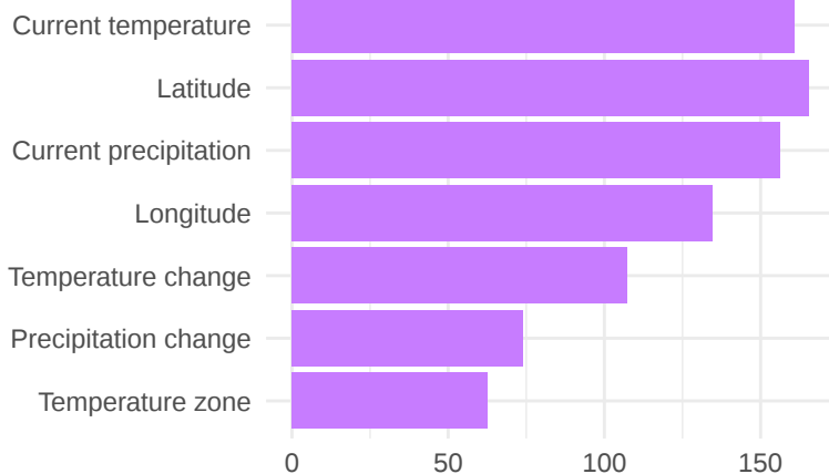
RCP8.5
