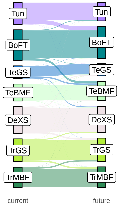
(a) RCP26
