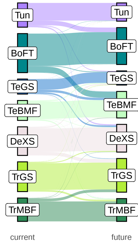
(c) RCP85
