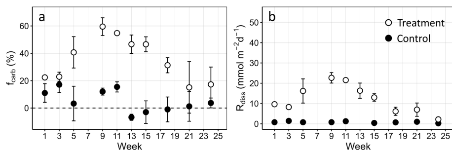
Figure 4. (a) Mean fraction of total DIC derived from \text{CaCO}_3 dissolution ( f_{\text{carb}} ) as determined using the Keeling plot method. Values are expressed as percentages. (b) Corresponding mean \text{CaCO}_3 dissolution rates ( R_{\text{diss}} ). Values of R_{\text{diss}} were only calculated for positive values of f_{\text{carb}} , as discussed in the main text. Error bars are standard deviations based on three replicate chambers.
