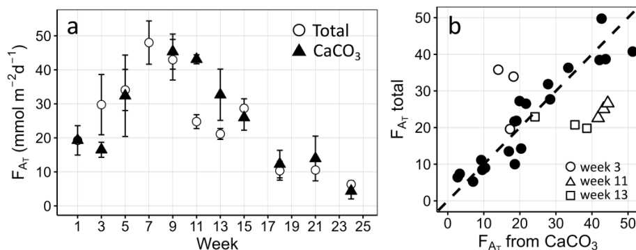
Figure 6. Shell-amended chamber flux comparison of total A_T , which was measured directly in the overlying water, and CaCO_3 A_T , which was derived using the Keeling plot analysis. (a) Mean weekly fluxes with standard deviations based on three replicate chambers. (b) 1 : 1 plot, comparing the individual weekly total and CaCO_3 -derived A_T fluxes per chamber.
