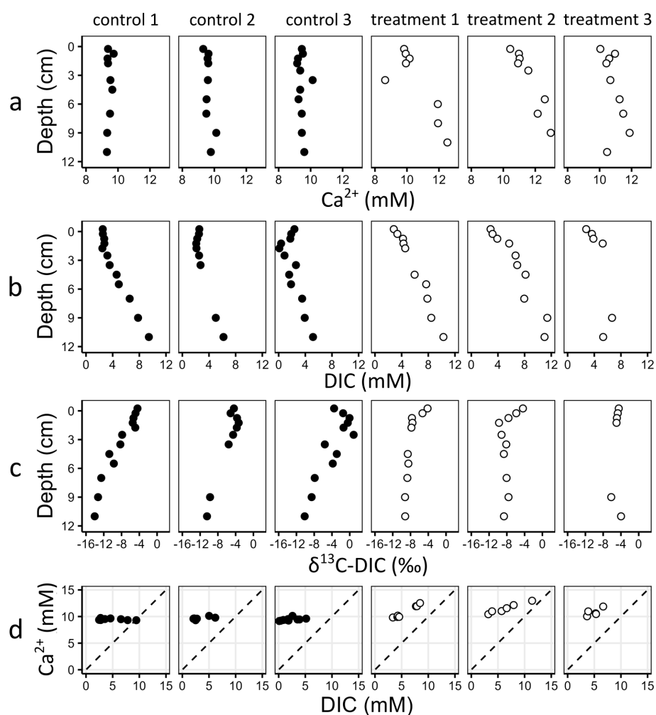
Figure 5. Pore-water profiles. (a) Calcium ( \text{Ca}^{2+} ). (b) Dissolved inorganic carbon (DIC). (c) Isotopic DIC composition ( \delta^{13}\text{C-DIC} ). (d) 1 : 1 plot, comparing \text{Ca}^{2+} and DIC concentrations. Pore-water samples were only taken once at the end of the experiment, explaining the buildup of solutes in deeper anoxic layers, as further discussed in the main text.
