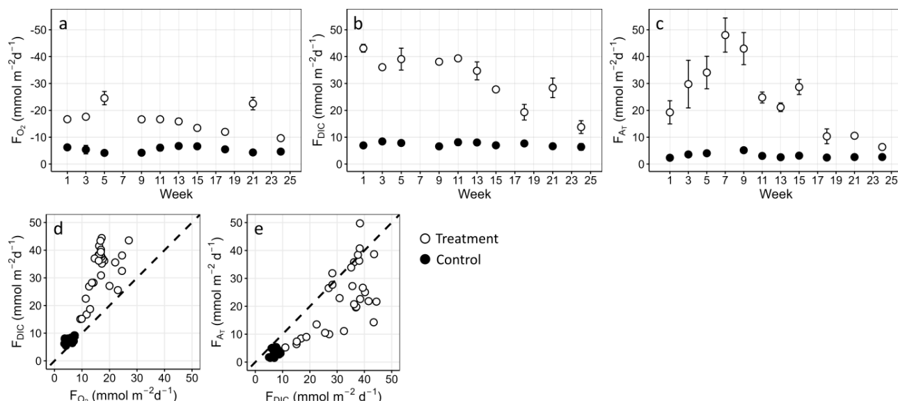
Figure 3. (a) Oxygen fluxes ( F_{\text{O}_2} ). (b) Dissolved inorganic carbon fluxes ( F_{\text{DIC}} ). (c) Alkalinity fluxes ( F_{\text{AT}} ). Positive fluxes indicate fluxes into the overlying water (i.e., net production by the sediment), negative fluxes indicate fluxes into the sediment (i.e., net consumption by the sediment). Means are plotted with error bars representing standard deviations based on three replicate chambers. No \text{O}_2 and DIC data were available for week 7, as only open incubations were performed during that week. (d) 1 : 1 plot, comparing F_{\text{DIC}} and F_{\text{O}_2} . (e) 1 : 1 plot, comparing F_{\text{AT}} and F_{\text{DIC}} .
