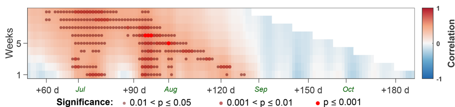
Figure 2. Correlogram showing the relationship between IRise and last-year precipitation averaged over different window sizes (y-axis, in weeks) and starting dates (x-axis, in days relative to SOS). Average calendar dates (across all years) at which each month begins are indicated in green. Correlations were computed on a 1 week \times 1 d grid and lightly smoothed using an anisotropic Gaussian filter ( \sigma_x = 0.8 d, \sigma_y = 1.3 d) for clarity. Statistical significance, computed on the unsmoothed correlations, is represented by markers whose size, opacity and color saturation scale with p -value. Colors indicate correlation sign and magnitude (red = positive; blue = negative). The strongest correlation occurs for a 6 week window, which can be decomposed into two shorter windows of influence: one at 3 weeks (SOS+94 d) and one at 2 weeks (SOS+120 d).
