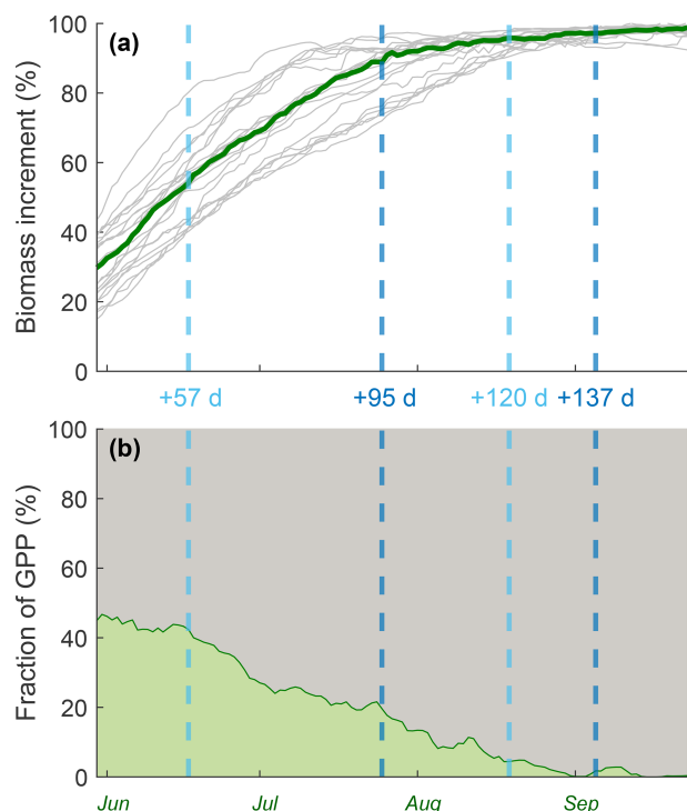
Figure 5. Effect of precipitation on tree physiological responses. Vertical dashed lines indicate the long-term correlation windows for P with I_{Peak} (SOS+57 to SOS+120, light blue) and I_{Rise} (SOS+95 to SOS+137, dark blue). Average calendar dates marking the start of each month (computed across all years) are shown in green. (a) Temporal evolution of median daily biomass accumulation expressed as a proportion of total annual storage. Individual yearly trajectories are shown in grey and the multi-year median is shown in green. (b) Daily fraction of GPP allocated to biomass storage (light green) versus other metabolic or structural processes (dark gray).
