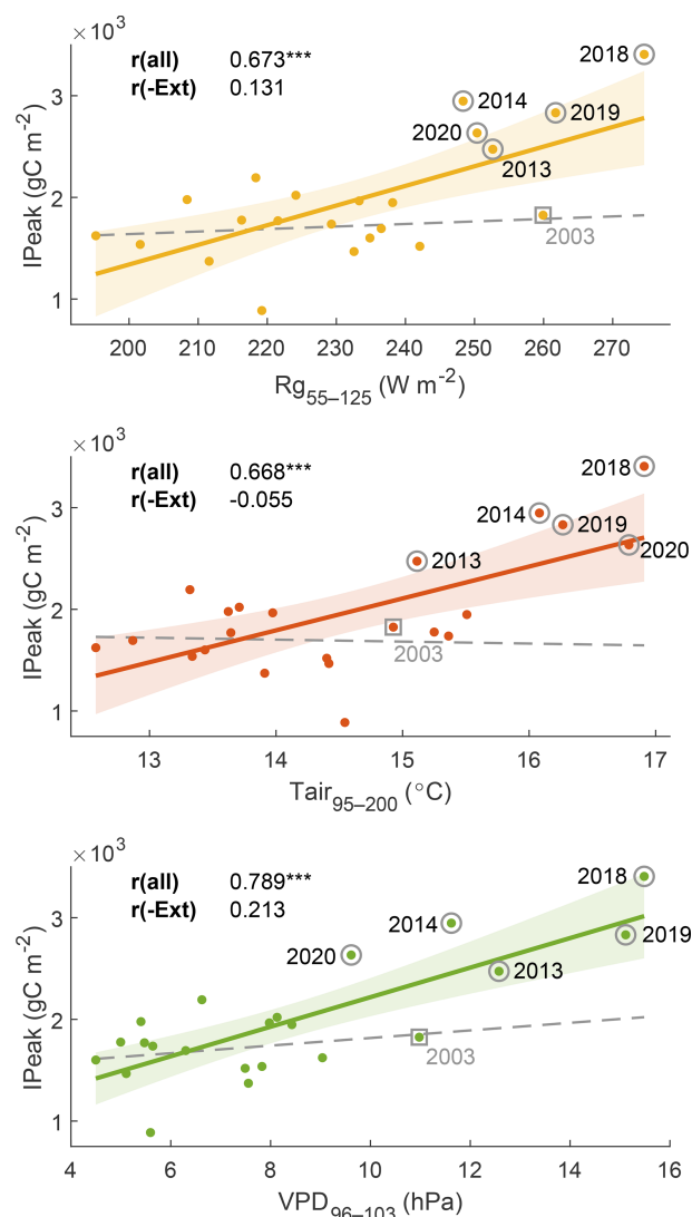
Figure 6. Scatter plots illustrating the strongest correlations between I_{Peak} and mean environmental drivers. Each panel displays the fitted linear regression (solid line) with its 95 % confidence interval (shaded area). The dashed grey line represents the regression excluding extreme-summer years, which are indicated by grey circles. The outlier year 2003 is additionally highlighted with a grey square. Correlation coefficients are reported both for the full time series (all) and for the subset excluding extreme-summer years (-Ext). Statistical significance is indicated by one, two or three stars for p \leq 0.05 , 0.01 and 0.001 , respectively. Approximate threshold values ( 250\ W\ m^{-2} for R_g , 16\ ^{\circ}C for T_{air} , and 10\ hPa for VPD ) mark the conditions above which I_{Peak} responds to environmental drivers. Although I_{Peak} retains the units of GPP, it represents a wavelet-derived metric and should be interpreted comparatively rather than as an absolute flux.
