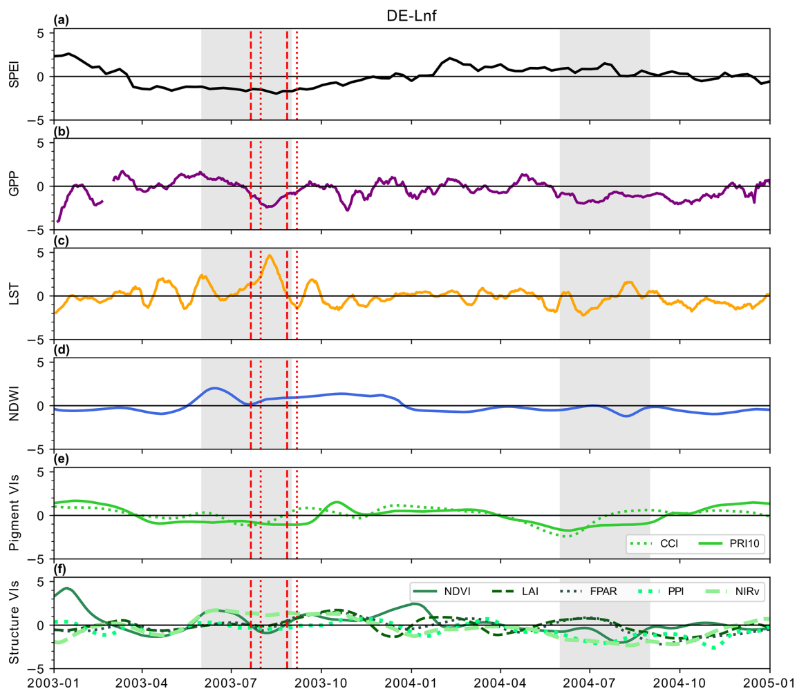
Figure A4. Time series of z -scores during drought and post-drought periods at DE-Lnf. Red vertical dashed lines show GPP Date start and GPP Date end and vertical red dotted lines show drought start and end dates based on SPEI-3. The grey shaded period shows the peak growing season that is used for the post-drought analysis.
