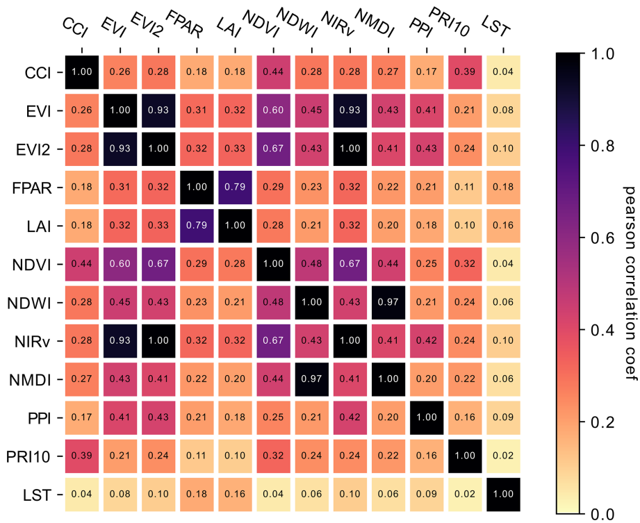
Figure A1. Average within site correlation between each combination of VI z-score time series.
