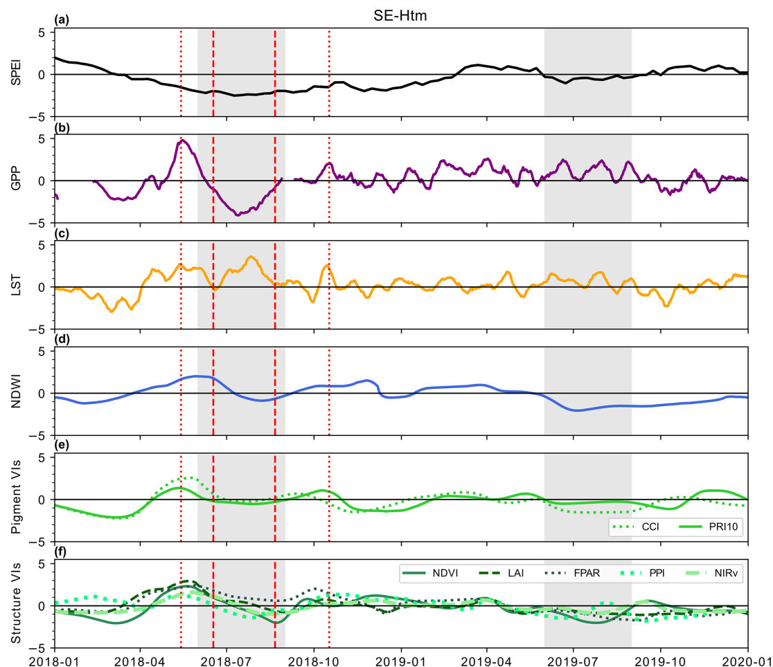
Figure A5. Time series of z -scores during drought and post-drought periods at SE-Htm. Red vertical dashed lines show GPP Date start and GPP Date end and vertical red dotted lines show drought start and end dates based on SPEI-3. The grey shaded period shows the peak growing season that is used for the post-drought analysis. The grey horizontal line marks -1 i.e. the threshold we used to define drought response.
