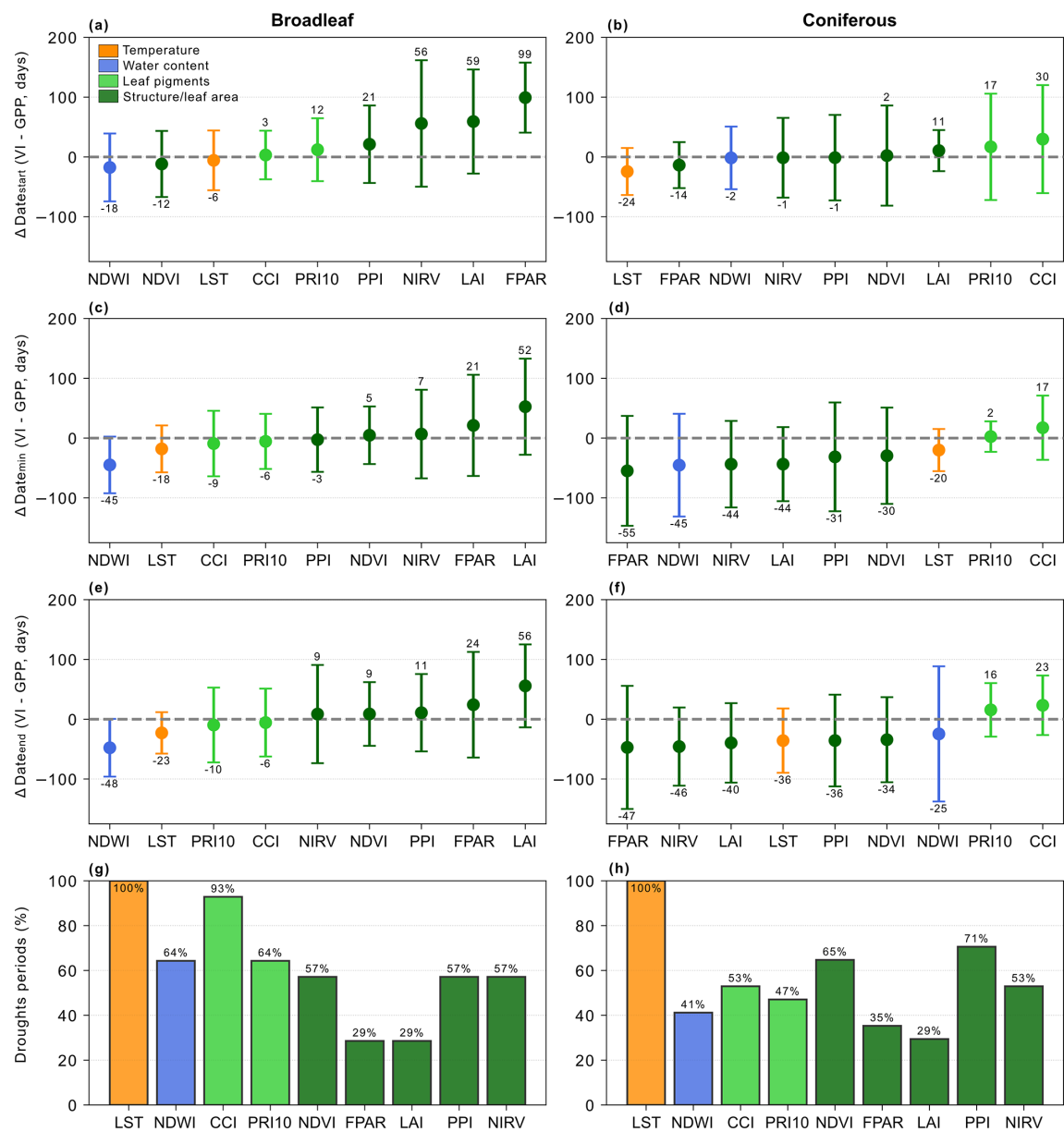
Figure 3. Mean ± standard deviation of difference between (a, b) Date start , (c, d) Date min and (e, f) Date end of VIs and GPP at broadleaf (left) and coniferous (right) sites. Negative number means the VI date preceded the GPP date. Numbers above or below the error bars are the mean difference in days. (g, h) show the percentage of droughts where Date start was found for each VI (i.e. VI responded to that drought). Bar colour refers to the VI category (orange = land surface temperature, blue = vegetation water content, light green = leaf pigments, dark green = canopy structure/leaf area). Note that VI order changes in each plot.
