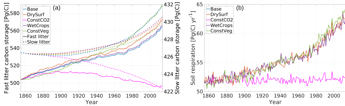
Figure S6. (a) Global dead carbon available for decomposition spitted into fast decomposable (solid) and slowly decomposable (dashed) components. (b) Decomposition rate of this carbon.
