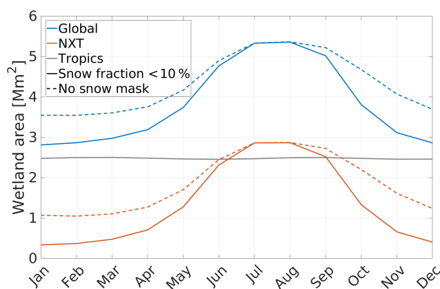
Figure 2. Wetland area annual cycle for the “Base” experiment. Solid lines only include cells with less than 10 % snow whereas dashed lines includes all cells. Blue lines are global values, reddish include only the NXT area (north of 30° N) and the gray line is the “tropics” (everything south of 30° N). For the tropical area, snow masking does not make any difference.
