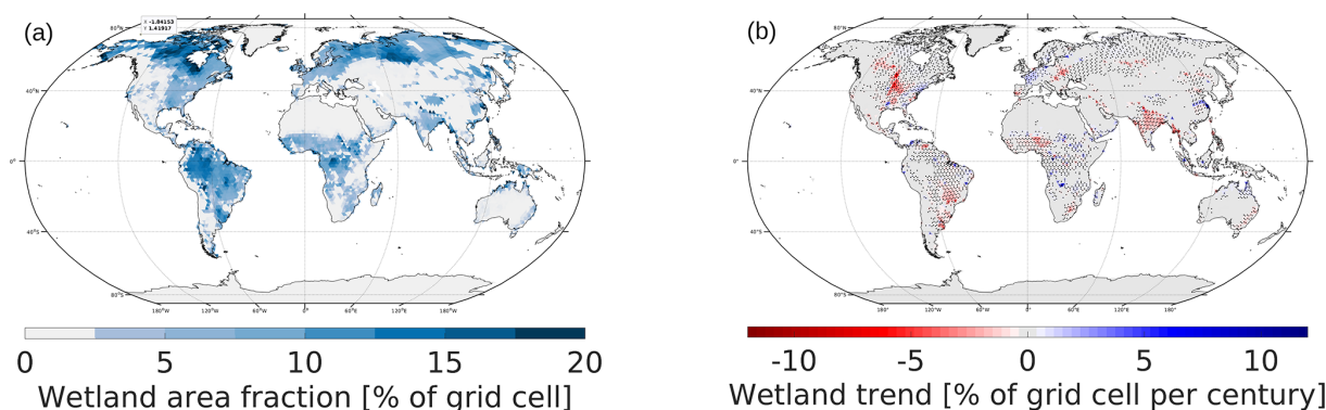
Figure 1. “Base” average distribution of (a) wetland area (% of grid cell area) in Northern Hemisphere summer (JJA) and (b) 1855–2014 wetland area trend of annual means (% of grid cell per century). Black dots mark cells with trends significant at the 95 % level according to Matlab’s fitlm function.
