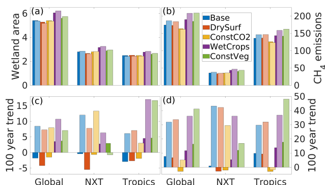
Figure 4. Top panels: NH summer (JJA) Wetland area (in \text{Mm}^2 ) for areas with \leq 10\% snow (a) and annual wetland methane emissions (b, [\text{Tg}(\text{CH}_4) \text{ yr}^{-1}] ). Bottom panels: 100 year trend (1855–2014 average) of (c) annual wetland area and (d) annual wetland methane emissions. Dark (colors exactly matching the legend) partly covered bars represent the entire experiment period (1855–2014), while brighter overlaid bars represent the 1980–2014 period. Colors indicate the different experiments.
