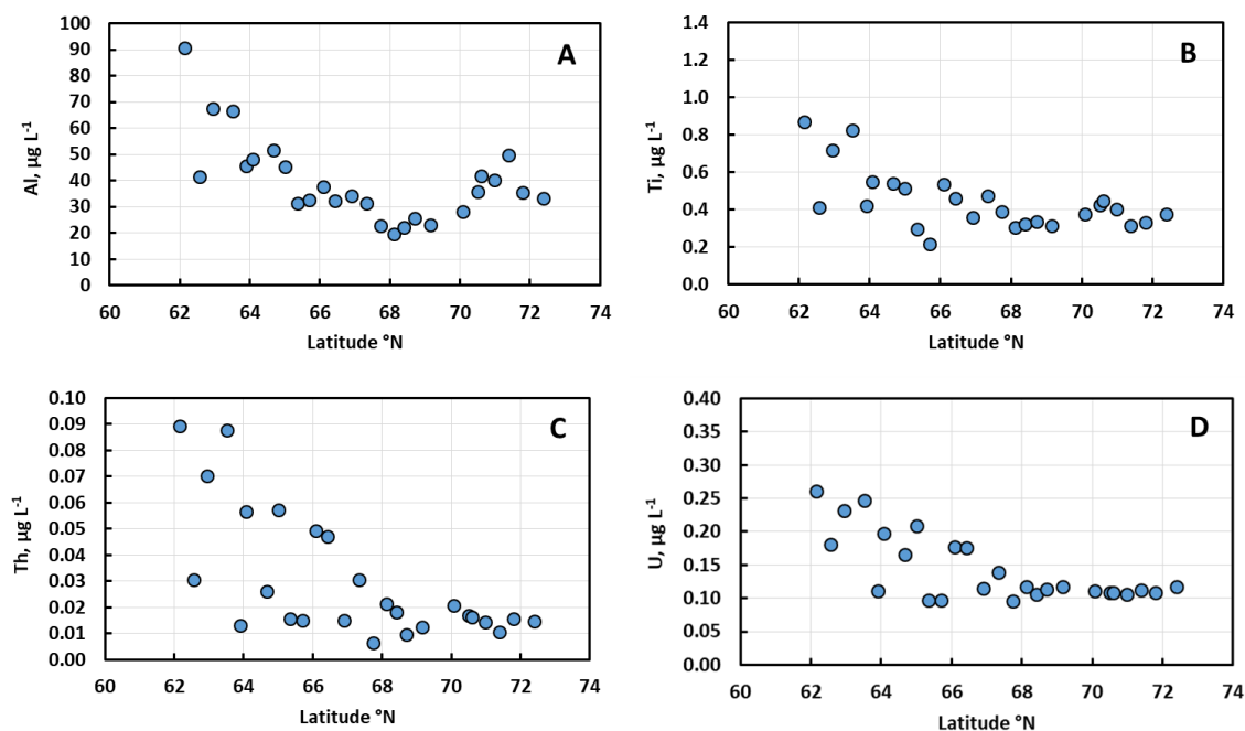
Figure 4. Examples of low-solubility, predominantly colloidal elements whose concentration in the Lena River main stem decreased northward, from Yakutsk to Kyusyur: (A), Al; (B), Ti; (C), Th and (D), U.
