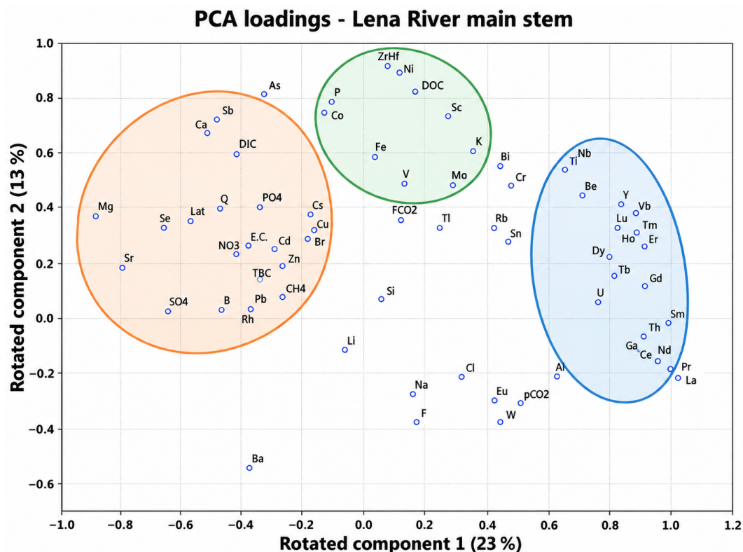
Figure 7. Varimax-rotated PCA loading plot for standardized hydrochemical variables measured in the Lena River main stem ( n = 26 ). Rotated components 1 and 2 explain 23 % and 13 % of total variance, respectively (36 % cumulative). Colored envelopes are visual guides to broad geochemical associations inferred from the loadings and independent geochemical evidence: orange, mobile weathering- and groundwater-related solutes; green, DOC, nutrients, and mixed surface-derived variables; blue, low-solubility lithogenic and colloid-associated elements. Overlap among envelopes and variables outside them emphasize that the ordination is exploratory and does not represent statistically discrete clusters.
