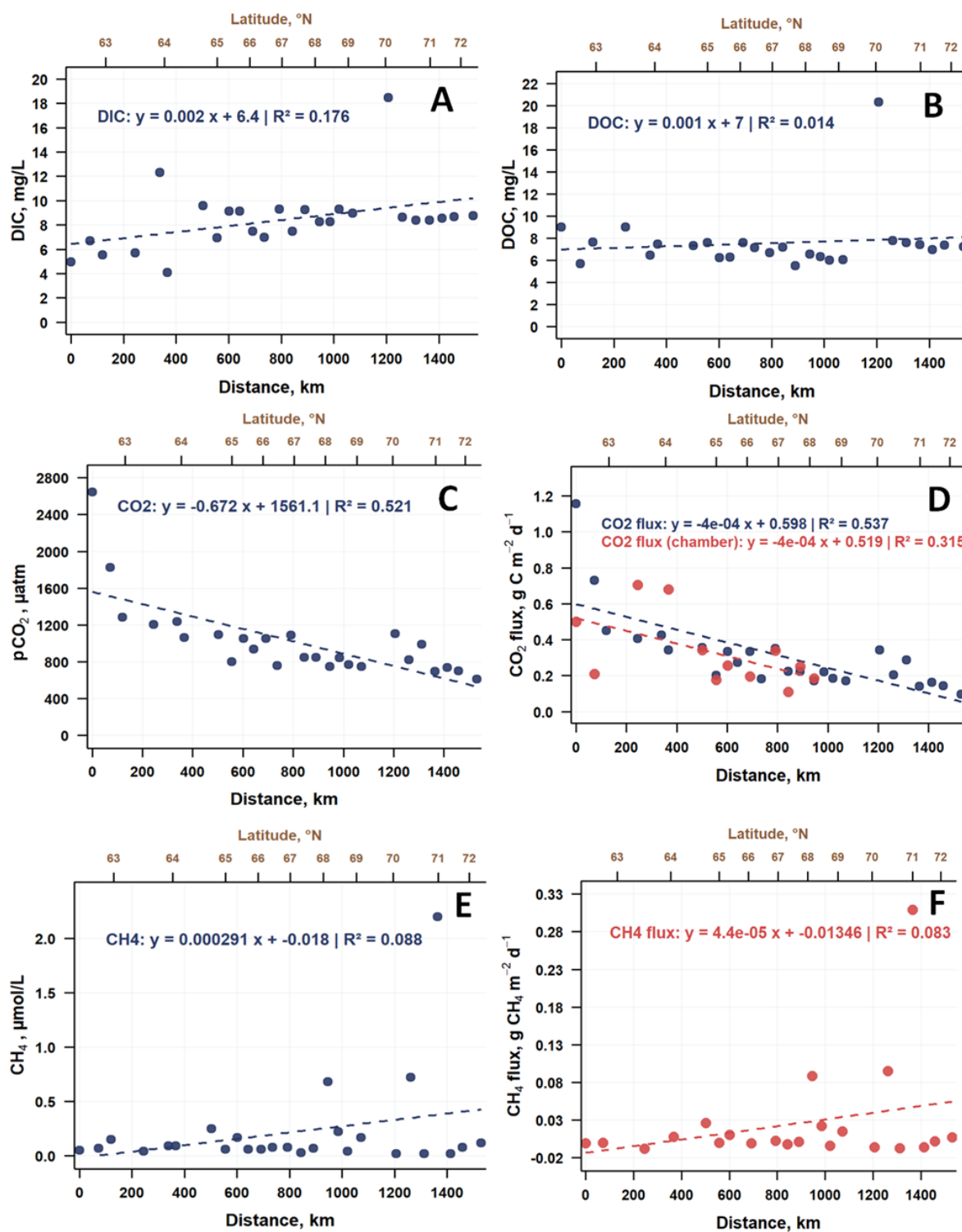
Figure 2. Spatial variations of DIC (A), DOC (B), p\text{CO}_2 (C), F_{\text{CO}_2} (D), \text{CH}_4 concentration (E) and F_{\text{CH}_4} (F) in the main stem of the Lower Lena River, from Yakutsk to Kyusur. The dots represent discrete sampling points and dashed lines are linear regressions with equation parameters given on each panel.
