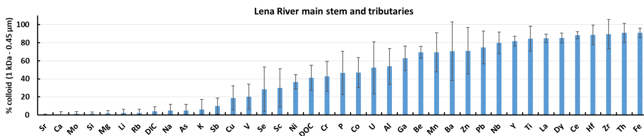
Figure 8. Average ( \pm SD, n = 12 ) proportion of colloidal forms of major and trace elements in the Lena River and tributaries measured by dialysis procedure.
