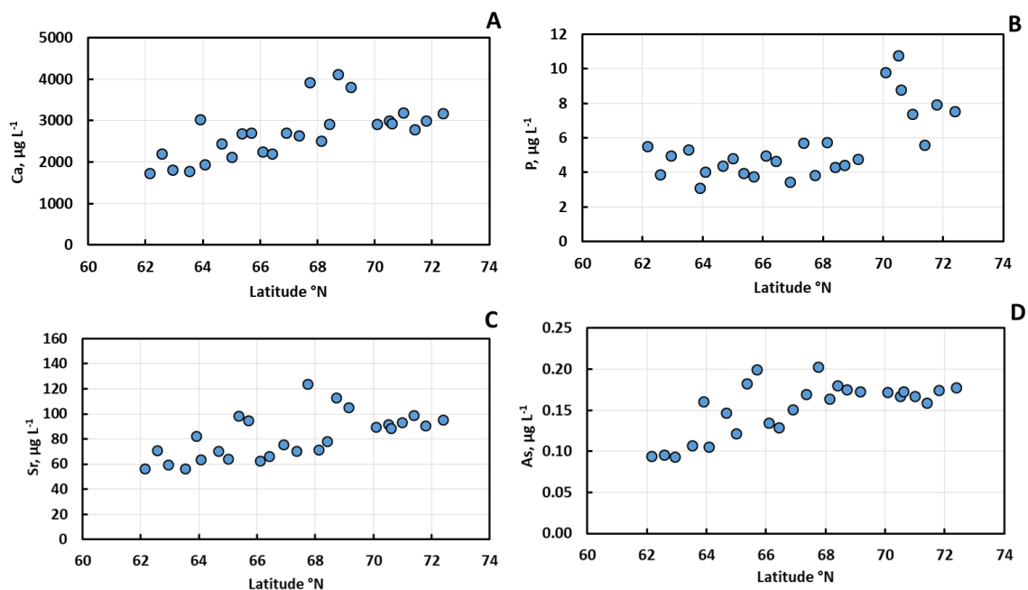
Figure 5. Examples of labile elements with low colloidal proportions whose concentrations increased northward, from Yakutsk to Kyusyur: (A), Ca; (B), P; (C), Sr and (D), As.
