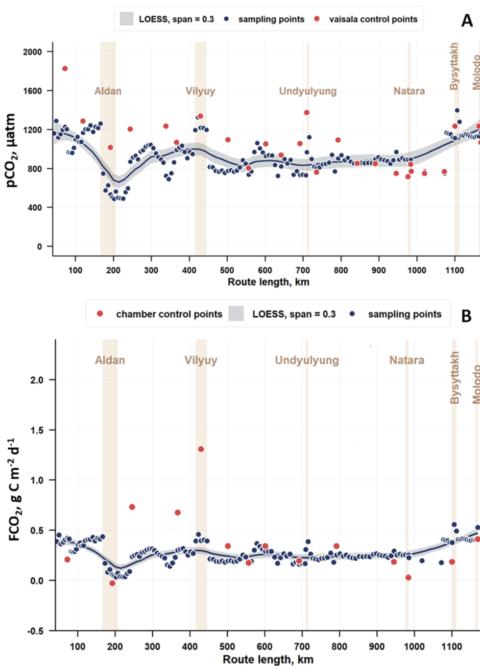
Figure 3. Spatial variation of p\text{CO}_2 (A) and diffusive CO 2 flux ( F_{\text{CO}_2} ) (B) along the Lower Lena River main stem during the south–north transect. Blue symbols show underway values obtained from the Kingston water intake, whereas red symbols show independent stationary checks obtained with a second Vaisala p\text{CO}_2 system. The two measurements were not strictly synchronous or spatially co-located; the red symbols therefore provide external field validation rather than exact replicate observations. Shaded vertical bands indicate the locations of major tributaries (Aldan, Vilyui, Undyulyung, Natara, Bysyttakh, Molodo). Solid lines represent LOESS (locally estimated scatterplot smoothing) fits: span = 0.3 for continuous measurements and span = 0.8 for control datasets due to their lower number of observations ( n = 24 ).
