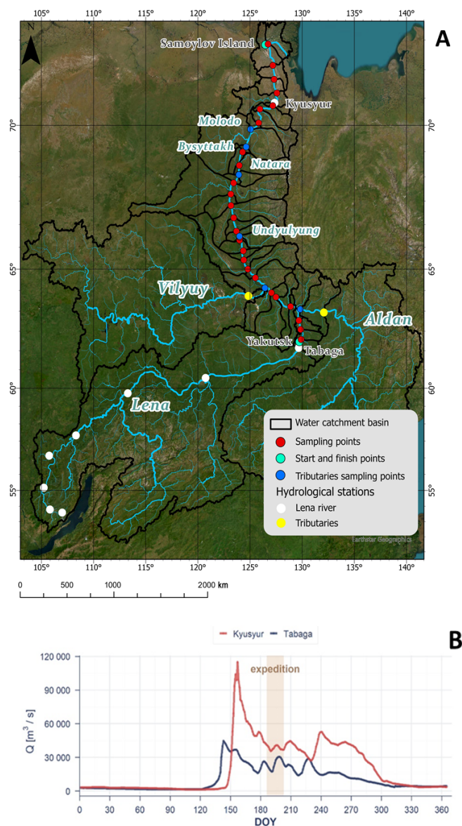
Figure 1. (A) The Lena River watershed and the position of sampling points of this study and (B) Hydrograph of the Lena River at Kyusyur (red line) and Tabaga (blue line) in 2022 for the period of expedition (highlighted in pink).
