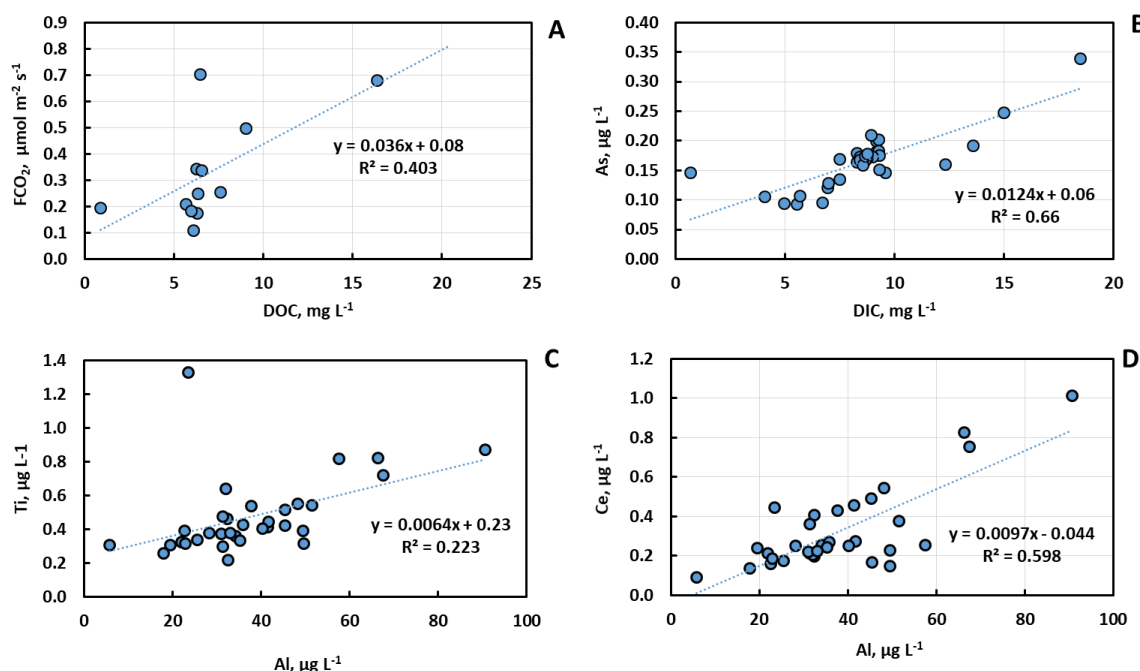
Figure 6. Linear relationships in the Lena River main stem between concentrations of DOC and chamber-measured F_{CO_2} (A), DIC and As (B) and dissolved Al with Ti (C) and Ce (D).
