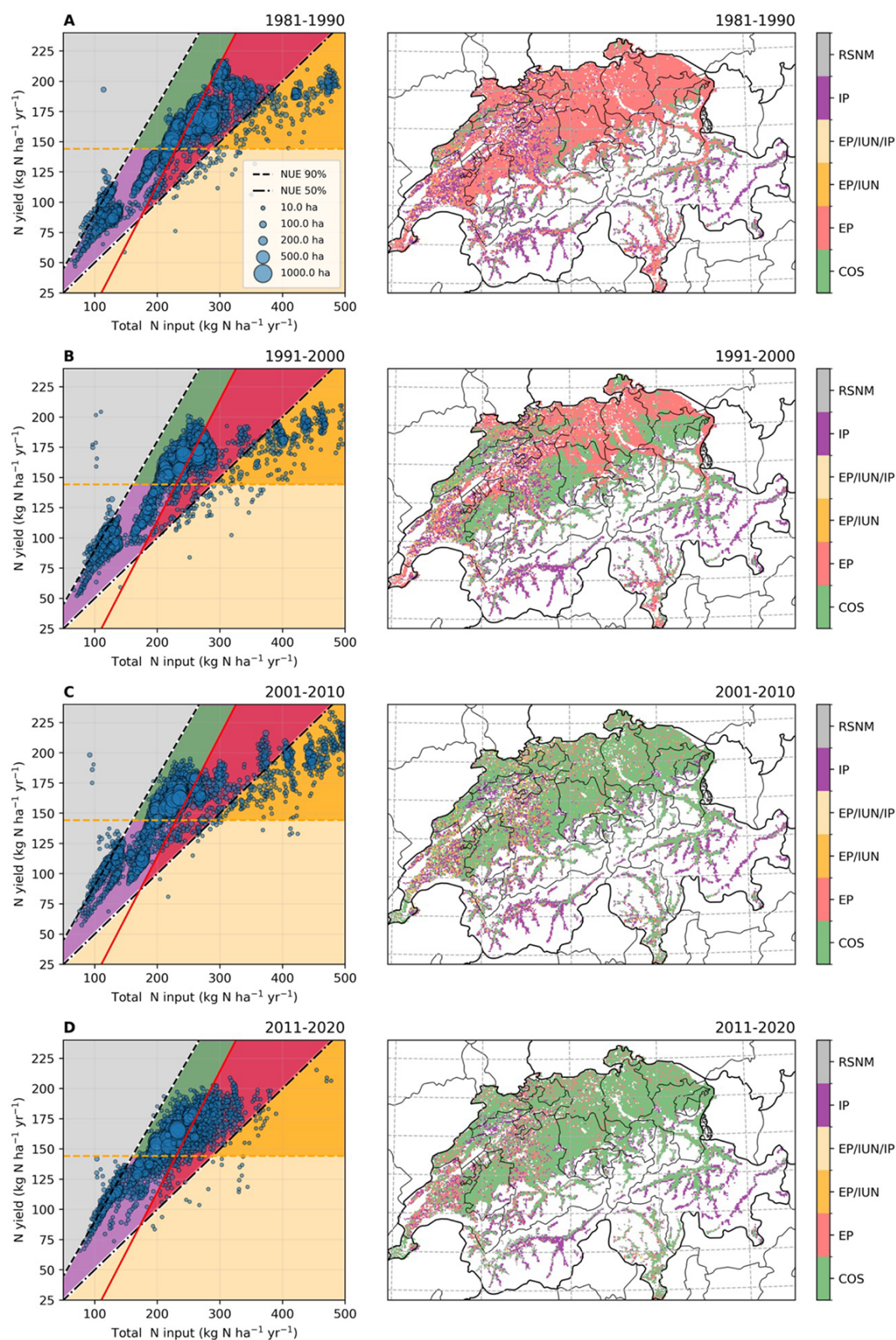
Figure 4. The EUNEP Framework of the NUE indicator diagram of Swiss grasslands and decadal geographical distributions of six categorised agricultural land. (A) 1981–1990, (B) 1991–2000, (C) 2001–2010, (D) 2011–2020. Grasslands refer to managed meadows only, while managed pastures and summer pastures for grazing are not included.
