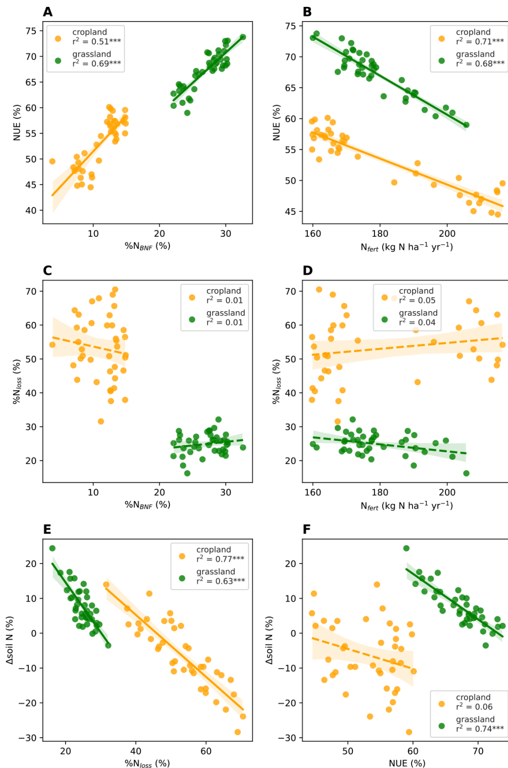
Figure 8. Analysis of N inputs, N loss and soil N balance of Swiss agroecosystems. Response of NUE to (A) relative BNF ( \%N_{BNF} ) and (B) fertilizer N inputs ( N_{fert} ). No significant relationships between (C) relative BNF (D) fertilizer N inputs and relative N loss ( \%N_{loss} ). Relationships between (E) relative N loss, (F) NUE and soil N balance ( \Delta\text{soil N} ). BNF, N loss and soil N balance are expressed as percentage relative to total N input. The points represent annual mean values. Croplands are shown in yellow colour, and grasslands are shown in green colour. Solid lines show significant relationships with significance level *** P < 0.001 , and dashed lines indicate insignificant relationships.
