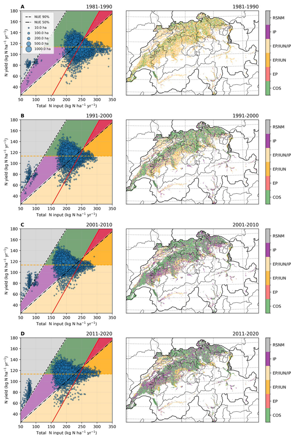
Figure 3. The EUNEP Framework of the NUE indicator diagram of Swiss croplands and decadal geographical distributions of six categorised agricultural land. (A) 1981–1990, (B) 1991–2000, (C) 2001–2010, (D) 2011–2020. For the NUE diagram, the dashed black lines are 90 % NUE, and dotted black lines are 50 % NUE. The solid red lines and dashed orange lines represent desired maximum N surplus and desired minimum N yield, which are the mean values of simulated N surplus and N yield for each agroecosystem in the 1980s, which set goals for improvement in the following decades. Six regimes are (note the colour scheme is different from the originally proposed diagram; EU Nitrogen Expert Panel, 2016): characteristic operating space (COS – shaded green area), excessive pollution (EP – shaded red area), insufficient productivity (IP – shaded purple area), EP and inefficient use of nitrogen (EP/IUN – shaded orange area), EP/IUN/IP (shaded light yellow area), risk of soil nitrogen mining (RSNM – shaded grey area). The dark blue and light blue circles represent data from 1981–1990 and 2011–2020, respectively. The size of the circle is proportional to the summed area of croplands or grasslands that is aggregated by N yield and total N input (precision at 0.1 \text{ kg N ha}^{-1} ), with legends shown in the figure.
