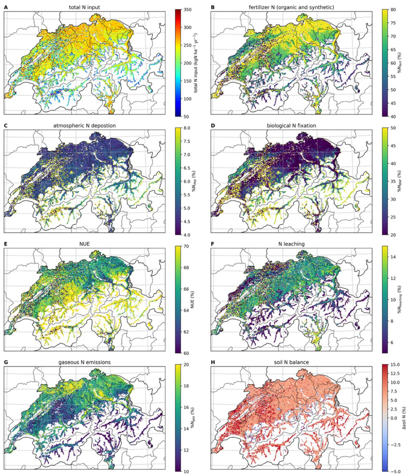
Figure 6. Spatial maps of N budgets and soil N balance of Swiss grasslands over 1981–2020. (A) total N input, (B) fertilizer N including manure and synthetic fertilizers, (C) atmospheric N deposition, (D) BNF, (E) NUE, (F) N leaching, (G) gaseous emissions, (H) soil N balance. Total N inputs have the unit \text{kgN ha}^{-1} \text{yr}^{-1} , and other variables are expressed as percentage relative to total N inputs (note the difference in scales). See Fig. S7 in the Supplement for maps shown absolute values.
