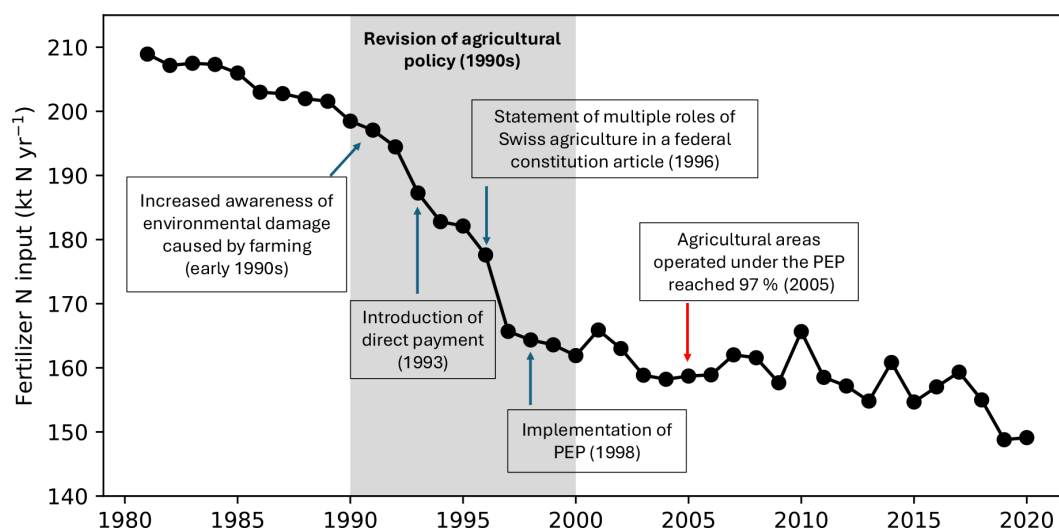
Figure 1. Nitrogen inputs from fertilizers to agricultural land in Switzerland. Fertilizers include livestock manure and synthetic fertilizers. Values from compiled datasets (see Methods). Shaded grey area represents the period in the 1990s when national policies and measures were implemented in the agricultural sector. Important events are shown along the timeseries of fertilizer N inputs. Values in the parenthesis are corresponding years. Note that the y-axis starts from 140 kt N yr -1 . PEP is Proof of Ecological Performance.
