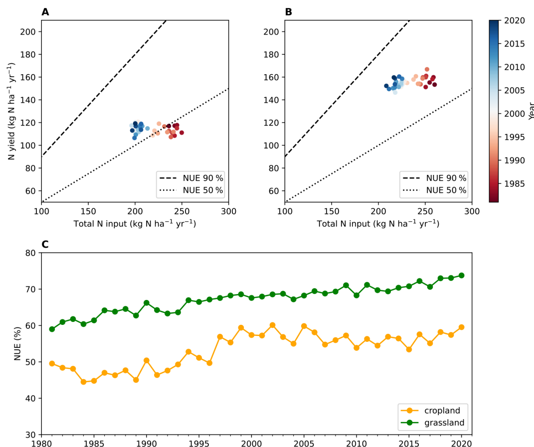
Figure 2. Modelled annual mean total N input, N yield and NUE of Swiss croplands and grasslands from 1981 to 2020. Total N input and N yield of croplands (A) and grasslands (B). In panels (A) and (B), the dashed black lines and dotted black lines represent 90 % and 50 % NUE, respectively and the red-blue scale shows the year. Note the axes do not start from zero. (C) NUE of croplands (yellow) and grasslands (green). Note the y-axis starts from 30 %.
