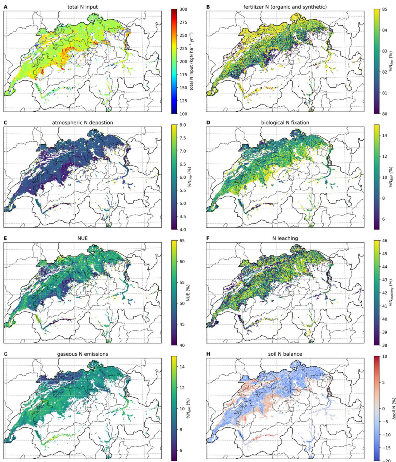
Figure 5. Spatial maps of N budgets and soil N balance of Swiss croplands over 1981–2020. (A) total N input, (B) fertilizer N including manure and synthetic fertilizers, (C) atmospheric N deposition, (D) BNF, (E) NUE, (F) N leaching, (G) gaseous emissions, (H) soil N balance. Total N inputs have the unit \text{kg N ha}^{-1} \text{ yr}^{-1} , and other variables are expressed as percentage relative to total N inputs (note the difference in scales). See Fig. S6 in the Supplement for maps showing absolute values.
