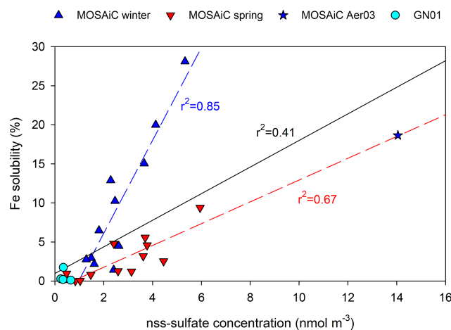
Figure 6. Relationship between aerosol Fe solubility and \text{nss-sulfate} concentration. Fe solubility is plotted against \text{nss-sulfate} concentration for GN01 (cyan circles), MOSAiC Winter (blue triangles), and MOSAiC Spring (red inverted triangles). Dashed regression lines are included where statistically significant correlations exist for seasonal data (Aer03 excluded from MOSAiC winter data due to unusually high \text{nss-sulfate} ). Solid black regression line indicates significant correlation for all data.
