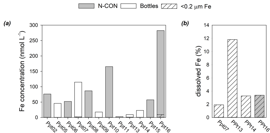
Figure 3. Iron concentration and solubility in GN01 precipitation samples. (a) Total dissolvable and dissolved Fe concentrations in precipitation samples collected by N-CON sampler and cut-off bottles, with dissolved Fe contributions to four samples indicated by hatching. (b) Percent of total dissolvable Fe in the dissolved fraction at the time of sample recovery for four samples where a subsample was filtered.
