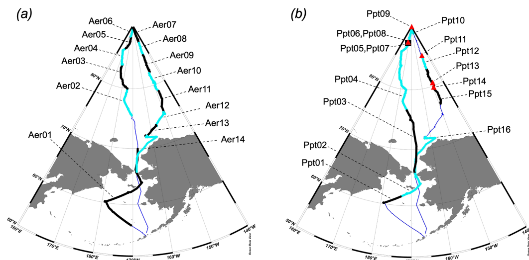
Figure 1. Locations of (a) bulk aerosol and (b) precipitation samples collected during GN01. Cruise track is shown by thin blue line with aerosol or N-CON precipitation sample collections overlain in black and cyan on each map. Red triangles in (b) indicate locations of blowing snow samples collected with cutoff bottles, while the black square indicates two N-CON samples (Ppt06, Ppt08) collected close to each other and to cutoff bottle samples Ppt05 and Ppt07. The figure was created using Ocean Data View (ODV), version 5.7.2, developed by Schlitzer (2025).
