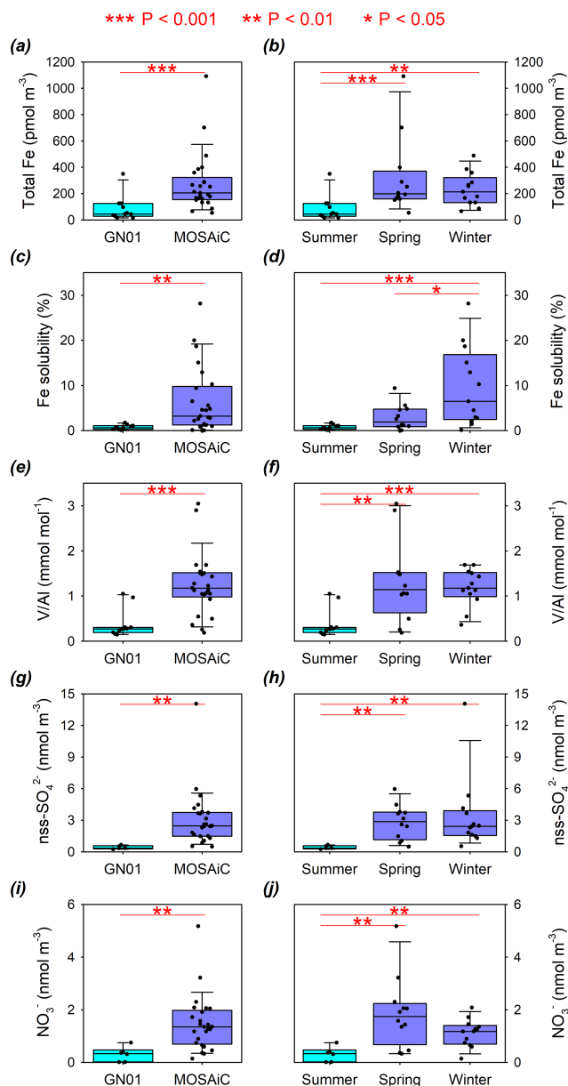
Figure 5. Comparison of aerosol characteristics between GN01 (cyan) and MOSAiC (purple). (a, b) Total aerosol Fe concentration, (c, d) Fe UPW-solubility, (e, f) V/Al molar ratio, (g, h) \text{nss-SO}_4^{2-} concentration, and (i, j) nitrate concentration. Comparisons are made between the two projects (left column) and between seasonal datasets (right column), with MOSAiC data ( n = 26 ) split between winter (deployments 1–13, n = 13 ) and spring (deployments 14–26, n = 13 ). GN01 data excludes samples collected south of 70^\circ \text{S} (Aer01, Aer14; n = 11 , or less where some measurements are below detection). Each box spans 25th to 75th percentiles of data and is bisected by the median, with whiskers extending to 10th and 90th percentiles. Individual datapoints are superimposed as black dots. Red lines indicate statistically significant differences between datasets (Mann-Whitney Rank Sum Test), with level of significance indicated by asterisks.
