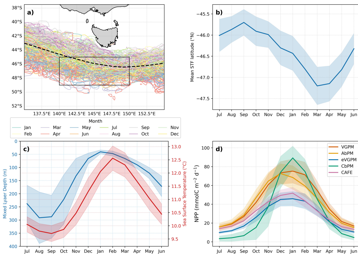
Figure 1. Regional bounding box (solid black line) in which observational and modelled climatological averages were calculated. Mean monthly contours of the subtropical front (STF; 11^{\circ} isotherm at 100 m depth, definition per Orsi et al. 1995) for the period 1998–2022 are given by coloured lines, with the mean given by the dashed black line. (b) Climatological STF extent (1998–2022) as the mean latitude ( ^{\circ} N) ( \pm 1\sigma from the mean) of the 11^{\circ} isotherm at 100 m depth (Orsi et al., 1995). (c) Climatological (1998–2022) means of MLD (blue) derived from Hadley EN4.2.2. profiles and SST (red) from ARMOR-3D, shading is \pm 1\sigma from the mean in the SOTS region box (a). (d) Climatological mean NPP estimates from OC-CCI based satellite algorithms (1998–2022), shading is \pm 1\sigma from the temporal mean.
