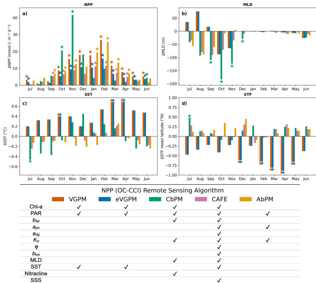
Figure 2. (a) Change in integrated NPP ( \Delta NPP) from five OC-CCI-based remote sensing algorithms calculated from the difference in climatological means of the five highest and five lowest NPP seasons for observations in the region 140–150°E, 45–49°S, for the period 1998–2022. Corresponding changes in the physical drivers for corresponding algorithm high and low NPP year groups are shown for (b) \Delta MLD, (c) \Delta SST and (d) \Delta STF mean latitude. Positive values of \Delta MLD, \Delta SST and \Delta STF indicate deeper MLDs, warmer SSTs and further north mean STF latitude during high NPP seasons respectively. Stars indicate that mean monthly climatological difference in the selected high and low NPP season groups is significant relative to the full time series climatological variability at the p < 0.05 level (10 000 iteration random year bootstrapping analysis). The figure legend describes the specific observational and spectral variables used in each NPP algorithm (Chlorophyll a (Chl- a ), photosynthetically active radiation (PAR), backscatter at 443 nm ( b_{bp} ), phytoplankton absorption at 443 nm ( a_{ph} ), detrital absorption at 443 nm ( a_{dg} ), diffuse attenuation coefficient at 490 nm ( K_d ), the spectral slope of backscatter ( \eta ), the backscatter of pure water ( b_{bw} ), Hadley EN4.2.2 mixed-layer depth (MLD), sea surface temperature (SST), nitracline depth, and sea surface salinity (SSS)).
