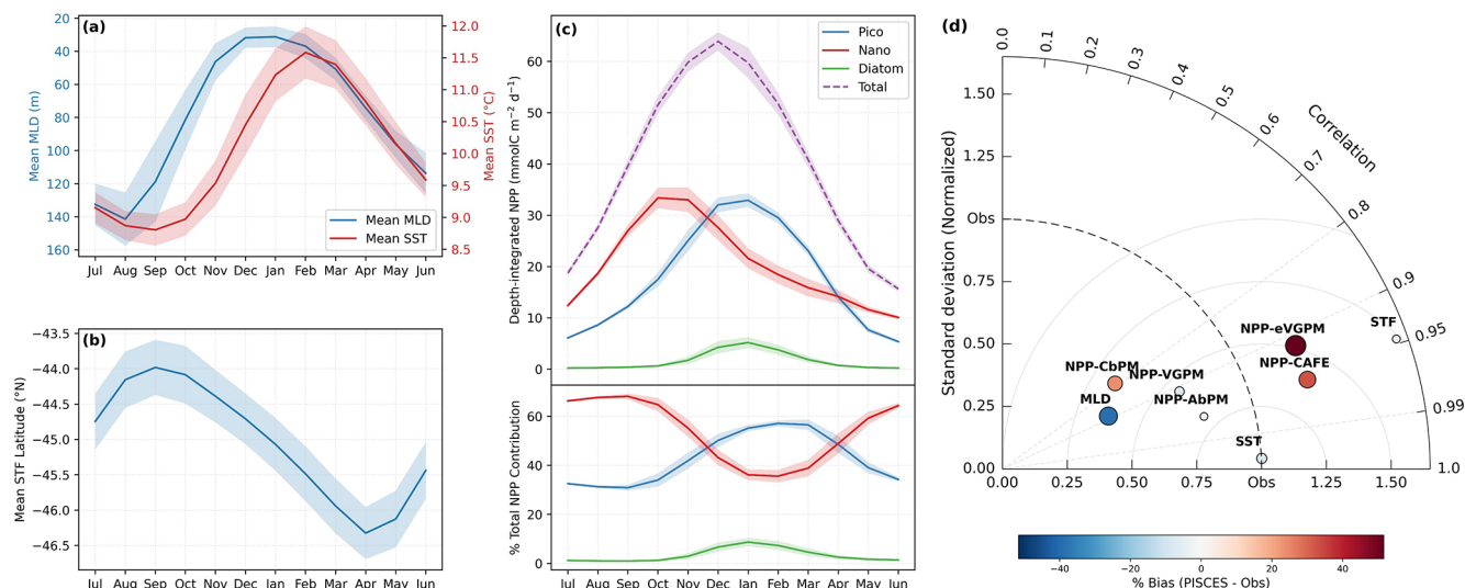
Figure 3. (a) Mean climatological MLD (blue) and SST (red), (b) STF mean latitude in the longitude range 140–150° E extent, and (c) phytoplankton class and total resolved depth-integrated NPP, including percentage contribution of each class to the total NPP inventory, and (d) Taylor diagram summarising climatological differences between NPP, MLD, SST and STF latitude between PISCES-Quota-Fe and observations for the period 1998–2023. Relative bias (%) is given as marker size and colour denoting bias direction.
