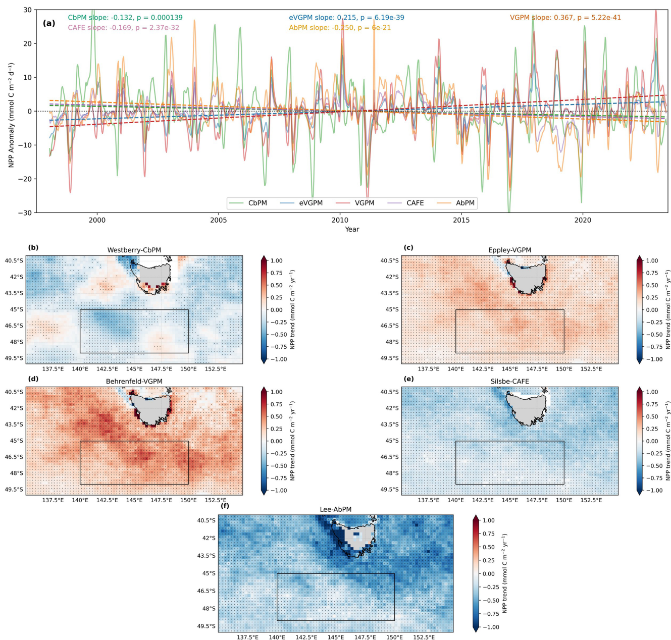
Figure 9. (a) Timeseries (1998–2022) of monthly NPP anomalies from the five remote sensing NPP algorithms, spatially averaged over the SOTS region (45–49° S, 140–150° E). Trends were determined from ordinary least squares regression of the monthly anomalies, with trend slope and p -values for significance given. (b–e) Spatial trends computed from ordinary least squares regressions on monthly single pixel NPP anomalies for each remote sensing NPP algorithm in (a). Stippling in pixels indicates significant trends at the p < 0.05 level. The black box denotes study region used for averaging in (a).
