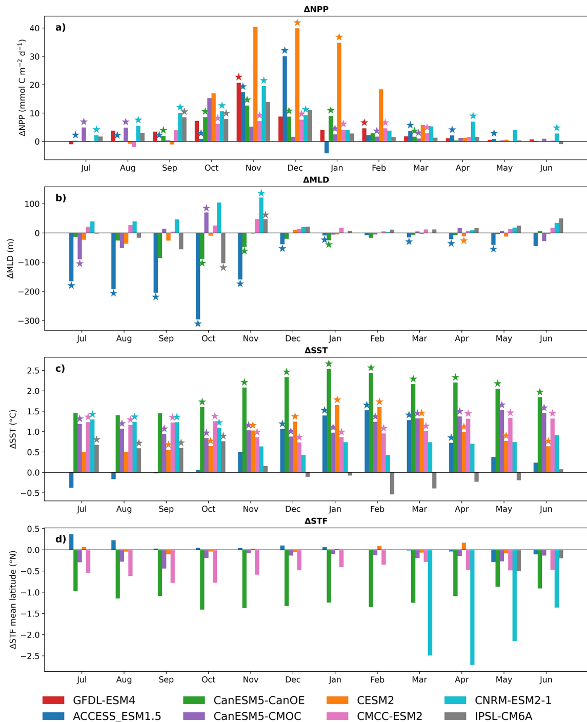
Figure 8. (a) Bootstrap analysis of the change in mean climatological NPP between the 5 highest and 5 lowest seasons of NPP for 8 CMIP6 models listed in Table 2 (note SST and MLD not available for GFDL-EMS4). (b–d) Change in MLD, SST and STF mean latitude correspond to mean climatological changes based on respective model high and low NPP season groups in (a). SST and MLD not available for GFDL-ESM4 output. Stars denote trends significantly different from zero at the p < 0.05 confidence level.
