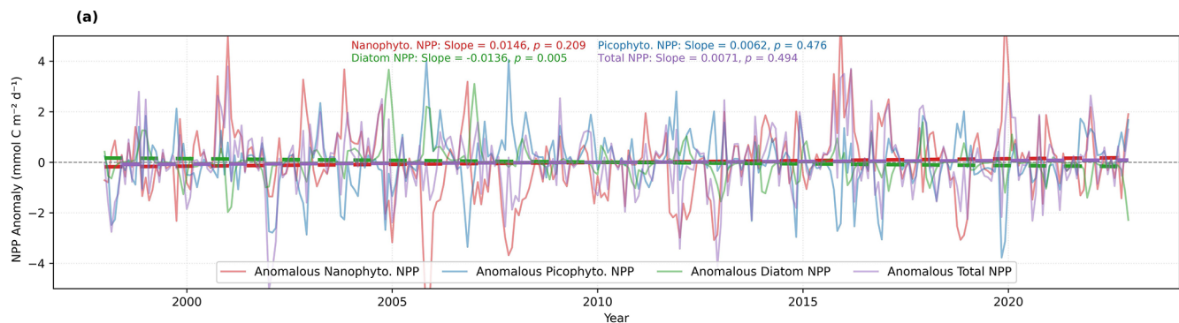
Figure 10. (a) PISCES-Quota-Fe simulated class specific NPP monthly anomalies (thin lines), fitted with ordinary least squares trend regressions for the period 1998–2022 corresponding to the remote sensing record. (b) Extended NPP trend analysis over the full study simulation time series 1975–2022.
