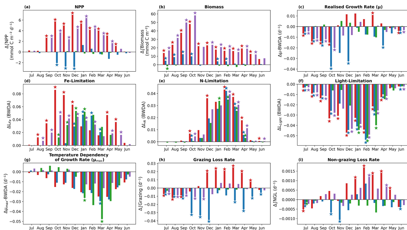
Figure 6. Simulated changes ( \Delta ) in phytoplankton class specific and total mean climatological terms determined from the mean climatological difference between high and low integrated total NPP seasons for: (a) depth integrated \Delta NPP, (b) depth integrated \Delta Biomass, (c) biomass-weighted depth-averaged growth rate \Delta\mu , (d) biomass-weighted depth-averaged iron limitation, \Delta L_{Fe} (positive \Delta L_{Fe} indicates reduced iron limitation), (e) biomass-weighted depth-averaged nitrogen limitation \Delta L_N (positive \Delta L_N indicates reduced nitrate limitation), (f) biomass-weighted depth-averaged light limitation \Delta L_{light} (negative \Delta L_{light} indicates increased light limitation), (g) biomass-weighted depth-averaged growth rate temperature dependency \mu_{max} , (h) phytoplankton biomass normalized specific grazing loss rate \Delta Grazing, and (i) phytoplankton biomass normalized specific non-grazing loss rate \Delta NGL. Stars denote that mean monthly climatological difference in the selected high and low NPP season groups is significantly exceeds the full time series climatological variability at the p < 0.05 level (10 000 iteration random year group bootstrapping analysis).
