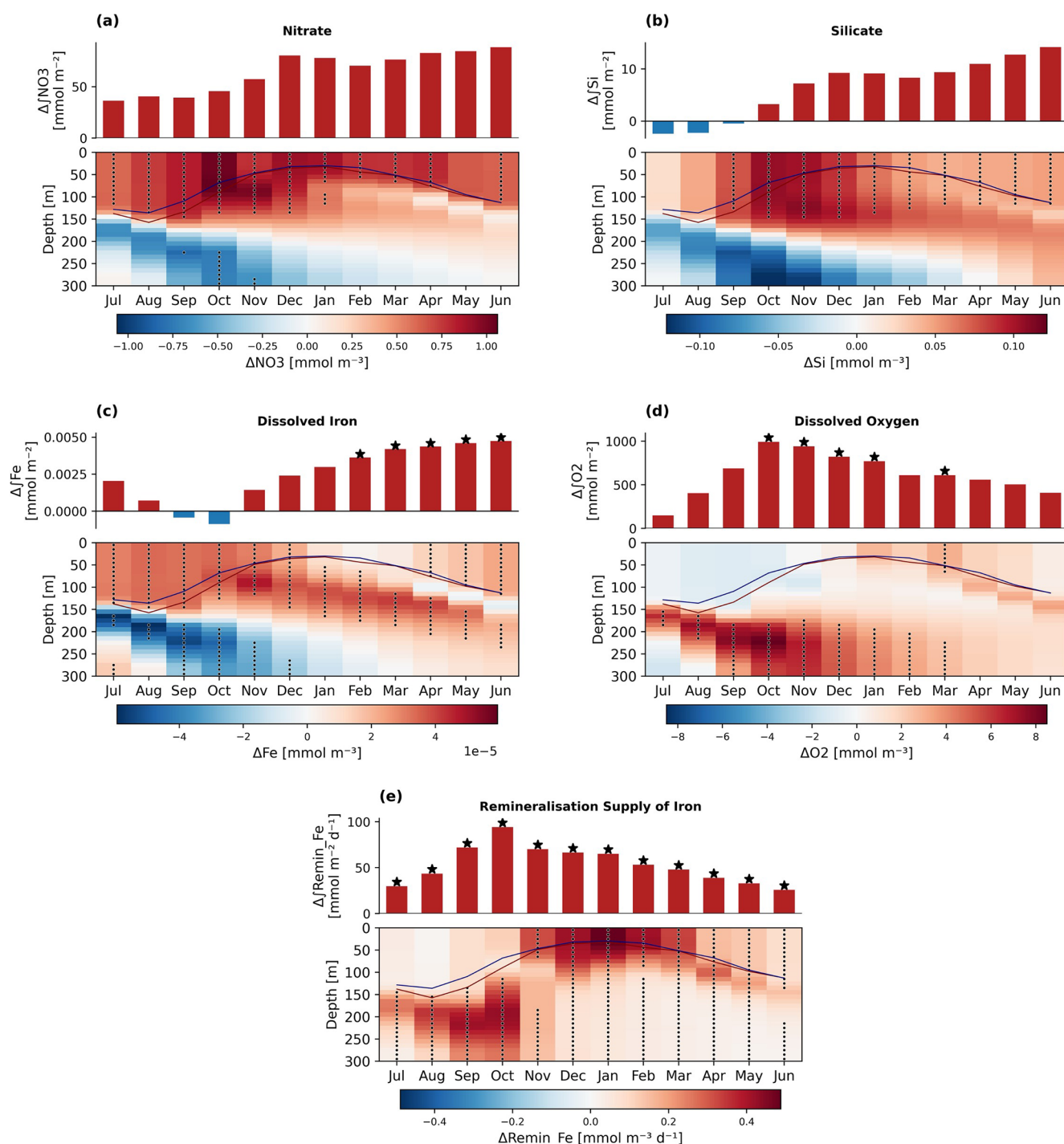
Figure 5. Climatological difference in simulated mean nutrient water column inventories (bar plots) and depth resolved concentration differences interpolated onto a 10 m regular grid (heatmaps) for (a) \Delta\text{NO}_3 , (b) \Delta\text{Si} , (c) \Delta\text{DFe} , (d) \Delta\text{O}_2 , and (e) the difference in the rate of remineralised iron supply ( \Delta\text{Remin\_Fe} ) between high and low NPP seasons. Stars and stippling indicate that mean monthly climatological difference in the selected high and low NPP season groups is significantly outside the full time series climatological variability at the p < 0.05 level (10 000 iteration random year bootstrapping analysis). Red and blue solid lines denote mean MLDs in respective high and low NPP year groups.
