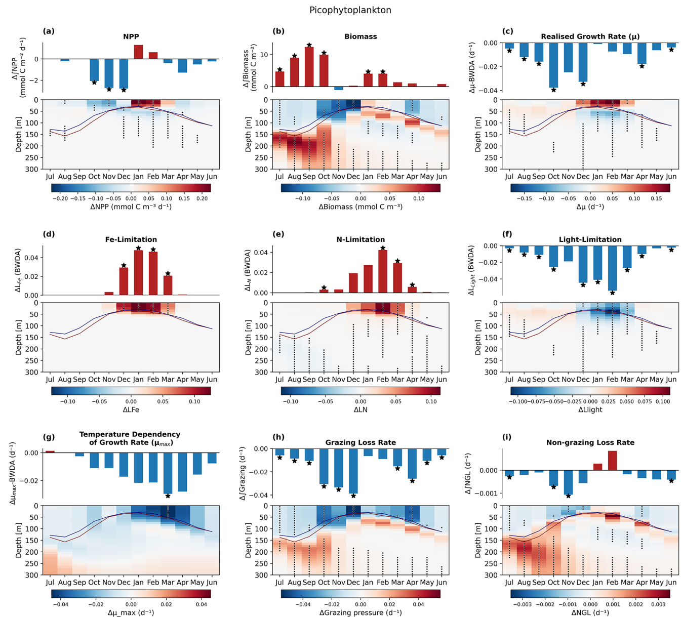
Figure A4. Simulated picophytoplankton class specific integrated (bar plots) and depth resolved (interpolated onto a 10 m regular grid) mean climatological (a) \Delta \text{NPP} (b) \Delta \text{Biomass} , (c) biomass-weighted depth-averaged growth rate \Delta \mu , (d) biomass-weighted depth-averaged iron limitation, \Delta L_{\text{Fe}} , (e) biomass-weighted depth-averaged nitrogen limitation \Delta L_{\text{N}} , (f) biomass-weighted depth-averaged light limitation \Delta L_{\text{light}} , (g) Biomass-weighted depth-averaged growth rate temperature dependency \mu_{\text{max}} , (h) phytoplankton biomass normalized specific grazing loss rate, \Delta \text{Grazing} , (i) phytoplankton biomass normalized specific non-grazing loss rate, \Delta \text{NGL} . \Delta terms were determined from the mean climatological difference between high and low integrated total NPP seasons. Stars denote that mean monthly climatological difference in the selected high and low picophytoplankton NPP season groups significantly exceeds the full time series climatological variability at the p < 0.05 level (10 000 iteration random year bootstrapping analysis).
