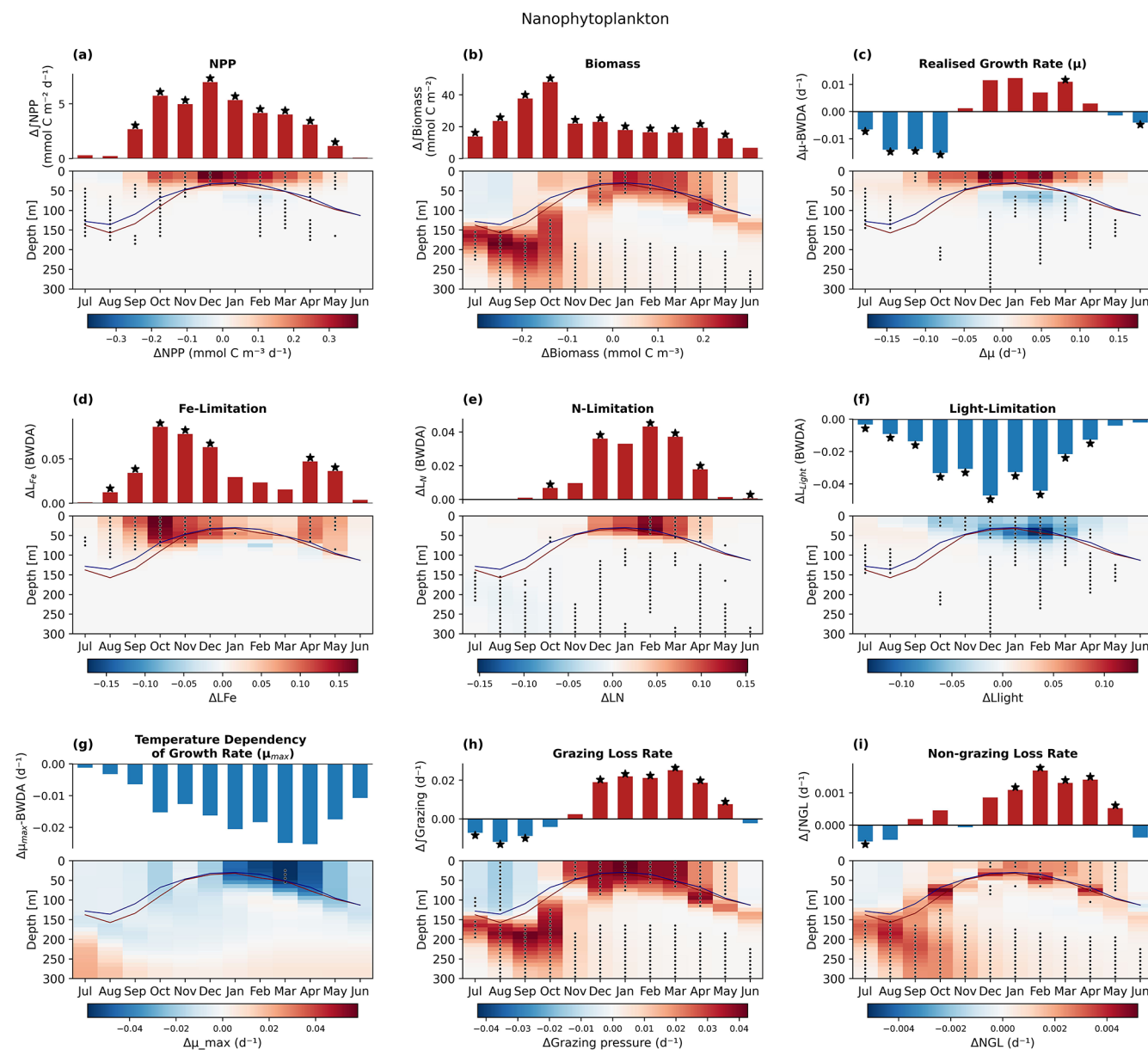
Figure A3. Simulated nanophytoplankton class specific integrated (bar plots) and depth resolved (interpolated onto a 10 m regular grid) mean climatological (a) \Delta\text{NPP} (b) \Delta\text{Biomass} , (c) biomass-weighted depth-averaged growth rate \Delta\mu , (d) biomass-weighted depth-averaged iron limitation, \Delta L_{\text{Fe}} , (e) biomass-weighted depth-averaged nitrogen limitation \Delta L_{\text{N}} , (f) biomass-weighted depth-averaged light limitation \Delta L_{\text{light}} , (g) Biomass-weighted depth-averaged growth rate temperature dependency \mu_{\text{max}} , (h) phytoplankton biomass normalized specific grazing loss rate, \Delta\text{Grazing} , (i) phytoplankton biomass normalized specific non-grazing loss rate, \Delta\text{NGL} . \Delta terms were determined from the mean climatological difference between high and low integrated total NPP seasons. Stars denote that mean monthly climatological difference in the selected high and low NPP season groups significantly exceeds the full time series climatological variability at the p < 0.05 level (10 000 iteration random year bootstrapping analysis).
