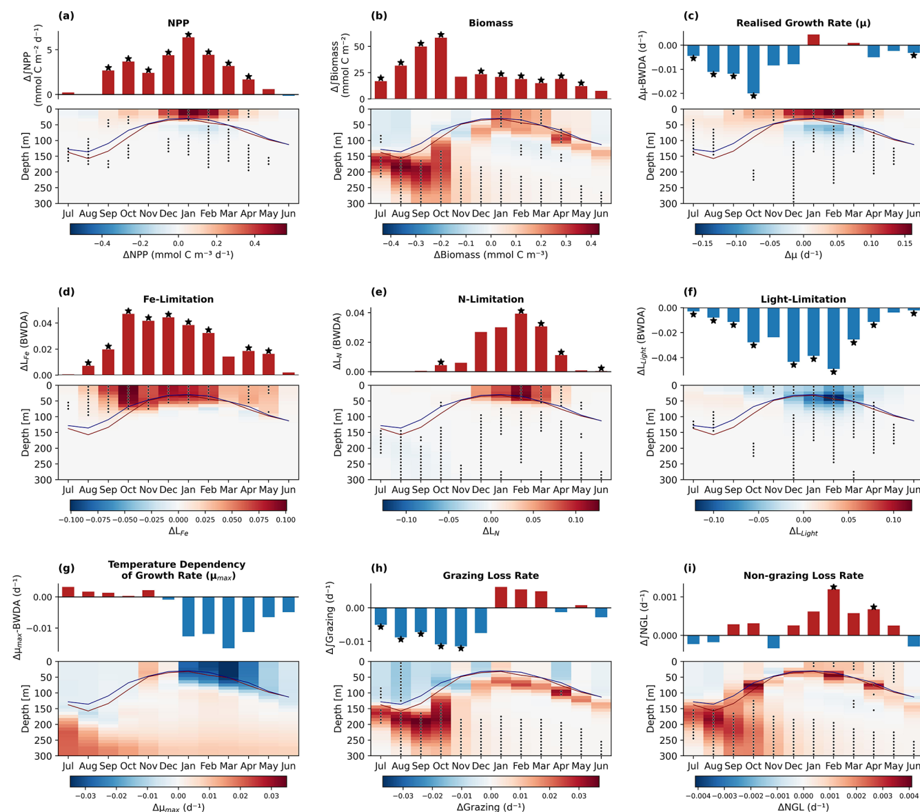
Figure 7. Simulated integrated (bar plots) and depth resolved (interpolated onto a 10 m regular grid) mean climatological (a) \Delta\text{NPP} , (b) \Delta\text{Biomass} , (c) biomass-weighted depth-averaged growth rate \Delta\mu , (d) biomass-weighted depth-averaged iron limitation, \Delta L_{\text{Fe}} , (e) biomass-weighted depth-averaged nitrogen limitation \Delta L_{\text{N}} , (f) biomass-weighted depth-averaged light limitation \Delta L_{\text{light}} , (g) Biomass-weighted depth-averaged growth rate temperature dependency \mu_{\text{max}} , (h) phytoplankton biomass normalized specific grazing loss rate \Delta\text{Grazing} , and (i) phytoplankton biomass normalized specific non-grazing loss rate \Delta\text{NGL} . \Delta terms were determined from the mean climatological difference between high and low integrated total NPP seasons. Stars and stippling denote that mean monthly climatological difference in the selected high and low NPP season groups significantly exceeds the full time series climatological variability at the p < 0.05 level (10 000 iteration random year bootstrapping analysis). Red and blue solid lines denote mean MLDs in respective high and low NPP year groups.
