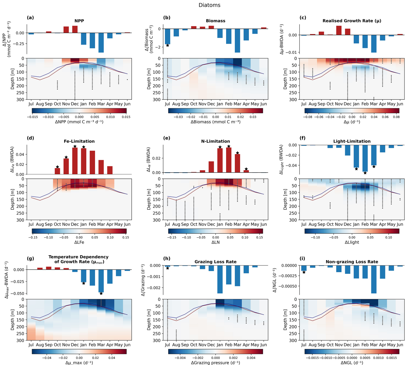
Figure A5. Simulated diatom class specific integrated (bar plots) and depth resolved (interpolated onto a 10 m regular grid) mean climatological (a) \Delta NPP (b) \Delta Biomass, (c) biomass-weighted depth-averaged growth rate \Delta\mu , (d) biomass-weighted depth-averaged iron limitation, \Delta L_{Fe} , (e) biomass-weighted depth-averaged nitrogen limitation \Delta L_N , (f) biomass-weighted depth-averaged light limitation \Delta L_{light} , (g) Biomass-weighted depth-averaged growth rate temperature dependency \mu_{max} , (h) phytoplankton biomass normalized specific grazing loss rate, \Delta Grazing, (i) phytoplankton biomass normalized specific non-grazing loss rate, \Delta NGL. \Delta terms were determined from the mean climatological difference between high and low integrated total NPP seasons. Stars denote that mean monthly climatological difference in the selected high and low diatom NPP season groups significantly exceeds the full time series climatological variability at the p < 0.05 level (10 000 iteration random year bootstrapping analysis).
