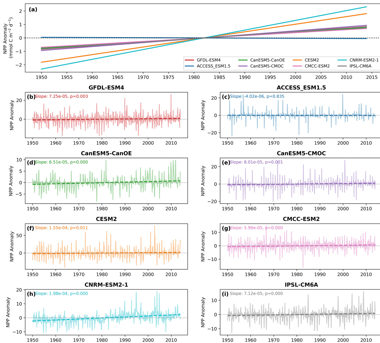
Figure A8. (a) Trends in monthly anomalous NPP time series from the 8 CMIP6 historical models listed in Table 2. (b–i) Individual CMIP6 model time series of spatial mean monthly NPP anomalies. Linear trends were calculated using ordinary least squares regression, with slope and p -values given for trends significantly different from zero (climate modes were not subtracted).
