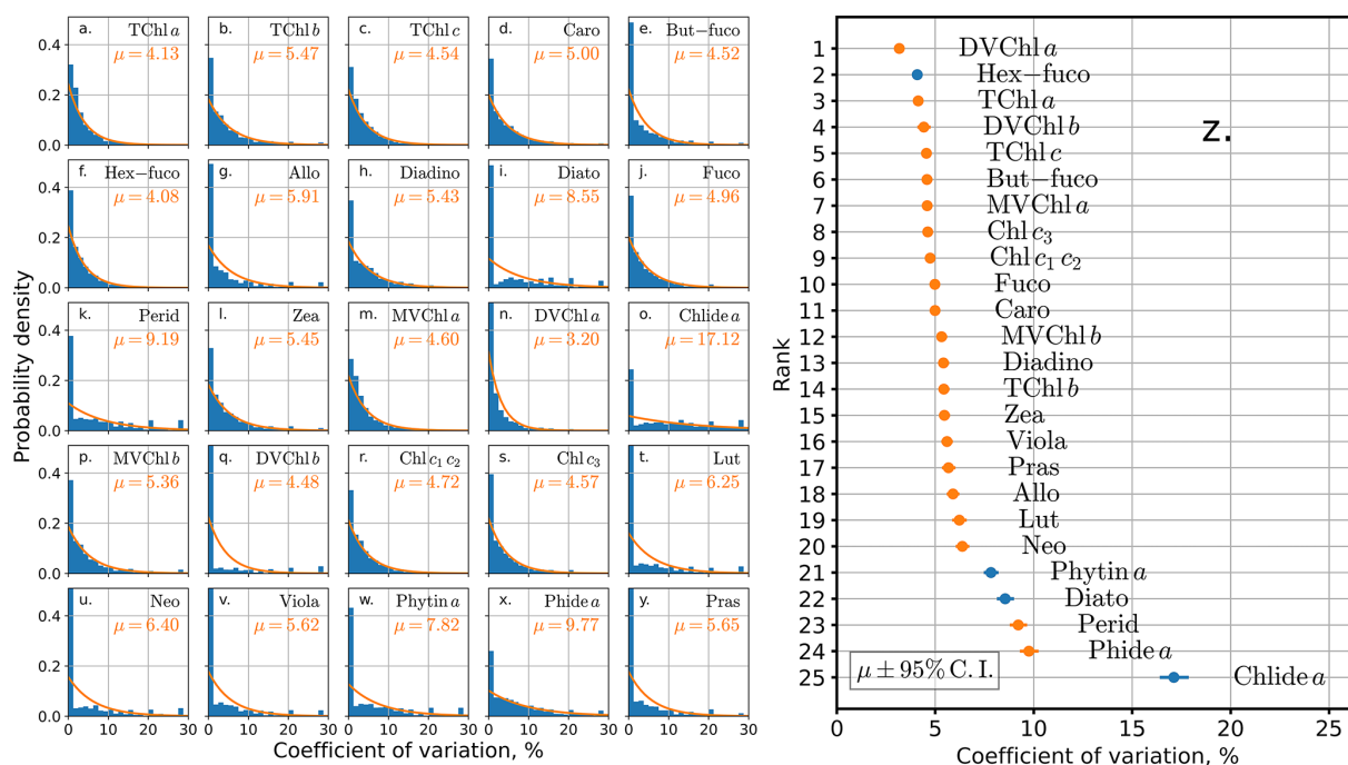
Figure 3. (a–y) Histograms of replicate sample precision (CV %) calculated for each phytoplankton pigment analyzed by HPLC from 2011–2022. Overlaid in orange is the exponential probability density function for each pigment, and \mu is mean precision. Panel (z) shows pigments ranked by precision. Blue symbols mark instances of non-overlapping confidence intervals with the next-lowest pigment.
