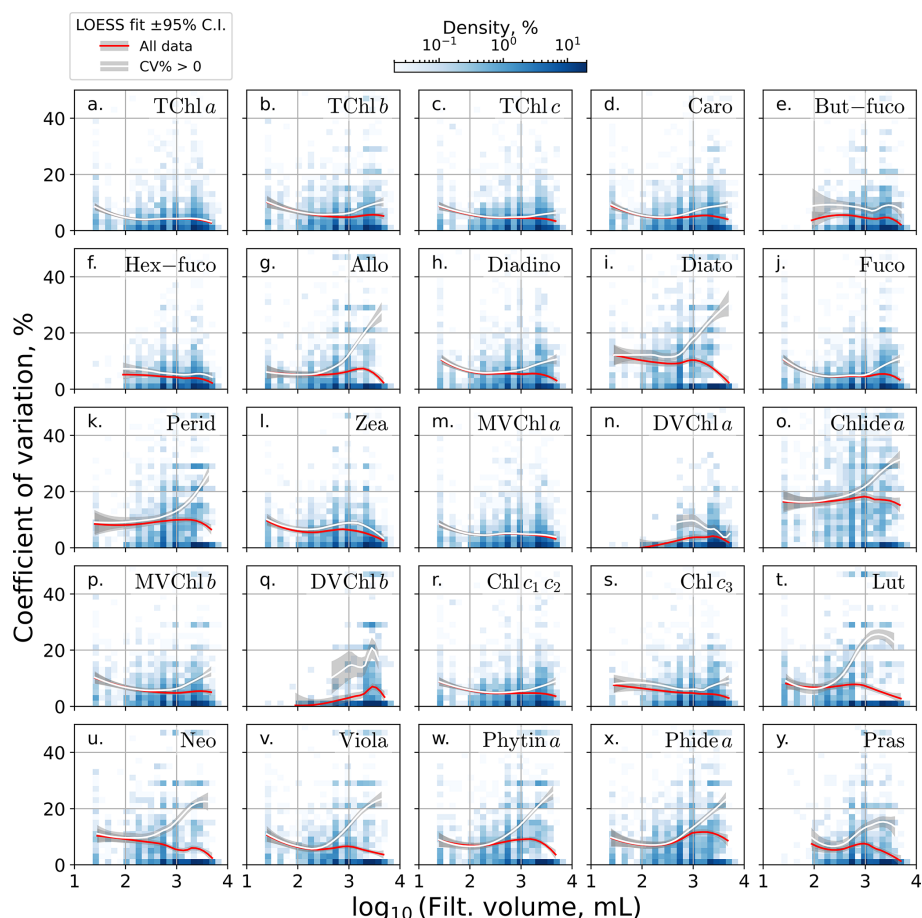
Figure 7. Replicate sample precision (CV %) versus \log_{10} -transformed filtered volume for each phytoplankton pigment. LOESS regression fits on all data (red line) and CV % > 0 only data (white line), with 95 % CIs shaded. 2D histograms display CV % sample density, with color bar showing percent sample density.
