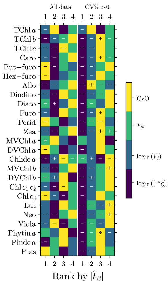
Figure 10. Variable importance rankings (1–4, based on normalized regression coefficient magnitudes |\hat{t}_\beta| ) from multivariate models predicting pigment precision. Left: full dataset. Right: censored dataset (CV % > 0, excluding invariant replicates). Symbols show effect direction: “+” = increases CV % (worsens precision), “–” = decreases CV % (improves precision), blank = non-significant ( \alpha = 0.05 ). Variables [color-coded]: \log_{10}([Pig]) = pigment concentration, \log_{10}(V_f) = filtered volume, F_m = microplankton fraction, CvO = coastal vs. oceanic.
