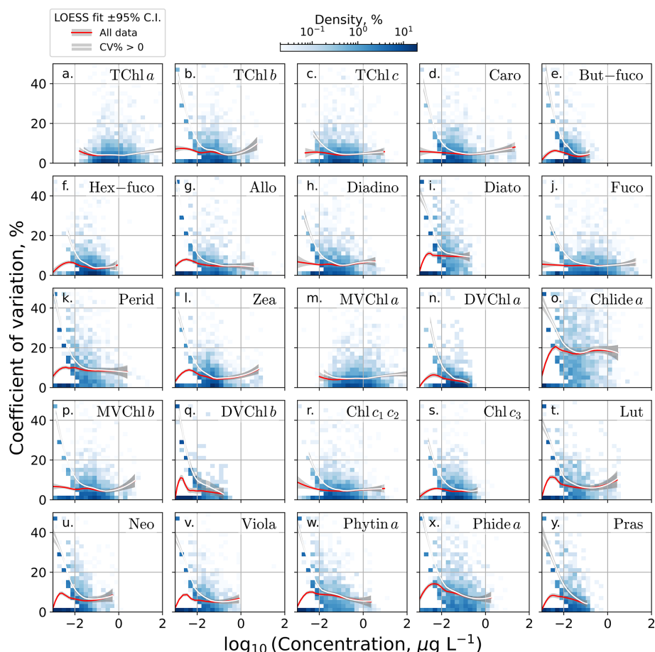
Figure 5. Replicate sample precision (CV %) versus \log_{10} -transformed pigment concentration for each phytoplankton pigment. LOESS regression fits on all data (red line) and CV % > 0 only data (white line), with 95 % CIs shaded. 2D histograms display CV % sample density, with color bar showing percent sample density.
