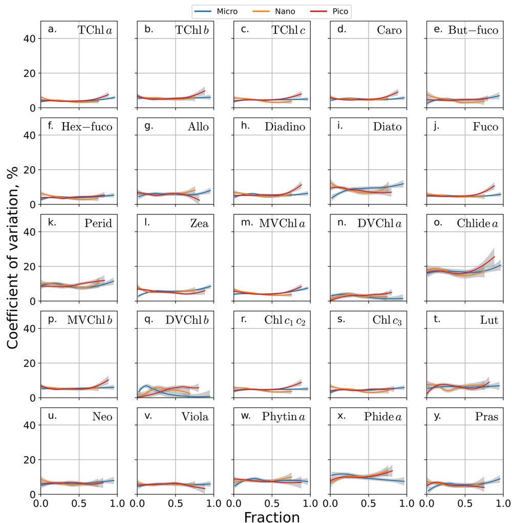
Figure A1. LOESS regression fits of sample precision (all data) versus estimated phytoplankton size fraction: micro ( > 20 \mu\text{m} ), nano ( 2\text{--}20 \mu\text{m} ), and picoplankton ( < 2 \mu\text{m} ) Eqs. (2)–(4). Shaded area contains 95 % confidence bands.
