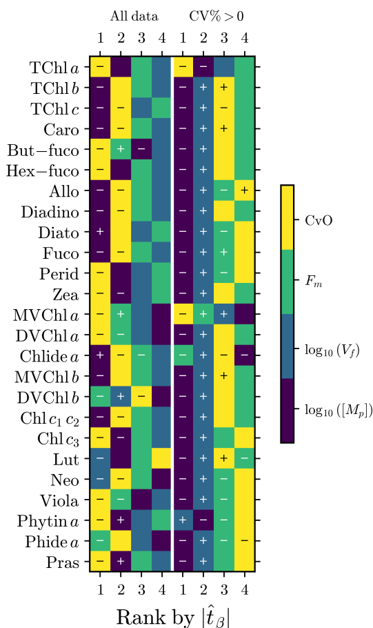
Figure B1. Variable importance rankings from multivariate regressions predicting pigment precision for full dataset (left) and censored data excluding invariant replicates (right). Rankings (1–4) based on absolute t -statistics ( \hat{t}_\beta ). Symbols indicate effect direction: “+” increases CV %, “–” decreases CV %, blank = non-significant ( \alpha = 0.05 ). Variables: \log_{10}(M_p) = pigment mass, \log_{10}(V_f) = filtered volume, F_m = microplankton fraction, CvO = coastal (0) vs. oceanic (1). Colors denote variables as per the colorbar.
