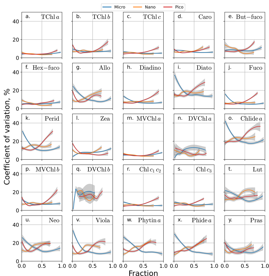
Figure 8. LOESS regression fits of replicate sample precision (CV % > 0) versus estimated phytoplankton size fraction: micro (> 20 \mu\text{m} ), nano (2–20 \mu\text{m} ), and picoplankton (< 2 \mu\text{m} ) Eqs. (2)–(4). Shaded area contains 95 % confidence bands.
