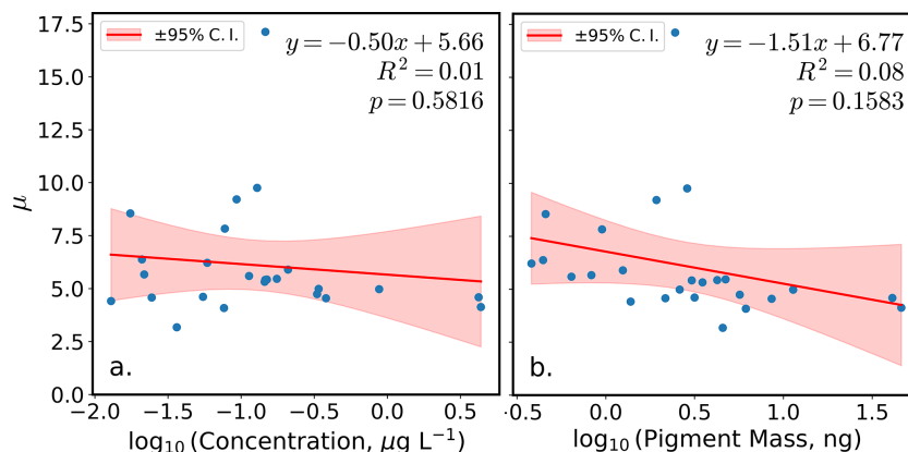
Figure 4. Mean coefficient of variation percentage (CV %) precision versus (a) mean \log_{10} -transformed pigment concentration, and (b) \log_{10} -transformed mean pigment mass. The adjusted R^2 quantifies goodness of fit, while the p -value tests significance of the slope.
