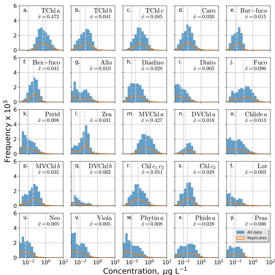
Figure 1. Distribution of phytoplankton pigment concentrations ( \text{mg m}^{-3} ) analyzed by HPLC at the NASA GSFC facility during 2011–2022. Bars indicate counts for all samples, while orange stairs show replicate sample fraction. Vertical lines denote the median concentration.
