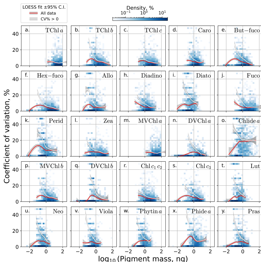
Figure 6. Replicate sample precision (CV %) versus \log_{10} -transformed pigment mass injected for each phytoplankton pigment. LOESS regression fits on all data (red line) and CV % > 0 only data (white line), with 95 % CIs shaded. 2D histograms display CV % sample density, with color bar showing percent sample density.
