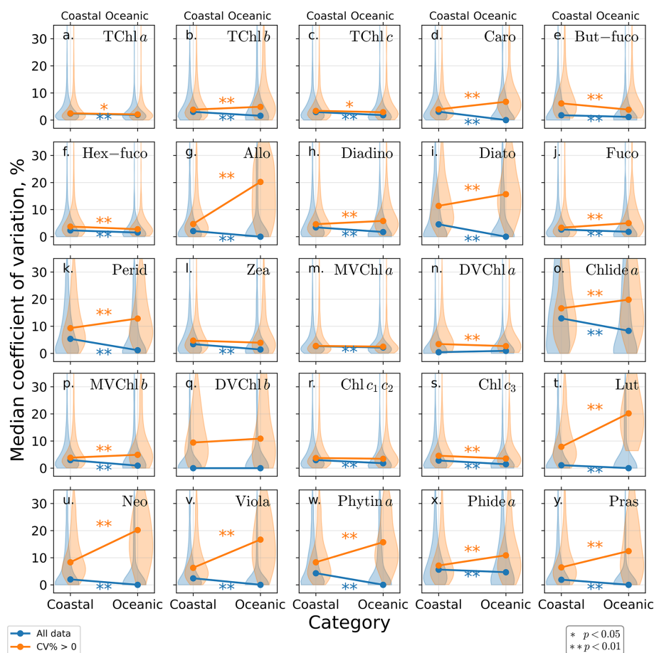
Figure 9. Lines depict the median sample precision (CV %) for phytoplankton pigments from coastal (< 200 km from shore) versus oceanic (> 200 km). Differences assessed using Mann-Whitney U test on full dataset (blue) and subset with CV > 0 only (orange). Violin plots depict CV % distribution per category. Comparisons marked “*” and “**” indicate statistically significant precision differences between coastal and oceanic at \alpha = 0.05 and \alpha = 0.01 , respectively.
