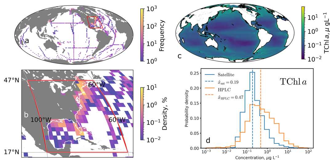
Figure 2. (a) Sample spatial distribution (bin counts), and (b) by percent of total samples for the North American region, which contains 41 % of analyzed samples over the 2011–2022 period included in this study. (c) Satellite-derived global total chlorophyll a concentration from MODIS-Aqua at 9 km resolution, averaged from 2002–2023. (d) Histograms comparing of satellite chlorophyll a concentration from (c) versus in situ total chlorophyll a measurements from HPLC analysis of samples collected globally from 2011–2022. Vertical lines mark the median concentration for each dataset.
