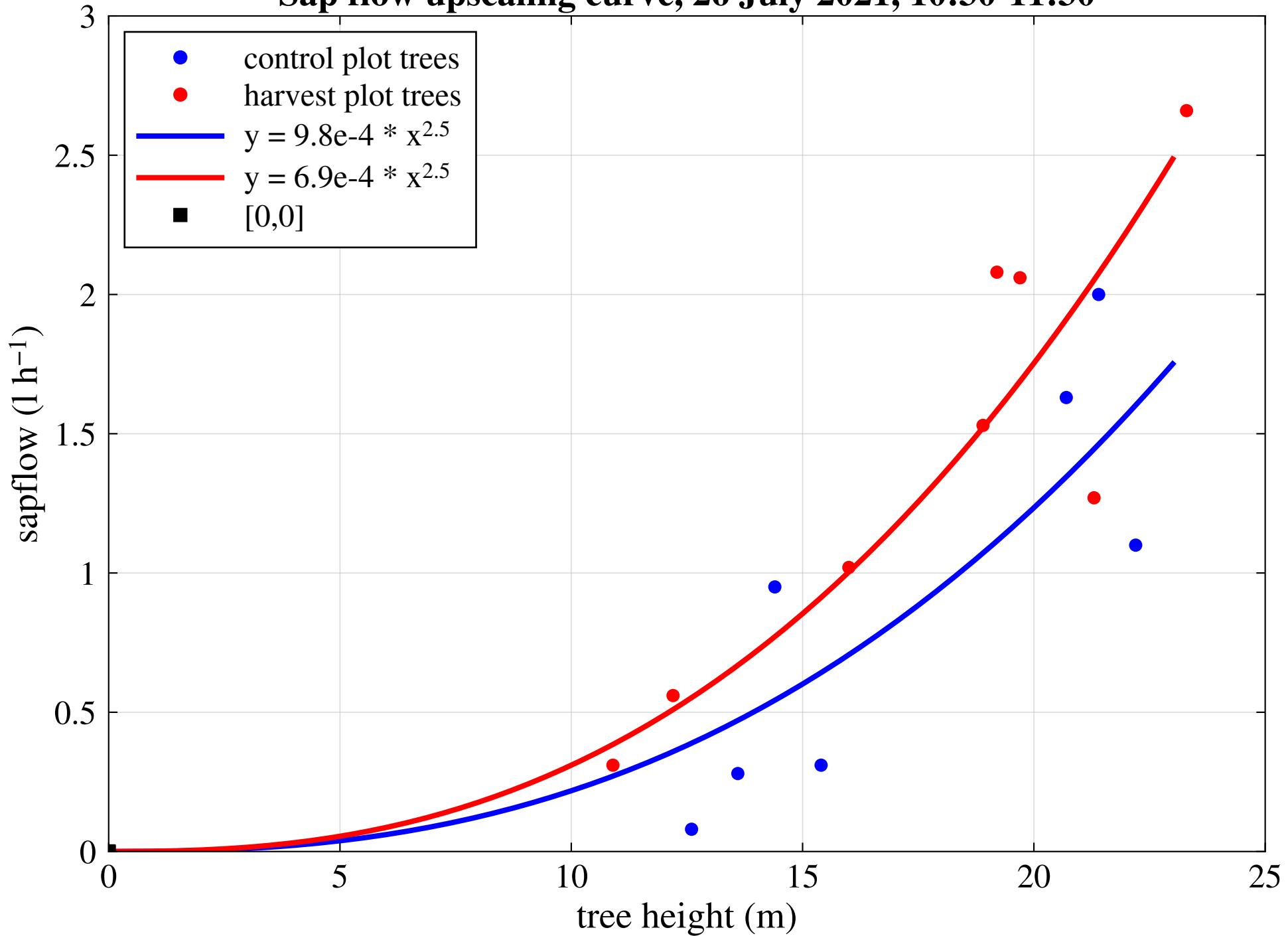
Sap flow upscaling curve, 26 July 2021, 10:30-11:30
