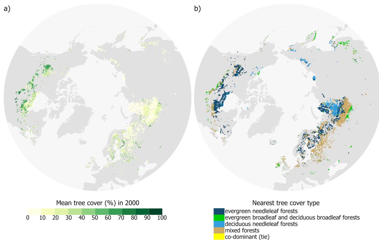
Figure A2. Mean tree cover in 2000 (a) and the nearest type of tree cover (b) in the studied northern peatlands.
