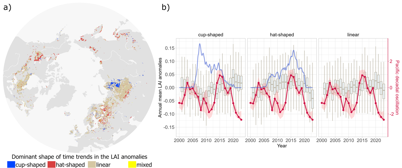
Figure 4. Spatial and temporal patterns of dominant LAI anomaly trends in northern peatlands. (a) Spatial distribution of the dominant trend shape in LAI anomalies, classified as cup-shaped, hat-shaped, linear, or mixed (where two or more shapes occurred with equal frequency within a hexagon). (b) Annual mean LAI anomalies (box plots) for pixels belonging to each trend type, overlaid with the density of posterior mean breakpoint years (blue line; higher values indicate more pixels with a breakpoint in that year) and the Pacific Decadal Oscillation (PDO) index (red line; shaded area shows 25 %–75 % quantiles).
