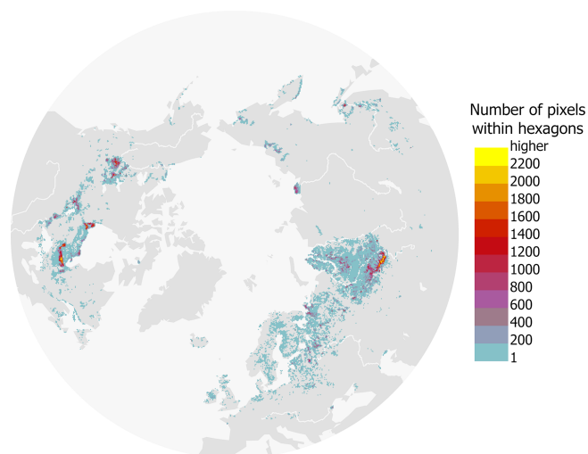
Figure 1. Study area and number of 500 m resolution pixels from the sensor-independent leaf area index raster within each 500 km 2 hexagon used for visualisation. The colour scheme indicates the number of LAI pixels with peatland coverage of 90 % or greater and without wildfire detected between 2001 and 2023.
