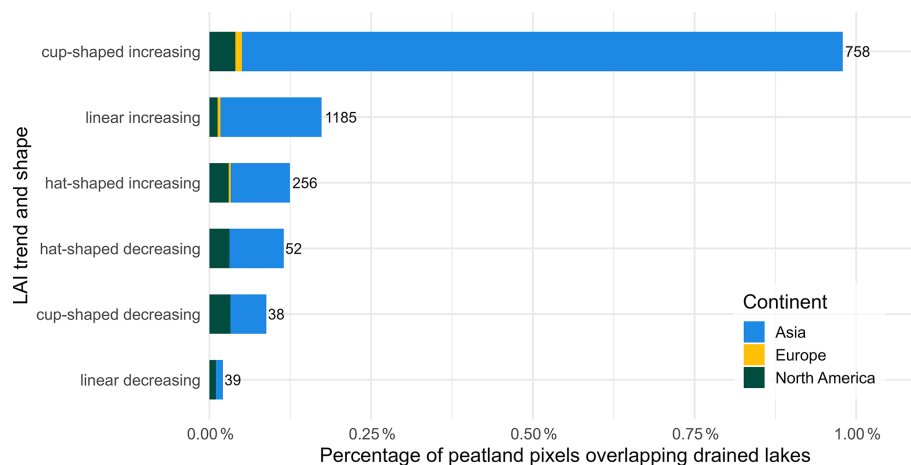
Figure 6. Proportion of peatland pixels that overlap drained-lake polygons by long-term LAI trend (increasing and decreasing) and trend-shape class. Horizontal bars indicate the share of pixels with a drained lake overlap greater than 0 %; coloured segments denote the continental composition (Asia, Europe, North America) of the overlapping pixels. Numbers at bar ends give the count of overlapping pixels. Classes are ordered by decreasing prevalence.
