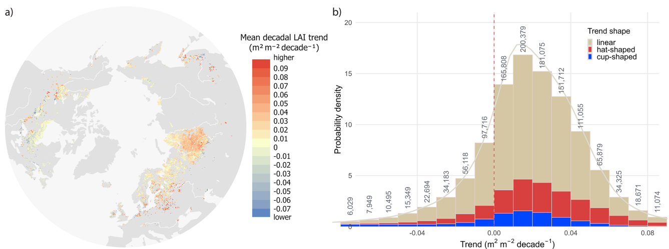
Figure 5. Spatial distribution and frequency of mean decadal LAI trends in northern peatlands (2001–2023). (a) Map of the mean decadal LAI trend, where warmer colours indicate stronger greening and cooler colours indicate browning. (b) Distribution of decadal trends shown as a density-scaled histogram, with bar fill indicating the dominant trend shape (linear, hat-shaped, cup-shaped). Numbers above bars are pixel counts per bin; the grey curve is the kernel density estimate, and the dashed vertical line marks zero trend.
