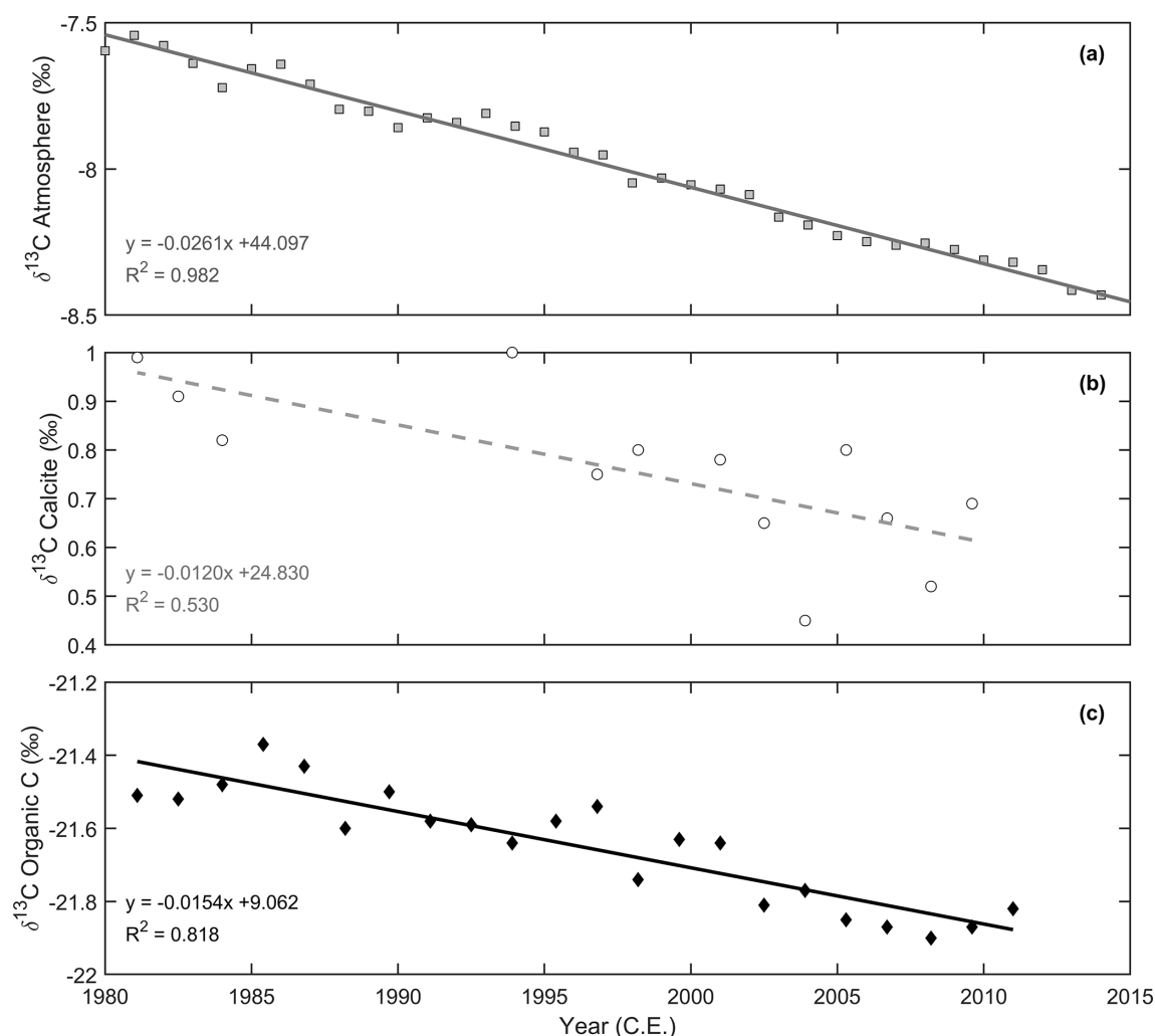
Figure 3. Linear regressions of \delta^{13}\text{C} (‰) records over the common interval used for trend comparison. (a) Atmospheric \delta^{13}\text{C} (‰) derived from instrumental observations. (b) \delta^{13}\text{C} of planktic foraminiferal calcite from N. dutertrei . (c) \delta^{13}\text{C} (‰) of sedimentary organic carbon. Regression equations and corresponding R^2 values are shown in each panel.
