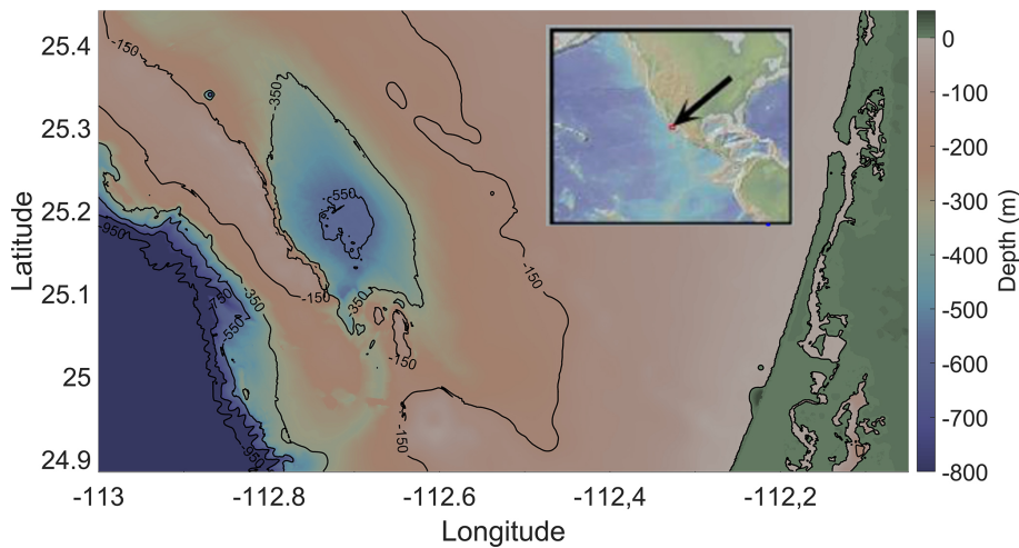
Figure 1. Localization of SLB, Baja California Sur, Mexico. The image was generated from GeoMapApp using the Global Multi-Resolution Topography (Ryan, et al., 2009) with modifications.
