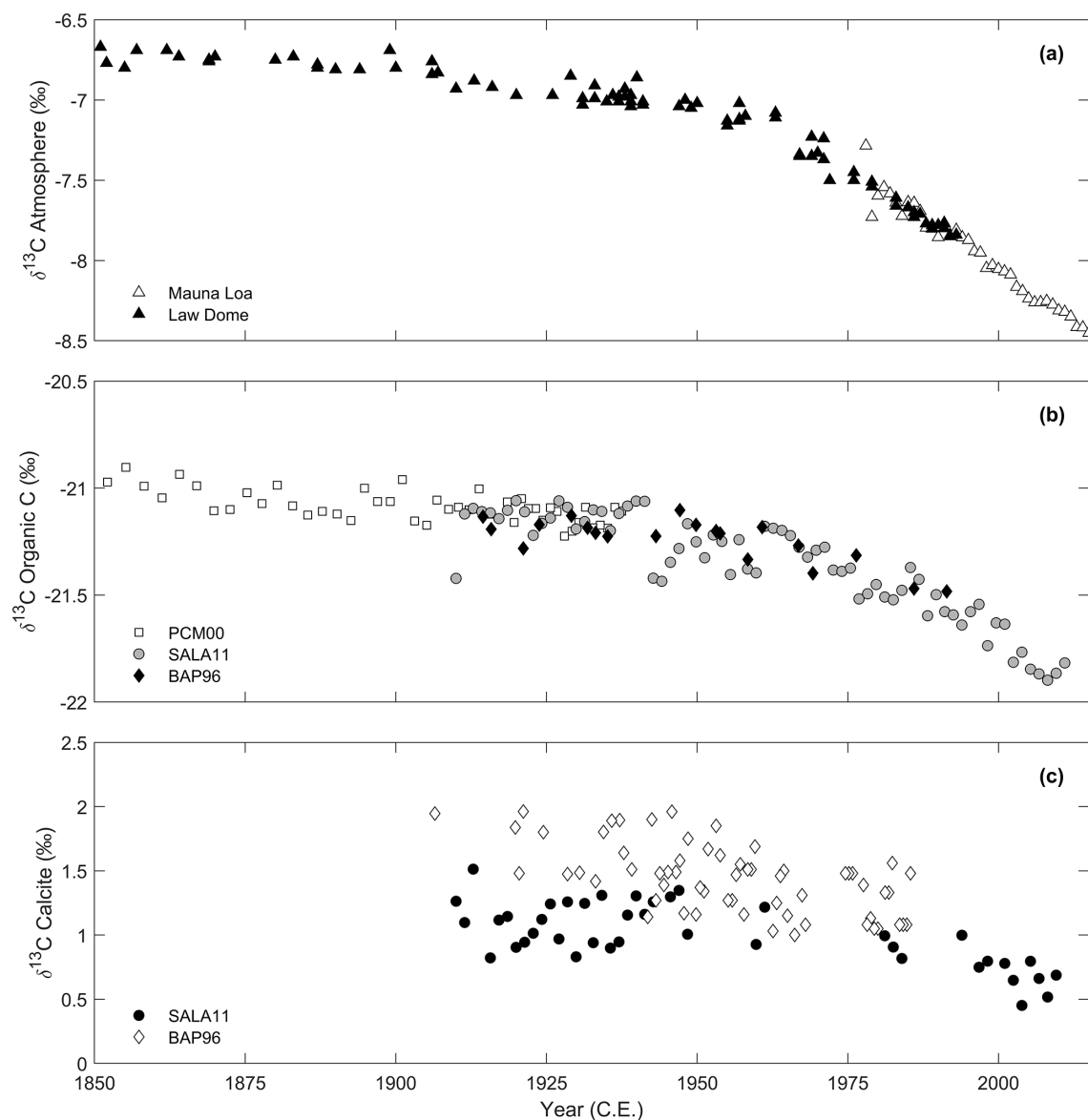
Figure 2. Time series of carbon isotopic composition from atmospheric and marine reservoirs. (a) Atmospheric \delta^{13}\text{C} (‰) values derived from the Law Dome ice-core record (Rubino et al., 2019) and instrumental measurements from Mauna Loa (Keeling et al., 2005); Scripps \text{CO}_2 Program database). (b) \delta^{13}\text{C} (‰) of sedimentary organic carbon from cores PCM00-78K, SALA11-E19MC-1, and BAP96-6C. (c) \delta^{13}\text{C} (‰) of planktic foraminiferal calcite from N. dutertrei (SALA11-E19MC-1) and G. ruber (BAP96-6C) obtained from sediment cores.
