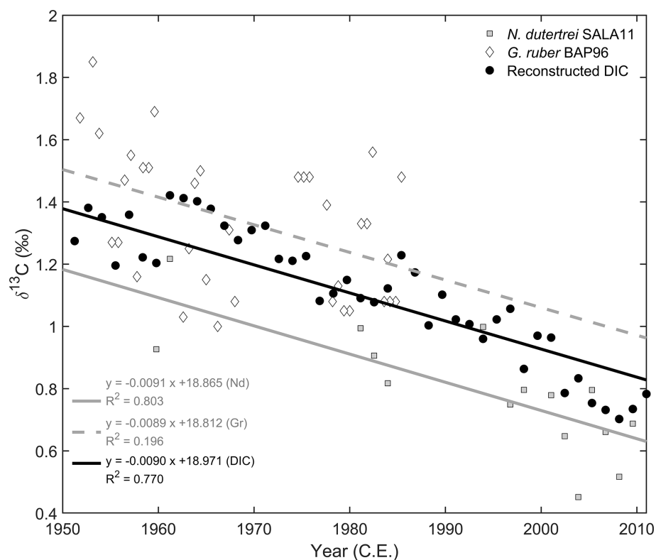
Figure 4. Time series and trends of the carbon isotopic composition of G. ruber (‰) (open diamonds) and N. dutertrei (‰) (black circles), as well as the DIC (‰) (grey squares), are derived from organic carbon in the sediments.
