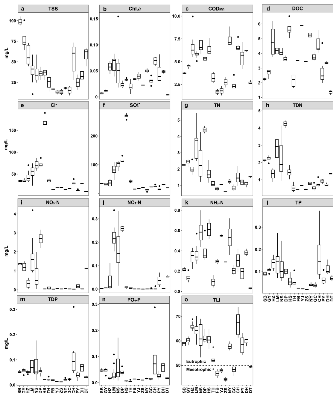
147 Figure S1 Water quality parameters of the Eastern China Plain Lakes
