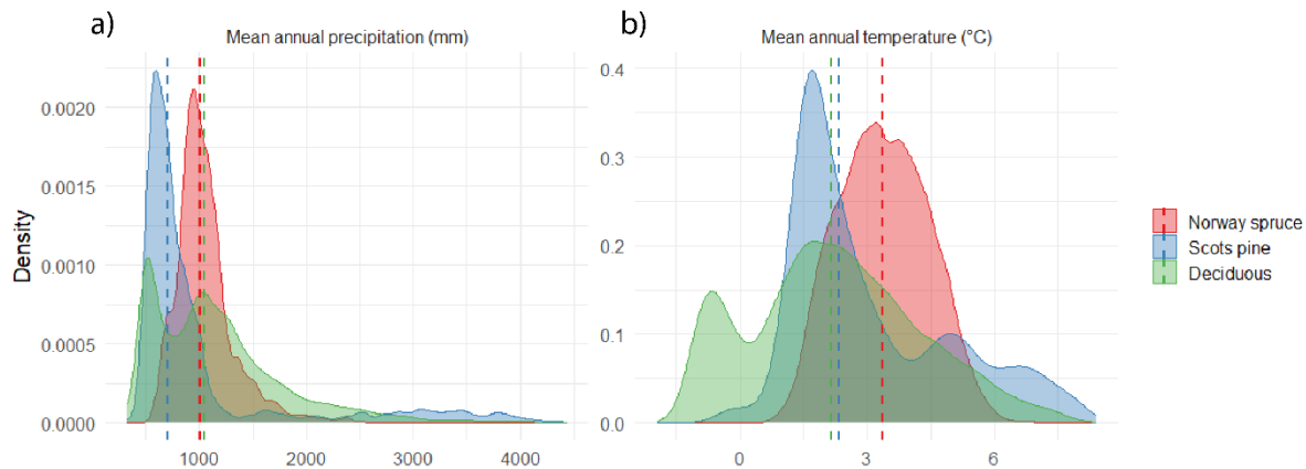
40 Figure S4: Density distributions of mean annual precipitation (a) and temperature (b). Vertical lines indicates the median values of the density distributions.
