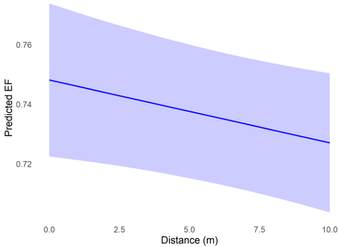
105 Figure S5: Predicted evaporative fraction for 400 m 2 and 1600 m 2 as function of edge distance. Predictions based on a linear mixed-effects model with distance as fixed effect and tree island as random intercept (EF = 0.748 + -0.0021 * Distance). EF decreased significantly with distance (-0.0021 ± 0.001 SE, p = 0.0386). The model explained 1.1% of the variance with fixed effects (marginal R 2 ), and 94.3% including random effects (conditional R 2 ).
