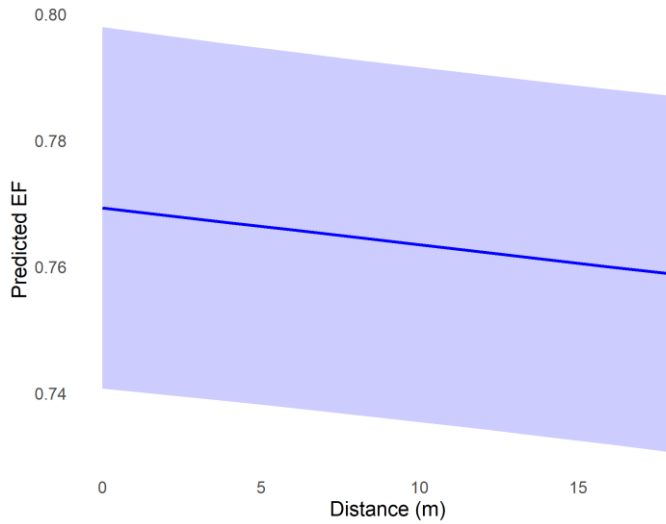
115 Figure S7: Predicted evaporative fraction for 1600 m 2 as function of edge distance. Predictions based on a linear mixed-effects model with distance as fixed effect and tree island as random intercept ( EF = 0.769 + -6e-04 * \text{Distance} ). EF decreased significantly with distance ( -0.00058 \pm 0.00024 SE, p = 0.016 ). The model explained 0.3% of the variance with fixed effects (marginal R^2 ), and 99.3% including random effects (conditional R^2 ).
