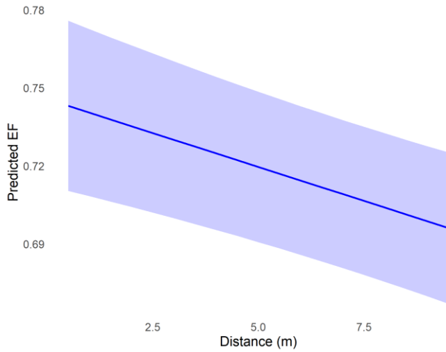
110 Figure S6: Predicted evaporative fraction for 400 m 2 as function of edge distance. Predictions based on a linear mixed-effects model with distance as fixed effect and tree island as random intercept ( EF = 0.746 + -0.0052 * \text{Distance} ). EF decreased significantly with distance ( -0.0052 \pm 0.00125 SE, p = 0.00004 ). The model explained 7% of the variance with fixed effects (marginal R^2 ), and 93.4% including random effects (conditional R^2 ).
