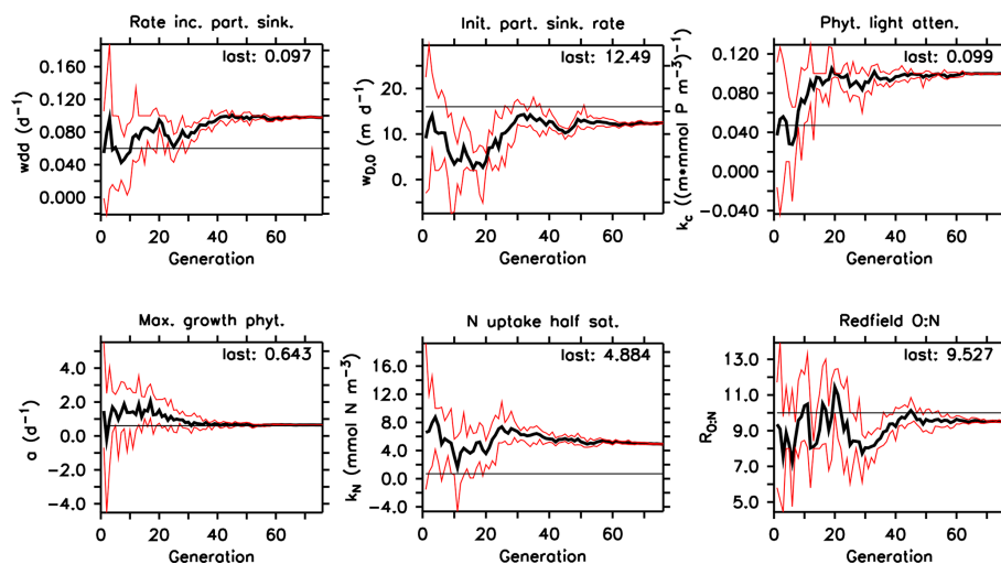
Figure 3. Resulting parameter values of the BL UVic ESCM biogeochemical parameter calibration, provided as an example of the evolution of the parameter optimisation. Thin black lines denote default model parameter values. Thick black lines are the average parameter values for all 10 individuals of a generation. Red lines are the maximum and minimum parameter values for each generation.
