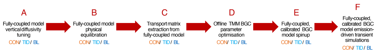
Figure 1. Work flow used in the model set-up and simulations. CON, TID, and BL stand for constant, tidal, and Bryan-Lewis vertical mixing schemes, respectively.
