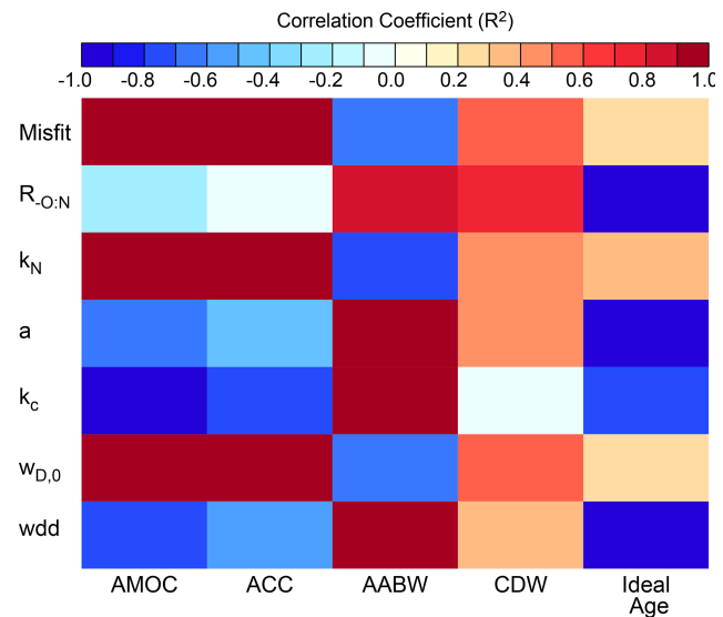
Figure 6. Mapping of optimal minimum misfit and optimal biogeochemical parameters to physical circulation metrics using calculation of the square of the Pearson product moment correlation coefficient, R^2 (colour coding).
