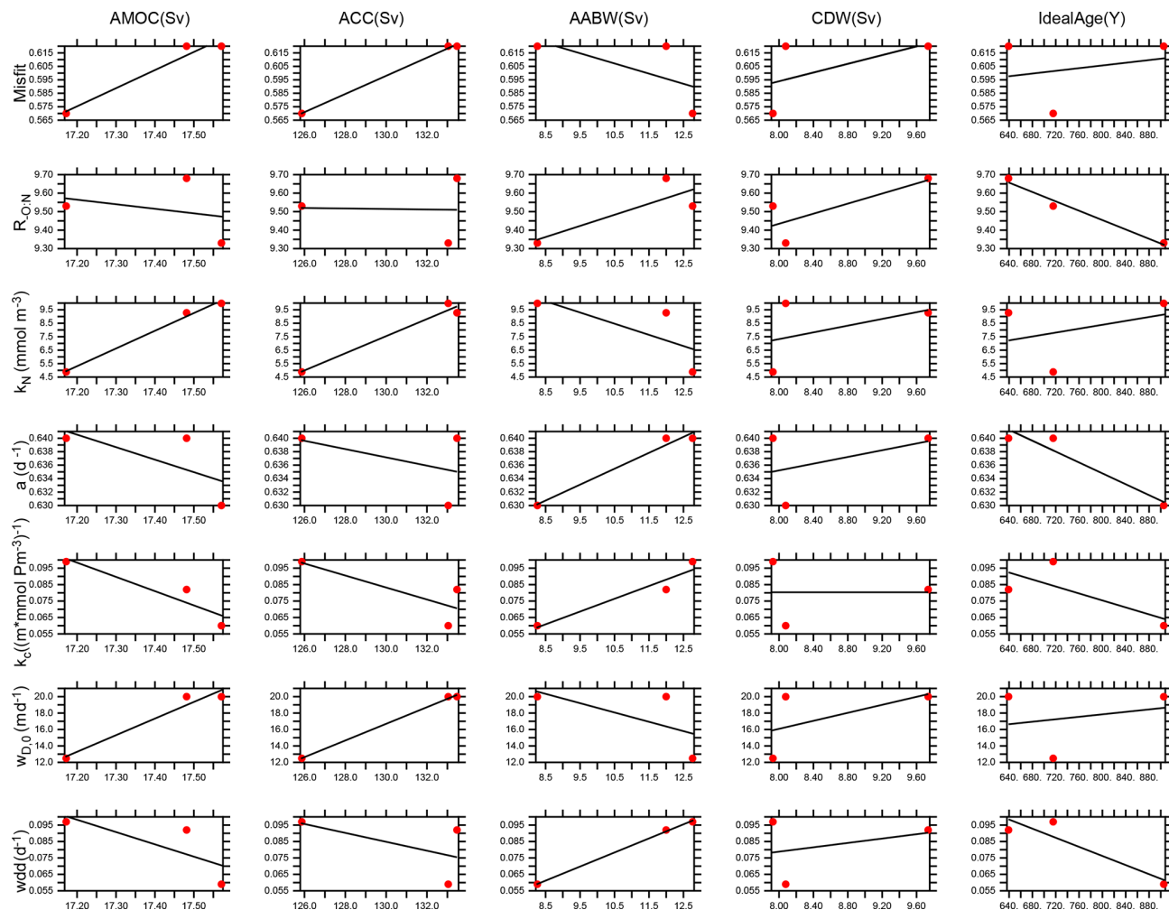
Figure A1. Calibrated model pre-industrial physical metrics ( x axes) versus optimal biogeochemical parameter value or minimum calibration misfit ( y axes); red dots. Linear regression lines; black line.
