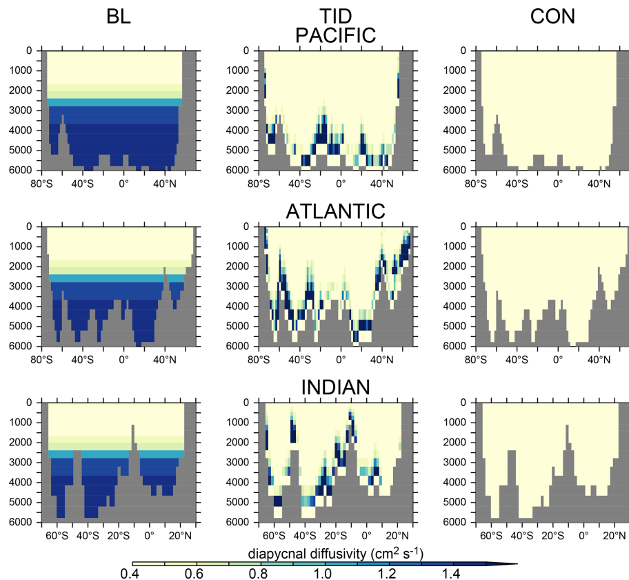
Figure 2. Longitudinal transects of diapycnal diffusivity at 150° W (Pacific Ocean), 30° W (Atlantic Ocean) and 65° E (Indian Ocean) for the three mixing parametrisations. See Table 1 for background k_v values.
