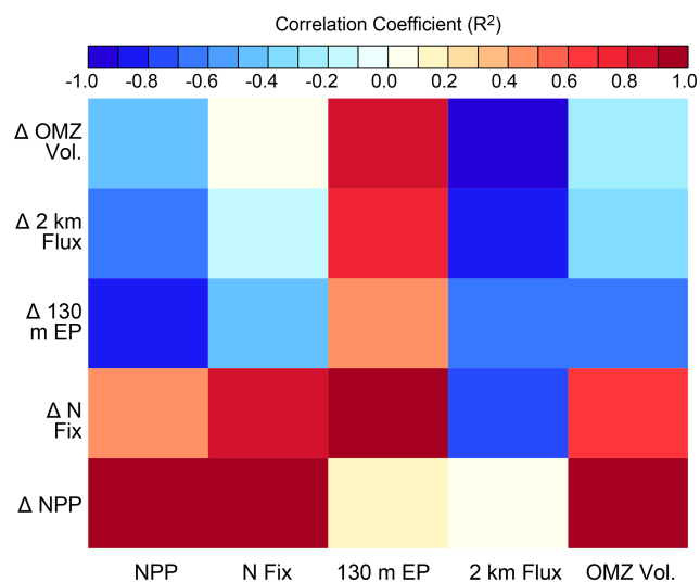
Figure 14. Mapping of pre-industrial biogeochemical metrics ( x axis) and from pre-industrial to year 2300 change in biogeochemical metrics ( y axis) using calculation of the square of the Pearson product moment correlation coefficient, R^2 (colour coding).
