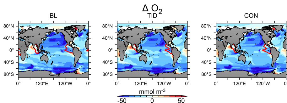
Figure 15. Change in oxygen concentration at 300 m depth (years 2300–1765) for all three calibrated models. Regions where concentrations are below 5 \text{ mmol O}_2 \text{ m}^{-3} at year 2300 are delineated in red to highlight regions in which denitrification occurs.
