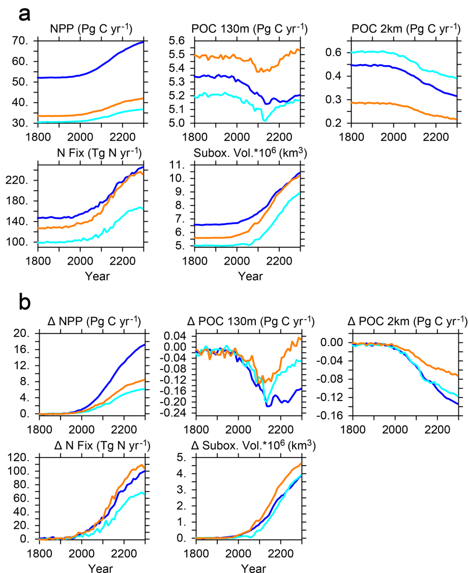
Figure 12. (a) Global biogeochemical metrics for all three calibrated models. Suboxic volume is calculated using a 5 \text{ mmol O}_2 \text{ m}^{-3} threshold. (b) Global biogeochemical response to \text{CO}_2 emissions forcing for all three calibrated models ( \Delta , year – pre-industrial value). Dark blue is BL, light blue is TID, orange is CON.
