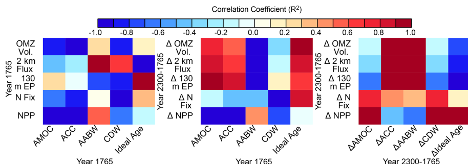
Figure 9. Mapping of pre-industrial circulation metrics ( x axis, left and middle plot) and year 2300 change ( \Delta ) in circulation metrics ( x axis, right plot) against biogeochemical metrics (pre-industrial, y axis of left plot, year 2300 change in, y axis of middle and right plot) using calculation of the square of the Pearson product moment correlation coefficient, R^2 (colour coding).
