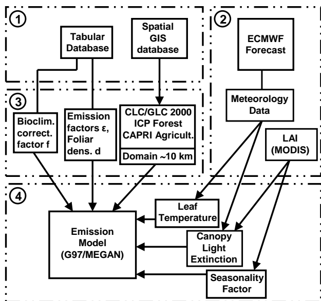
Fig. 1. BVOC emission model, schematic overview.
