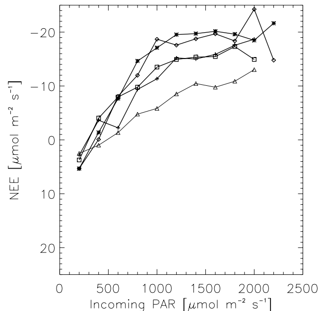
Fig. B1. Light response of NE_E measured by eddy correlation averaged over 200 \mu\text{mol quanta m}^{-2} \text{s}^{-1} bins at the different tower sites. Data used correspond to the period July–December. \Delta Tapajos, * Man K34, \diamond Jaru, \square Caxiuana, + Man C14.
