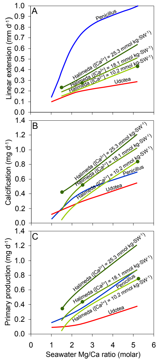
Fig. 7. Rates of linear extension ( A ), calcification ( B ), and primary production ( C ) for Halimeda incrassata (dark green curve: [Ca^{2+}] = 25.3 \text{ mmol kg-SW}^{-1} ; medium green curve: [Ca^{2+}] = 18.1 \text{ mmol kg-SW}^{-1} ; light green curve: [Ca^{2+}] = 10.2 \text{ mmol kg-SW}^{-1} ), Penicillus capitatus (blue curve), and Udotea flabellum (red curve) algae reared in experimental seawaters of modified Mg/Ca and [Ca^{2+}] . Rates of linear extension, calcification, and primary production increase significantly ( p < 0.05 ) for H. incrassata with both increasing seawater Mg/Ca ( [Ca^{2+}] fixed) and increasing seawater [Ca^{2+}] (Mg/Ca fixed). Rates of linear extension, calcification, and primary production also increase significantly ( p < 0.05 ) with elevations in seawater Mg/Ca that are formulated with geologically realistic (Hardie, 1996; Demicco et al., 2005) reductions in [Ca^{2+}] for all three species of calcifying algae ( H. incrassata = closed green circles; P. capitatus = blue curve; U. flabellum = red curve). Primary production is calculated as total dry weight minus weight of CaCO_3 . Data from Ries (2005a, b, 2006a); Stanley et al. (2010).
