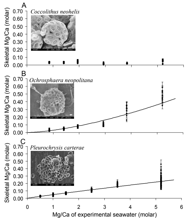
Fig. 16. Mg/Ca ratio of calcite secreted by coccolithophore species Cocolithus neohelis ( A ), Ochrosphaera neopolitana ( B ), and Pleurochrysis carterae ( C ) as a function of the Mg/Ca ratio of the experimental seawater in which they were reared. Error bars represent standard error of microprobe analysis. Fitted curves are power functions fit to the data using least squares regressions. From Stanley et al. (2005).
