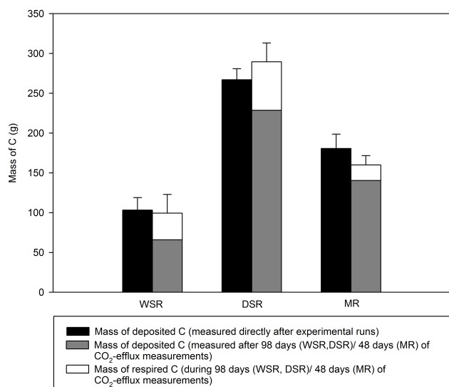
Fig. 6. Comparison between the mass of deposited C, directly after the experimental runs (M1) and the sum of the mass of respired CO 2 -C and the mass of C in deposited sediments after CO 2 -efflux measurements (M2).
