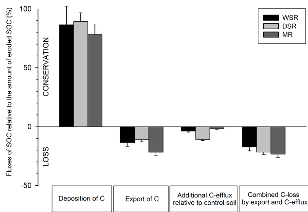
Fig. 7. Fate of eroded SOC (%) in the three simulation experiments, expressed relative to the total amount of eroded SOC.
