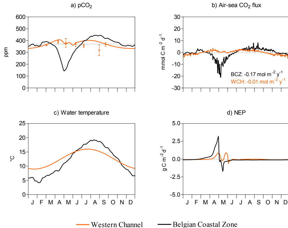
Fig. 6. Seasonal evolution of daily modelled (a) pCO 2 , (b) air-sea CO 2 flux, (c) water temperature and (d) net ecosystem production computed for WCH and BCZ boxes. Model results of pCO 2 in WCH (solid line) are compared with available observations in that area (◇). The dotted line, in the pCO 2 plots, corresponds to atmospheric pCO 2 . The calculated annual CO 2 air-sea flux is added to each plot of air-sea CO 2 flux.
