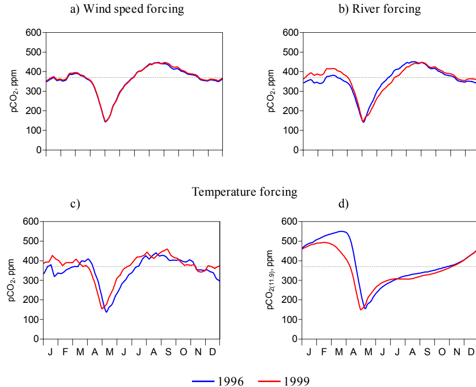
Fig. 8. Seasonal evolution of modelled pCO 2 computed with (a) wind speed forcing, (b) river (c) temperature forcings of 1996 and 1999 and (d) same as (c) but normalized to BCZ average temperature of 11.9°C. The dotted line corresponds to atmospheric equilibrium.
