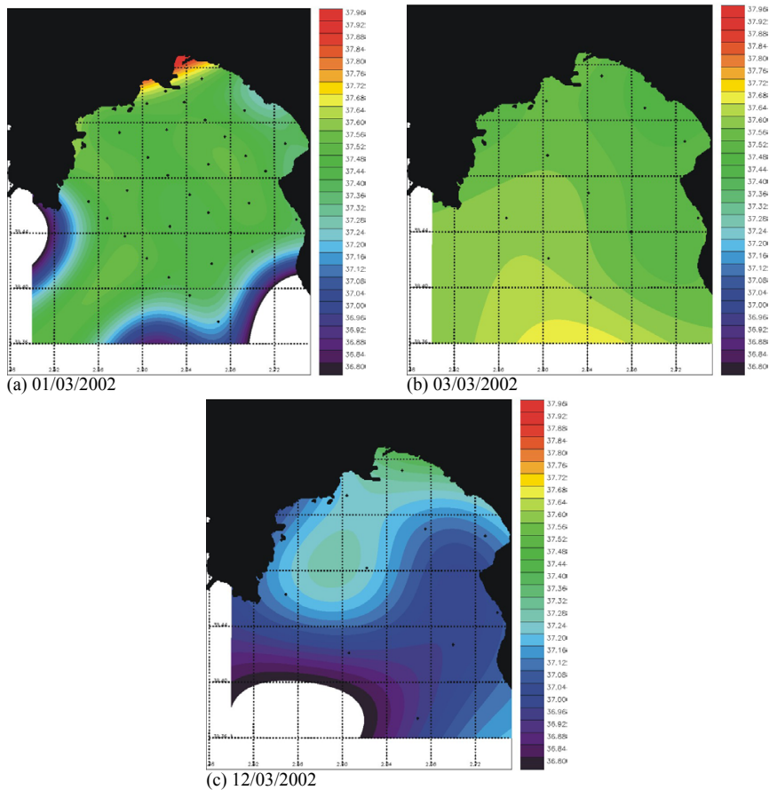
Fig. 4. Salinity distribution during EUBAL-I at 2 m for (a) 01 March 2002, (b) 03 March 2002; (c) 12 March 2002.
