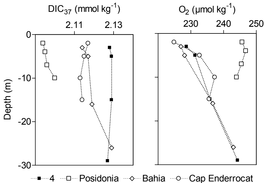
Fig. 10. Vertical profiles of DIC normalized to a constant salinity ( DIC 37 in mmol kg -1 ) and O 2 (µmol kg -1 ) at four reference stations (cf. Fig. 1).
