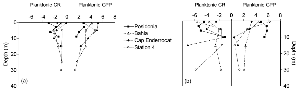
Fig. 5. Depth profiles of planktonic daily CR and GPP ( \text{mmolO}_2 \text{m}^{-3} \text{d}^{-1} ) measured at four stations in the Bay of Palma during (a) EUBAL-I and (b) EUBAL-II cruises (cf. Fig. 1).
