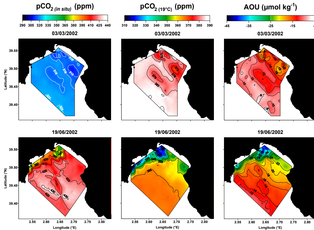
Fig. 8. Surface distributions of p\text{CO}_{2(\text{in situ})} (ppm), p\text{CO}_{2} normalized to a constant temperature ( p\text{CO}_{2(19^\circ\text{C})} , ppm) and AOU ( \mu\text{mol kg}^{-1} ) obtained on 3 March 2002 (EUBAL-I cruise) and 19 June 2002 (EUBAL-II cruise).
