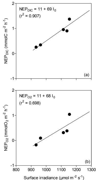
Fig. 9. NEP_{DIC} (A; \text{mmolC m}^{-2} \text{h}^{-1} ) and NEP_{O_2} (B; \text{mmol O}_2 \text{m}^{-2} \text{h}^{-1} ) over the Posidonia oceanica meadow versus surface irradiance ( I_0 ; \mu\text{mol m}^{-2} \text{s}^{-1} ) during the EUBAL-II cruise. NEP_{DIC} and NEP_{O_2} data were adjusted linearly to 12:00 Universal Time (UT; all surveys ended in mid-afternoon, ranging from 14:30 to 16:45 UT). Surface irradiance was averaged from dawn to 12:00 UT.
