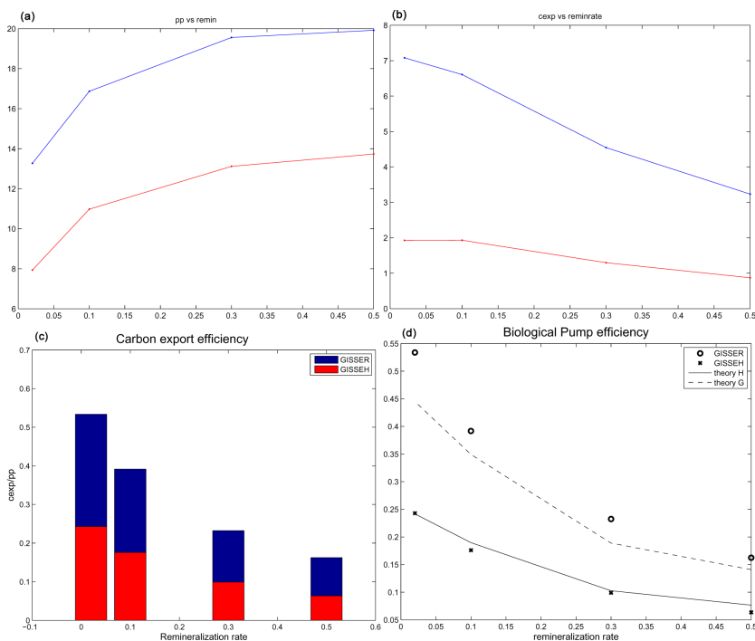
Fig. 8. (a) Vertically averaged PP as a function of remineralization rate. The vertical axis is global integral PP in \text{PgCyr}^{-1} and the horizontal axis is remineralization rate in \text{d}^{-1} . Blue line is for GISSER and the red line for GISSEH. (b) Globally integrated carbon export across 75 m ( \text{cexp} , in \text{PgCyr}^{-1} ) as a function of the remineralization rate (in \text{d}^{-1} ), (c) globally integrated efficiency of the biological pump (ratio of the carbon export at 75 m and primary productivity), (d) change of the carbon export efficiency with the remineralization rate in the two NASA-GISS climate models (circles GISSER, crosses GISSEH). Continuous lines depict analytic solutions obtained using Eq. (7).
