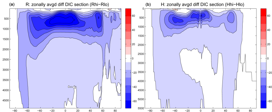
Fig. 11. Differences in the DIC zonally averaged vertical sections between same model runs with varying remineralization rates.
