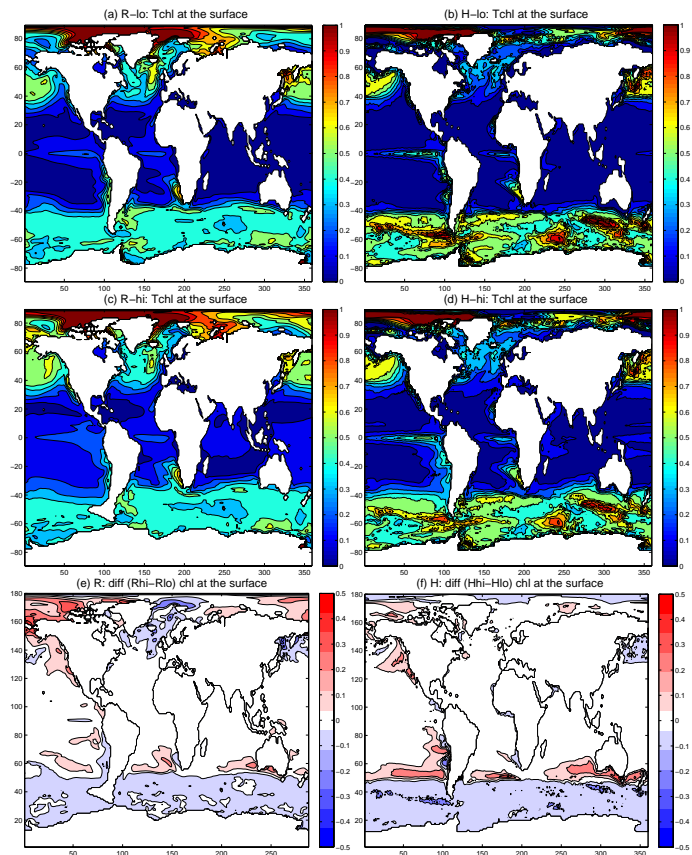
Fig. 5. Surface distributions of chlorophyll in (a) GISSER and (b) GISSER with low remineralization rate, (c) GISSER and (d) GISSER with high remineralization rate. Units are in \text{mg C m}^{-3} . (e, f) Differences in surface chlorophyll between same model runs but with varying remineralization rate. Units are in \text{mg C m}^{-3} .
