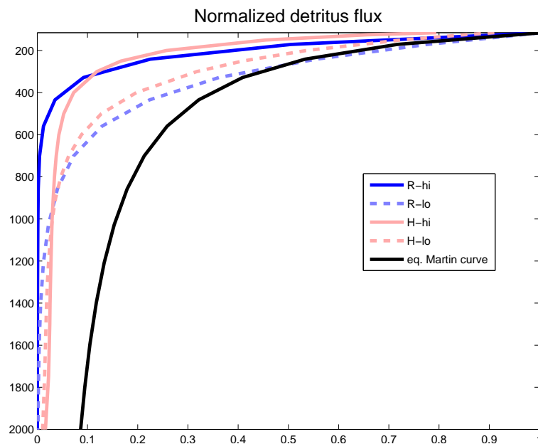
Fig. 3. Normalized detritus flux and comparison to the theoretical Martin curve. In blue: GISSER, in red: GISSEH.
