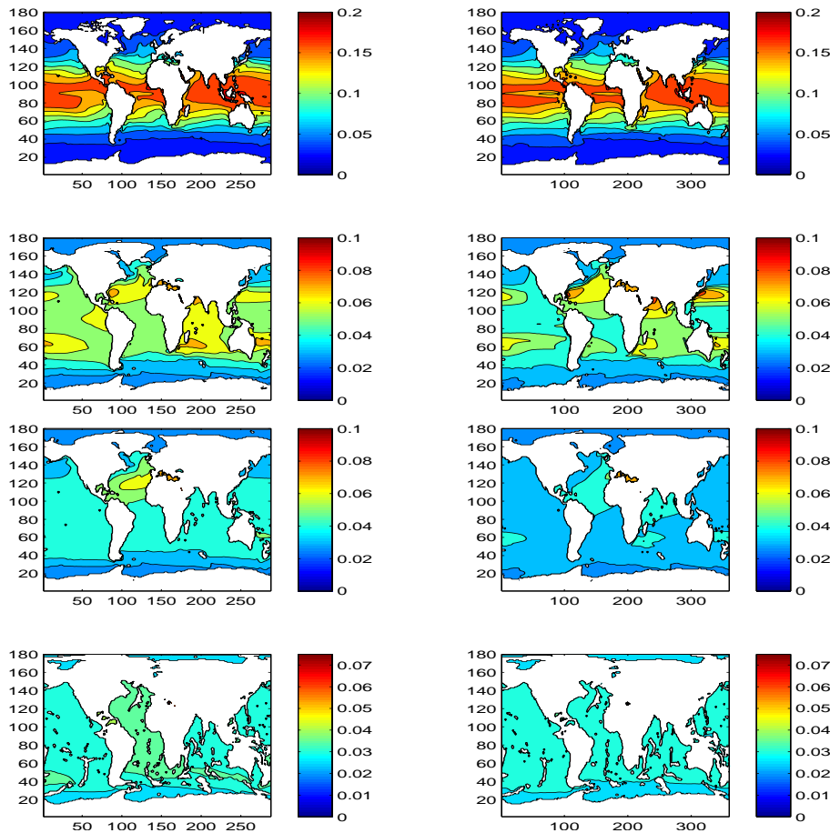
Fig. 2. Effective remineralization rate at surf, 500 m, 1000 m and 3000 m for \alpha = 0.1 \text{ d}^{-1} (the low remin. case). The left column is for the GISSER model and the right column for GISSEH.
