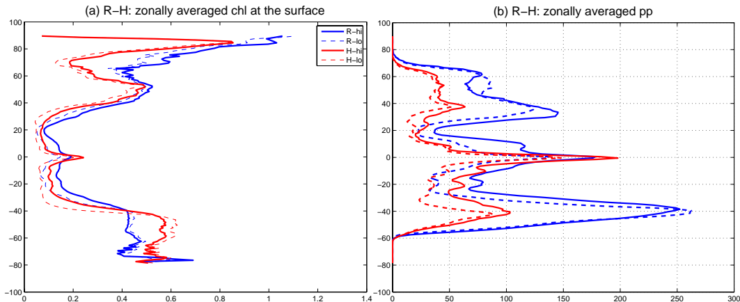
Fig. 6. Zonally averaged (a) total chlorophyll at the surface and (b) primary productivity vertically integrated. Continuous lines are for high remineralization rate and dashed for low remineralization rate. Blue lines are for GISSER and red lines for GISSEH. Units are \text{mg C m}^{-3} .
