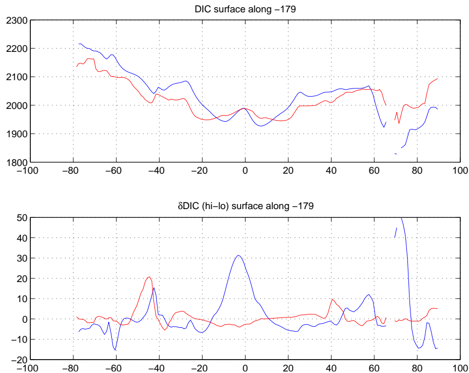
Fig. 10. Surface DIC and \delta DIC (high remin-low remin) along the 179W meridian. Unts are in \text{mmol C m}^{-3} .
