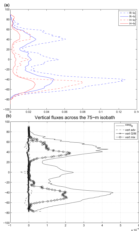
Fig. 7. (a) Zonally integrated carbon export at 75 m in \text{PgCyr}^{-1} . Color scheme is same as in previous figures. (b) Zonal mean vertical fluxes across 75 m depth for the Russell model: carbon export (R-lo, continuous line), vertical advection flux (multiplied by 10, dashed line), vertical flux associated with the Gent-McWilliams scheme (multiplied by 10, solid line with crosses) and vertical flux associated with vertical mixing (multiplied by 10, solid-circle line). All fluxes are positive down.
