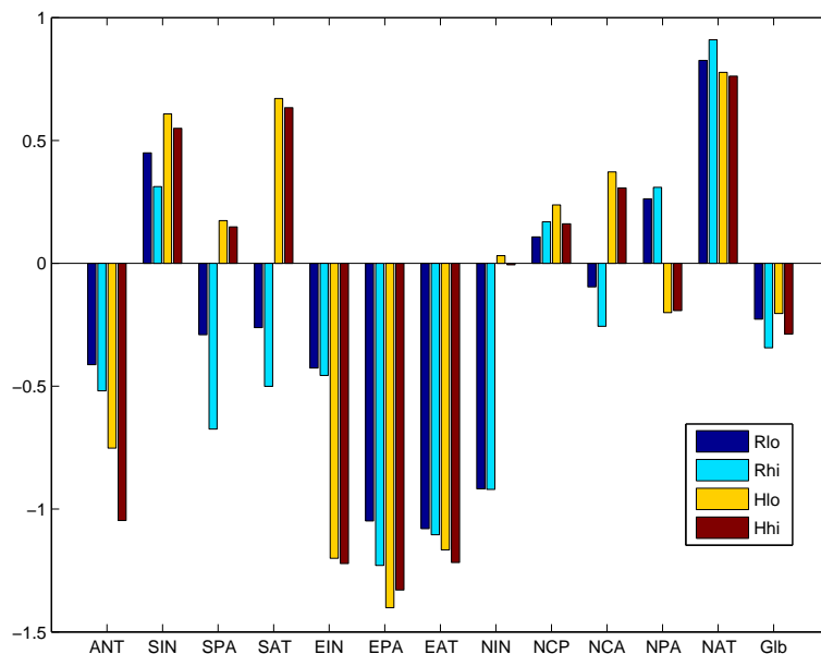
Fig. 13. Regional fluxes (in \text{mmol C m}^{-2} \text{yr}^{-1} ). The values are scaled to take into account the different areas of the regions.
