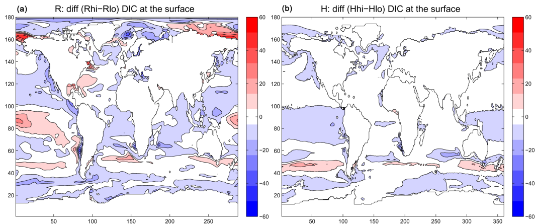
Fig. 9. DIC differences between the high and low remineralization runs in (a) GISSER and (b) GISSEH. Units are \text{PgCyr}^{-1} .
