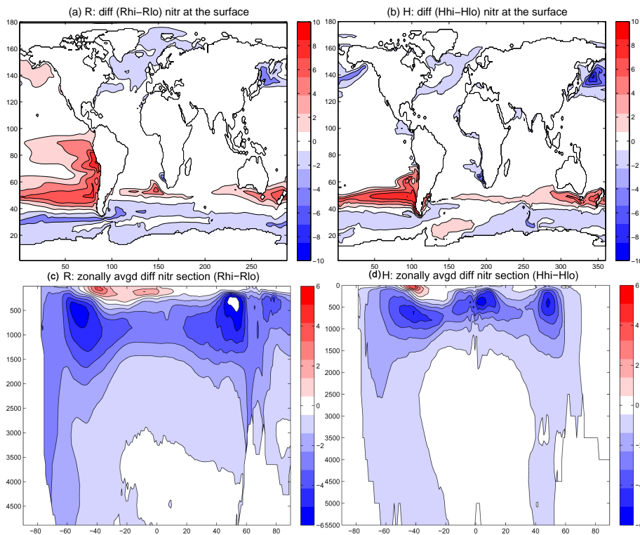
Fig. 4. (a, b) Surface distributions of \delta Nitrate in (a) the GISSER and (b) the GISSEH models at equilibrium. \delta Nitrate is defined as the difference between nitrate in the high and the low remineralization cases. Units are in \text{mmol N m}^{-3} . (c, d) Zonally averaged vertical sections of \delta nitrate defined as the difference in nitrate between high and low remineralization rates in the (a) GISSER and (b) GISSEH models. Units are in \text{mmol N m}^{-3} .
