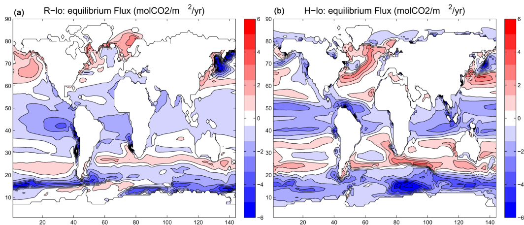
Fig. 12. Equilibrium flux ( \text{molCO}_2\text{m}^{-2}\text{yr}^{-1} ). Red denotes uptake, blue denotes outgassing. Unshaded regions the flux is low. These are results from the two runs R and H using different remineralization scales. 06 refers to high remineralization rate (i.e. fast recycling of nutrients) and 08 refers to low remineralization rate.
