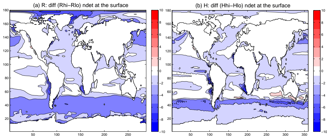
Fig. 1. Surface distributions of \delta\text{Detritus} in (a) the GISSER (shorthand: R) and (b) the GISSEH (shorthand: H) models at equilibrium. \delta\text{Detritus} is defined as the difference between detritus in the high (hi) and the low (lo) remineralization cases. Units are \text{milligrams C m}^{-3} .
