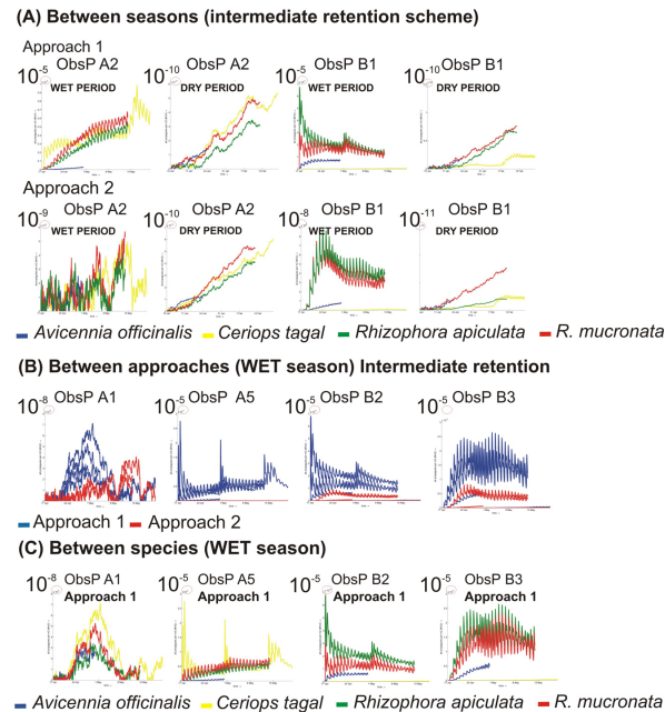
Fig. 8. Results of scenario 4 (the effect of dike removal) showing the time-series plots of Avicennia officinalis , Ceriops tagal and Rhizophora apiculata and Rhizophora mucronata . A comparison was made between (A) seasons (wet vs. dry season), (B) approaches of outer dike removal (In approach 1 60 m of an outer dike was removed at the north-eastern side of shrimp farm A and the northern side of shrimp farm B, while in approach 2 part 60 m of the outer dike at the south-eastern side of shrimp farm A and the north-western side of shrimp farm B was removed) and (C) the different species. ObsP Ax = observation point in shrimp farm area A, ObsP Bx = observation point in shrimp farm area B. X-axes = buoyancy period (days), Y-axes = propagule density \text{m}^{-2} .
