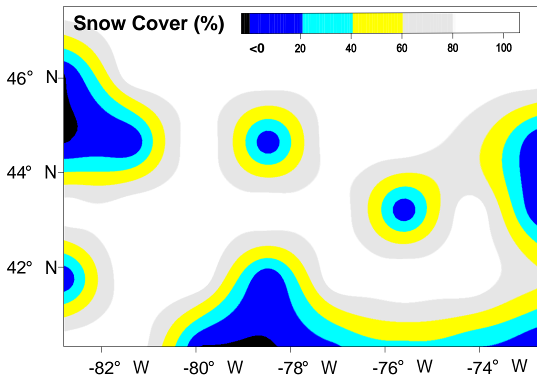
Fig. S2: Satellite image data of snow covering across southern Ontario in February 2007 (data was from http://neo.sci.gsfc.nasa.gov/Search.html? ).
