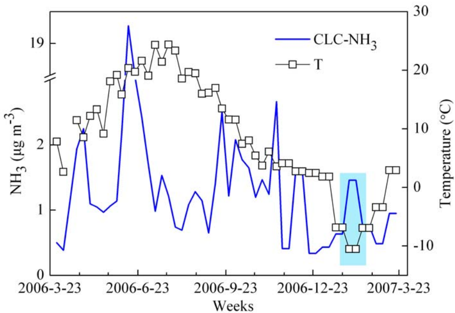
Fig. S3: Temporal variation of \text{NH}_3 at CLC in 2006-2007.
