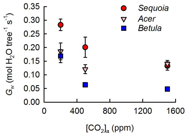
Fig. 6. [CO 2 ] a -regulated canopy conductance to water vapour. Whole canopy transpiration rates (G w ) increase with declining [CO 2 ] a . Values are means ±s.e.m. (n = 3).
