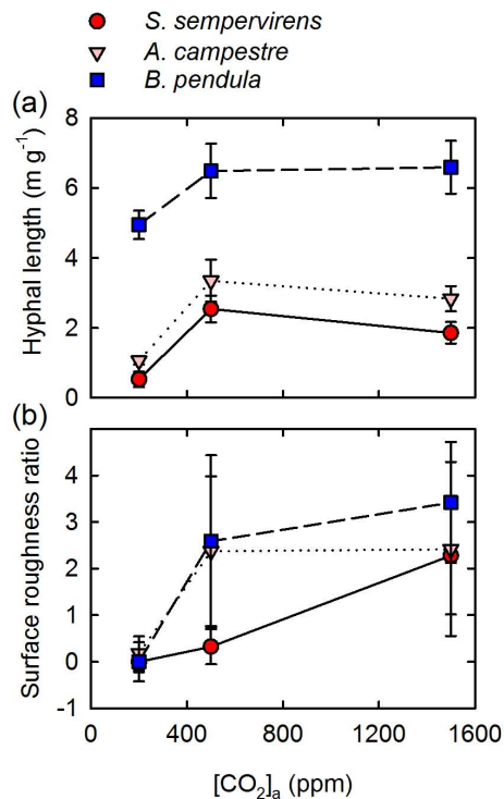
Fig. 1. [CO 2 ] a -regulated hyphal colonisation and mineral surface alteration. (a) Mycorrhizal hyphal lengths colonising basalt grains and (b) muscovite roughness ratios, decrease with falling [CO 2 ] a . All values are mean ± s.e.m.
