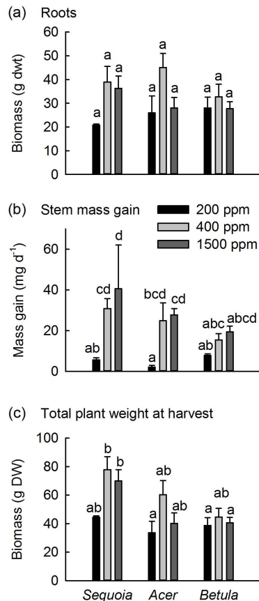
Fig. 4. Root biomass (a) , calculated stem mass gain (b) (a proxy for net primary production) and measured total plant biomass (c) at the end of the experiment. Values are mean \pm s.e.m ( n = 3 ). Bars sharing the same letter are not statistically different at P > 0.05 (two-way ANOVA testing for effects of species and [CO 2 ] a with Tukey multiple comparisons).
