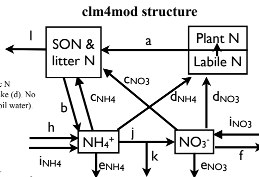
Fig. 3. Overview of the clm4cn and clm4mod model structure.
