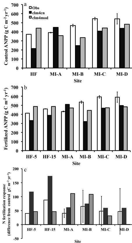
Fig. 1. Mean annual aboveground net primary production (ANPP) for the five temperate deciduous forests in Table 1. The measured values, clm4cn model predictions, and clm4mod model predictions are shown for (a) the control (non-fertilized) plots and (b) the nitrogen fertilized plots, along with (c) the differences between the control and fertilized treatments. The model simulations include transient nitrogen deposition, atmospheric CO 2 , and land-use. Error bars represent the S. E. reported in Pregitzer et al. (2008).
