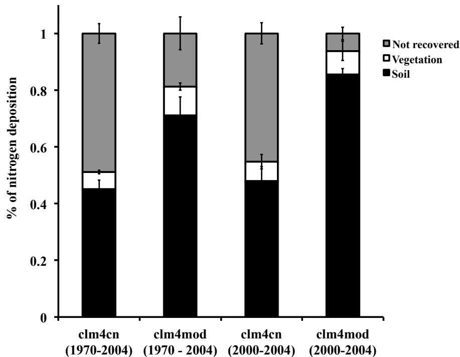
Fig. 2. Model predictions of ecosystem retention of nitrogen deposition, partitioned among soil organic matter and vegetation averaged across all five sites for two time periods: 1970–2004 and 2000–2004. Error bars represent variation among sites (1 S.E.).
