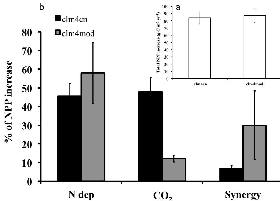
Fig. 5. Model predictions of net primary production (NPP) response to rising nitrogen deposition and atmospheric CO 2 averaged across all five sites. The total NPP increase between 1850 and 2004 (a; inset) is partitioned into the increase due only to nitrogen deposition, only to CO 2 fertilization, and the synergy between nitrogen deposition and CO 2 fertilization. Error bars represent variation among sites (1 S.E.).
