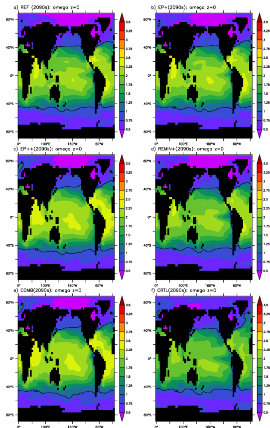
Fig. 5. Annual mean surface aragonite saturation state during the 2090–2100 period for (a) REF; (b) EP+; (c) EP++; (d) REMIN+; (e) COMB and (f) CTRL simulations.
