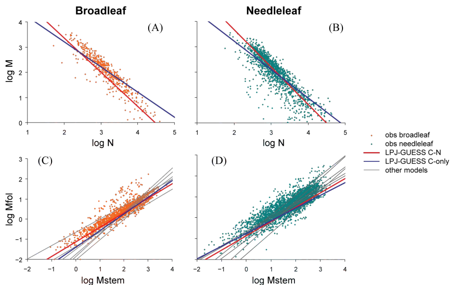
Fig. 5. Component biomass allometry for broadleaf-dominated ( A, C ) and needleleaf-dominated ( B, D ) grid cells from C-N and C-only simulations superimposed on data for forest stands from the Cannell (1982) and Usoltsev (2001) databases. Curves are fitted to model data from the 0.5^\circ \times 0.5^\circ grid cells encompassing stand coordinates from the observed databases. Allometric relationships from the land surface models considered by Wolf et al. (2011) (grey curves) are reproduced from that paper. N = tree population density ( \text{ha}^{-1} ); M = total biomass of average tree (kg); M_{\text{fol}} = foliage biomass of average tree (kg); M_{\text{stem}} = stem biomass of average tree (kg).
