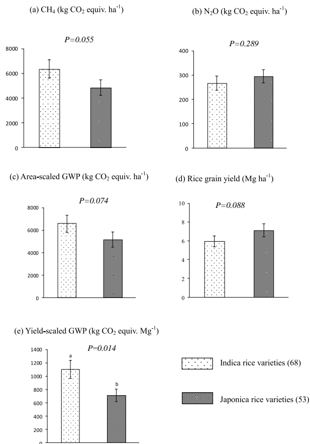
Fig. 1. Impacts of cropping systems on CH 4 and N 2 O emissions, area-scaled GWP, rice grain yield, and yield-scaled GWP during rice varieties types. The data in the bracket was the numbers of observation. All error bars represented 95% confidence intervals. Alphabet was refer to significant treatment effects in ANOVA at P \leq 0.05 .
