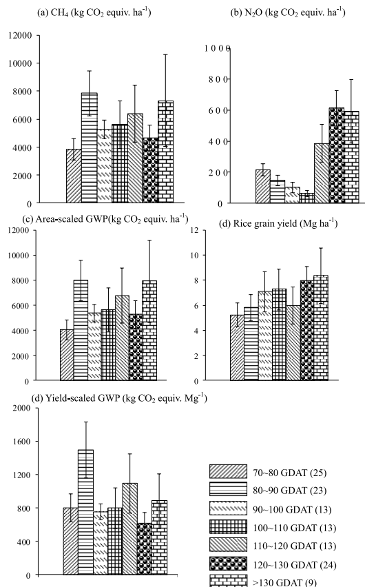
Fig. 2. Impacts of cropping systems on \text{CH}_4 and \text{N}_2\text{O} emissions, area-scaled GWP, rice grain yield, and yield-scaled GWP during different growth duration after transplanting (GDAT). The data in the bracket was the numbers of observation. All error bars represented 95 % confidence intervals.
