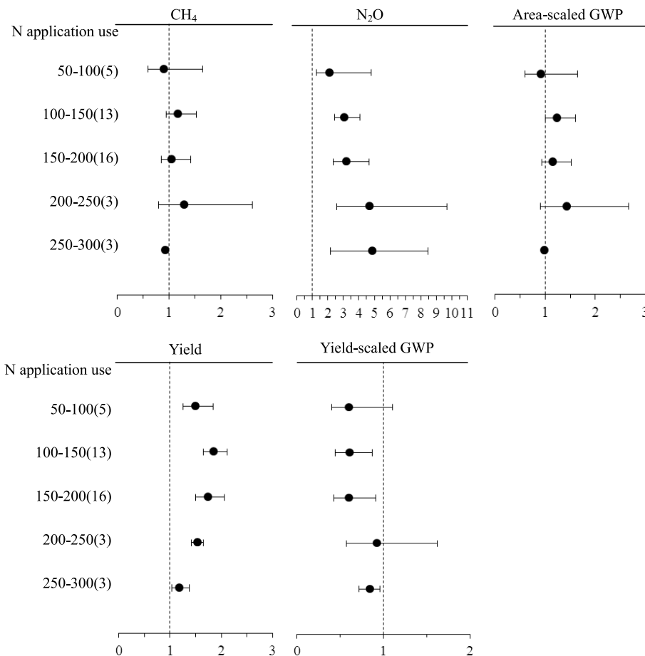
Fig. 3. Effects of different N application rates on CH 4 and N 2 O emissions, area-scaled GWP, rice yield, and yield-scaled GWP. The data were expressed as mean response ratios with 95% confidence intervals, and the numbers of observations included were indicated in parentheses.
