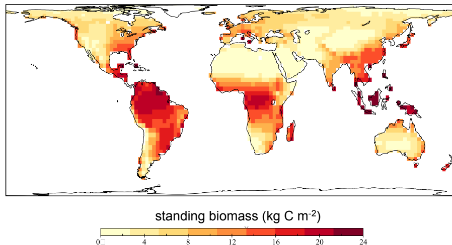
Fig. 7. Carbon in terrestrial vegetation biomass of the control run. In this scenario the vegetation growth is constrained only by water, light, and temperature so that vegetation biomass reaches its maximum everywhere around the globe, while not accounting for P limitation. In this simulation biomass reaches 24 \text{ kg C m}^{-2} in some tropical areas.
