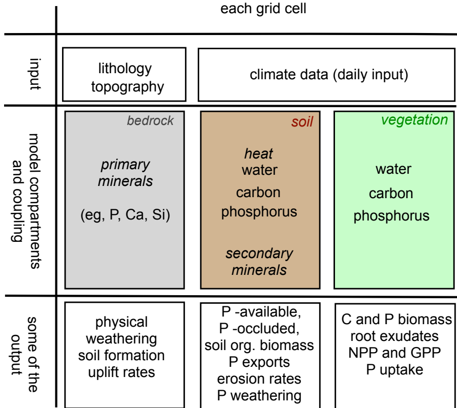
Fig. 3. Diagram of the model structure (after Porada et al., 2010). The model uses daily climate data, topography and lithological classes as input. It has three main components, bedrock, soil and vegetation in which fluxes of primary minerals from the bedrock are calculated. Vegetation dynamics drives water, carbon, and phosphorus dynamics. The model calculates e.g., weathering rates, gross primary productivity, and biomass production. For an extensive list of the model outputs refer to Table 4
