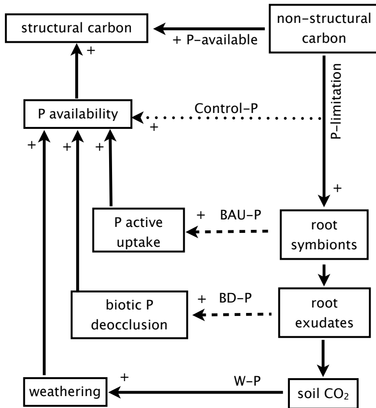
Fig. 6. Diagram showing the modeled carbon feedbacks on the P availability. Simulation scenarios are defined with respect to these feedbacks. Dashed line represents the effects that can be turned off and pointed line represents the unrealistic Control-P.
