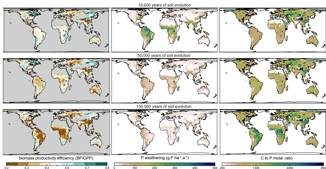
Fig. 12. Biomass production efficiency (BPE), P weathering rates, and C to P molar ratio in vegetation changes during pedogenesis. Top plots represent the dynamics in recent soils (after about 10 000 yr of soil evolution). The intermediate plots represent intermediate soil ages of about 50 000 yr and the bottom plots represent old soils about 150 000 yr of soil evolution. Biomass production is more efficient in temperate regions in both, young and old, soils. In tropical regions, BPE decreased in time, reaching a status of very low efficiency, particularly in central Africa and Western South America. P weathering rates (central panels), decrease everywhere with time. In the oldest soils, weathering is high in places at high elevations. Also locations with shale lithology produced relatively high weathering rates, compared to those with sandstone. The C to P molar ratio in vegetation increased in time. In tropical regions, the ratio was correlated with weathering rates.
