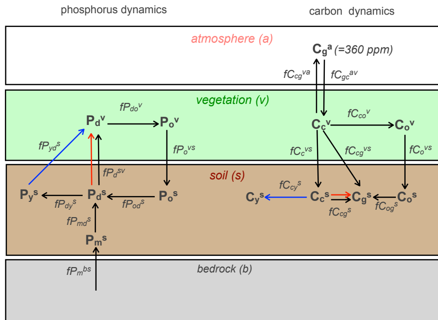
Fig. 4. The C-P biogeochemical model: symbols in bold denote pools and symbols, in italic denote fluxes between pools. Black arrows show fluxes in the standard version of the model (W-P); blue arrows show P de-occlusion and the associated carbon flux to recalcitrant forms (BD); red arrows show P active uptake mediated by mycorrhizae and its associated carbon respiration (BAU). The model has a switch for turning on and off active P uptake (blue fluxes) and biotic de-occlusion of P (red fluxes). For definition of symbols refer to Table 4
