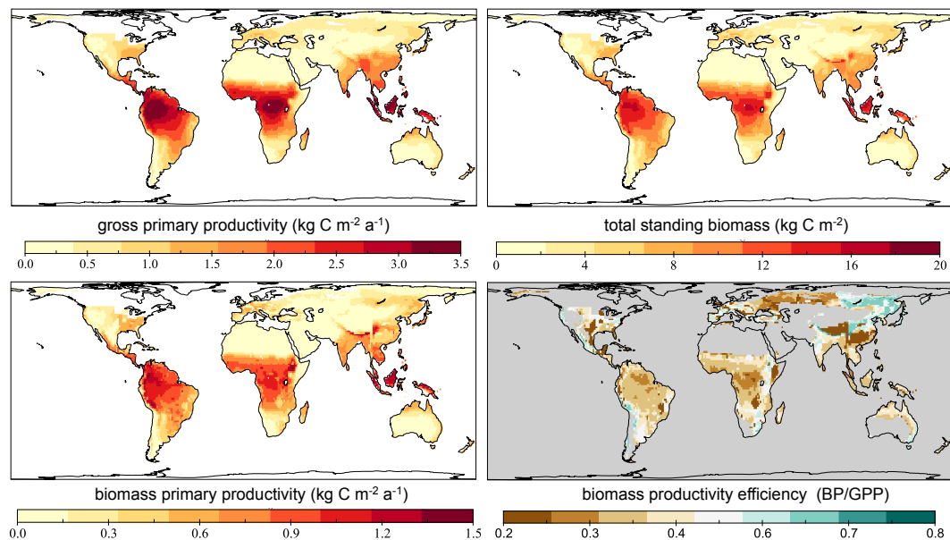
Fig. 11. Carbon fluxes and pools in vegetation considering active P vegetation uptake after 70 000 yr of soil evolution.
