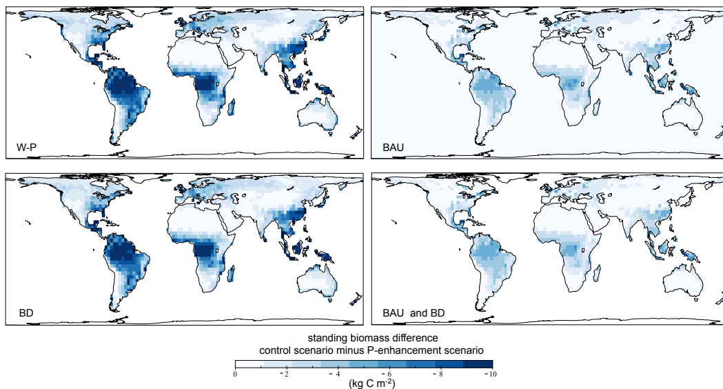
Fig. 8. Difference in the standing biomass of the control with the different feedback scenarios for the world after 50 000 yr of soil evolution. Biomass differences between the control simulation (see Fig. 7) and W-P (top-left), BD (bottom-left), BAU (top-right), BAU-BD (bottom right). W-P shows the greatest differences with the control scenario: more than 50 % biomass reduction worldwide, the differences are high in temperate coastal areas (e.g., Chile, Guyana, and South Africa). BD (bottom-left) shows a very similar pattern to the W-P scenario, with only small differences in temperate regions. Biotic active uptake (BAU) (top-right panel) shows much smaller differences to the control, with the absolute greatest differences located in the tropics. BAU-BD (bottom right) shows a pattern almost identical to the BAU scenario, with only very little differences.
