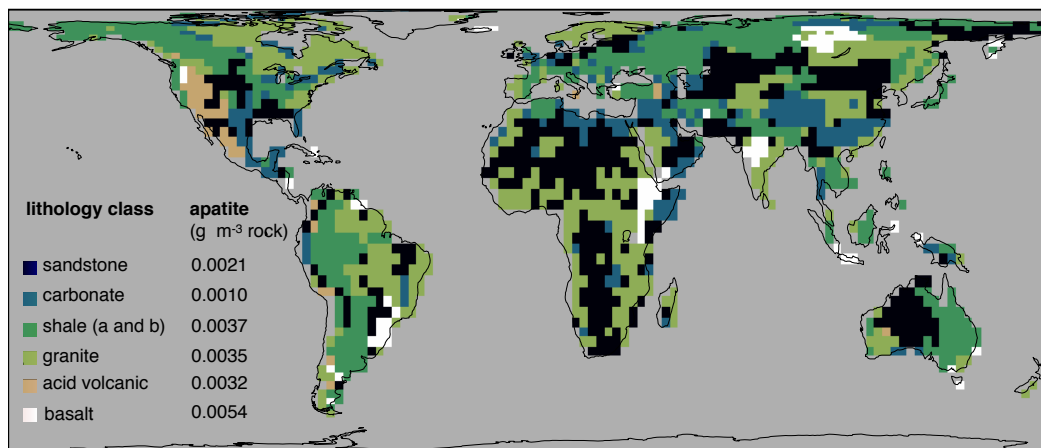
Fig. 5. Map of the lithological classes and their respective apatite concentrations ( \text{g Apatite m}^{-3} ). Lithological classes taken from Amiotte Suchet and Probst (1995), values for the concentration of apatite were calculated from Newman (1995).
