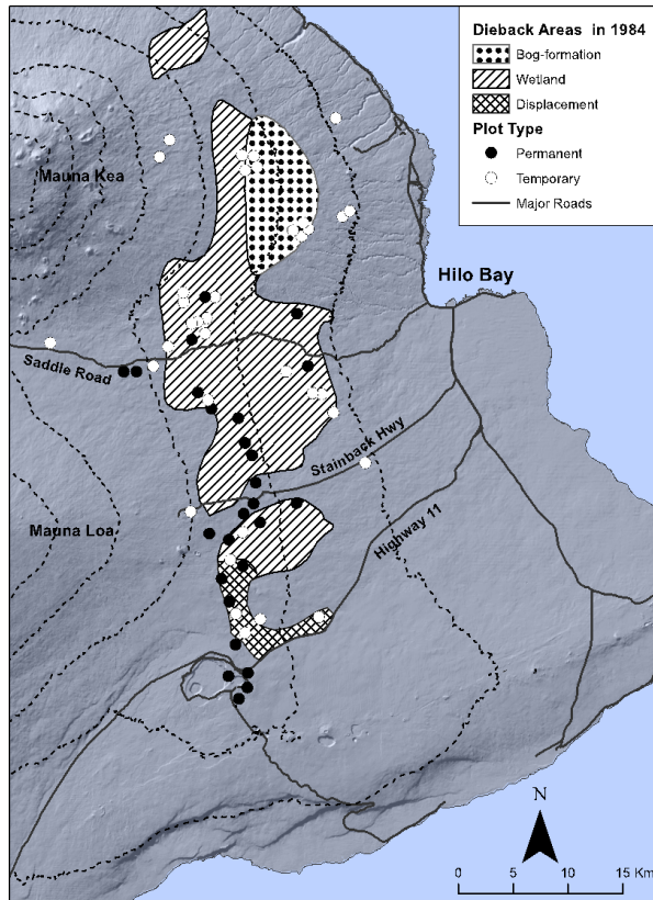
Fig. 9. The study area with plot locations. Black circles represent permanent plots (26/62). Three dieback types are shown. Dryland dieback refers to plots outside the mapped area, from the Saddle Road south into Hawaii Volcanoes National Park. Gap-formation dieback refers to plots on Mauna Kea in the wetland and bog-formation territory (map after Jacobi et al., 1983).
