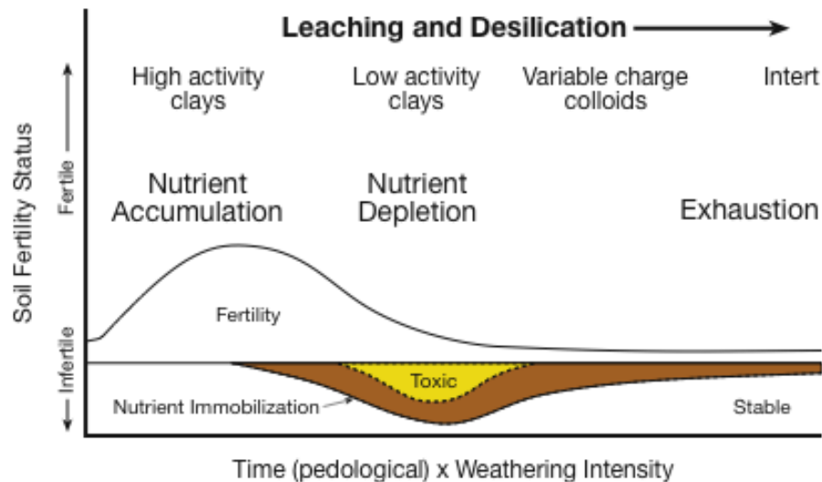
Fig. 14. Tropical soil formation and degradation, an independently designed conceptual model that matches the long-term primary successional model shown in Fig. 12 above. From Fox et al. (1991) with permission from Allertonia, a journal of the National Tropical Botanic Garden on Kaua'i Island.
