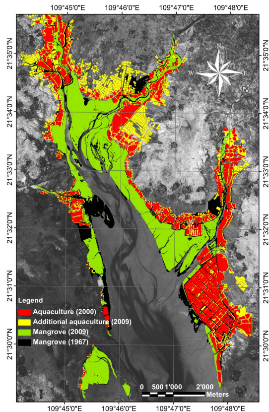
Fig. 2. Changes in the extent of Gaoqiao mangrove cover observed from 1967 (Corona) and 2009 (GeoEye-1) satellite data and expansion of aquaculture ponds observed from 2000 (Land-sat) and 2009 (GeoEye-1) satellite data (background: 1967 Corona imagery).
