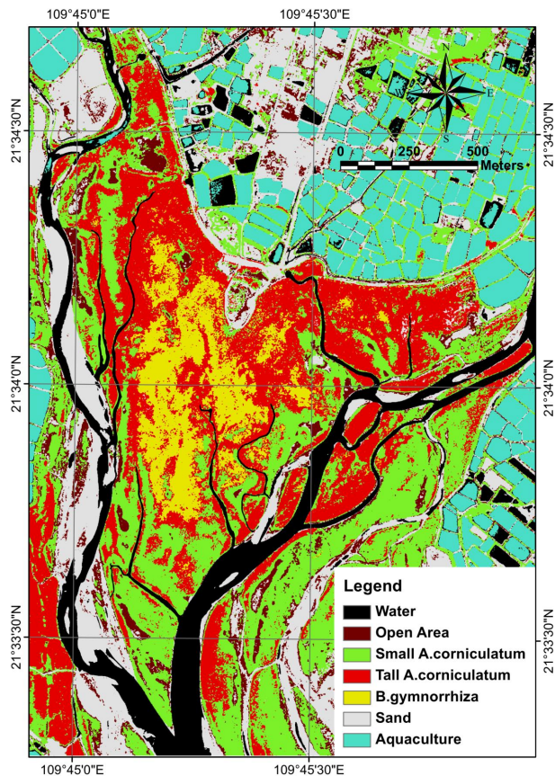
Fig. 4. Land-use/cover supervised classification of Gaoqiao based on the pansharpened multispectral GeoEye-1 (2009) image, and on the fieldwork transects shown in Fig. 1.
