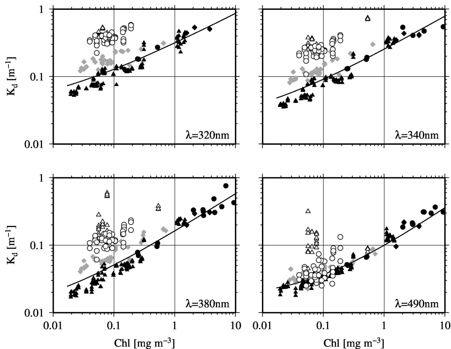
Fig. 9. K_d as a function of Chl a , and for selected wavelengths as indicated (redrawn from Morel et al., 2007a, with addition of the data from MALINA Leg2b). The open symbols are for the MALINA Leg2b clear water stations, the grey symbols for the Mediterranean Sea, and the black symbols for South Pacific data. The continuous black curve represents the MM01 prediction.
