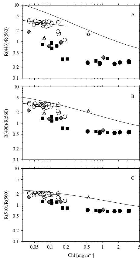
Fig. 7. Reflectance ratios for the wavelengths indicated, as a function of the Chl a concentration. The thick solid curves show modelled values from Morel and Maritorea (2001). The thin solid curves are linear fits using the log-transformed data, for the clear water stations only.
