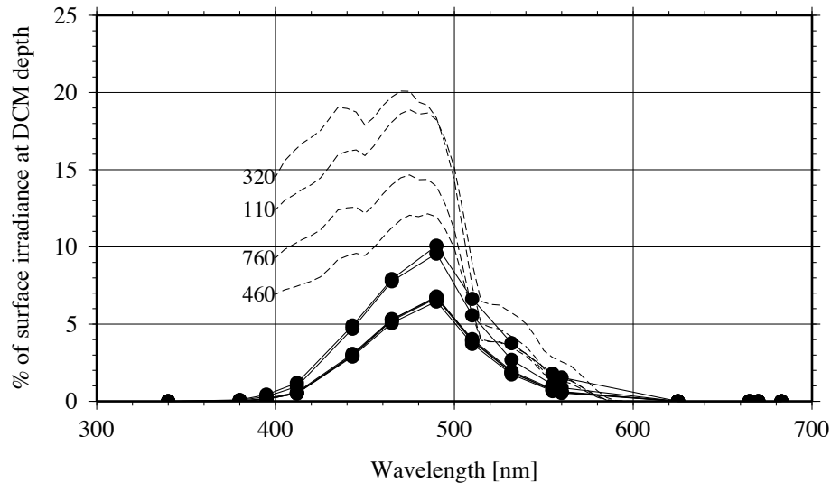
Fig. 11. Percentage of surface irradiance that reaches the depth of the deep chlorophyll maximum (DCM). The percentage is determined either from the radiometry profiles (black dots) or from MM01 (dashed curves) fed with the measured vertical Chl a profile.
