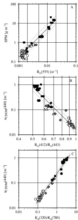
Fig. 8. Bio-optical relationships in the MALINA Leg2b data set. Solid curves are regression fits on the log-transformed data, and the dotted curves show the RMSE around the regressions (A) R_{rs} (555) nm as a function of SPM concentration, (B) Ratio of R_{rs} (412) to R_{rs} (443) as a function of CDOM absorption at 440 nm, (C) Ratio of K_d (320) to K_d (780), as a function of CDOM absorption at 440 nm.
