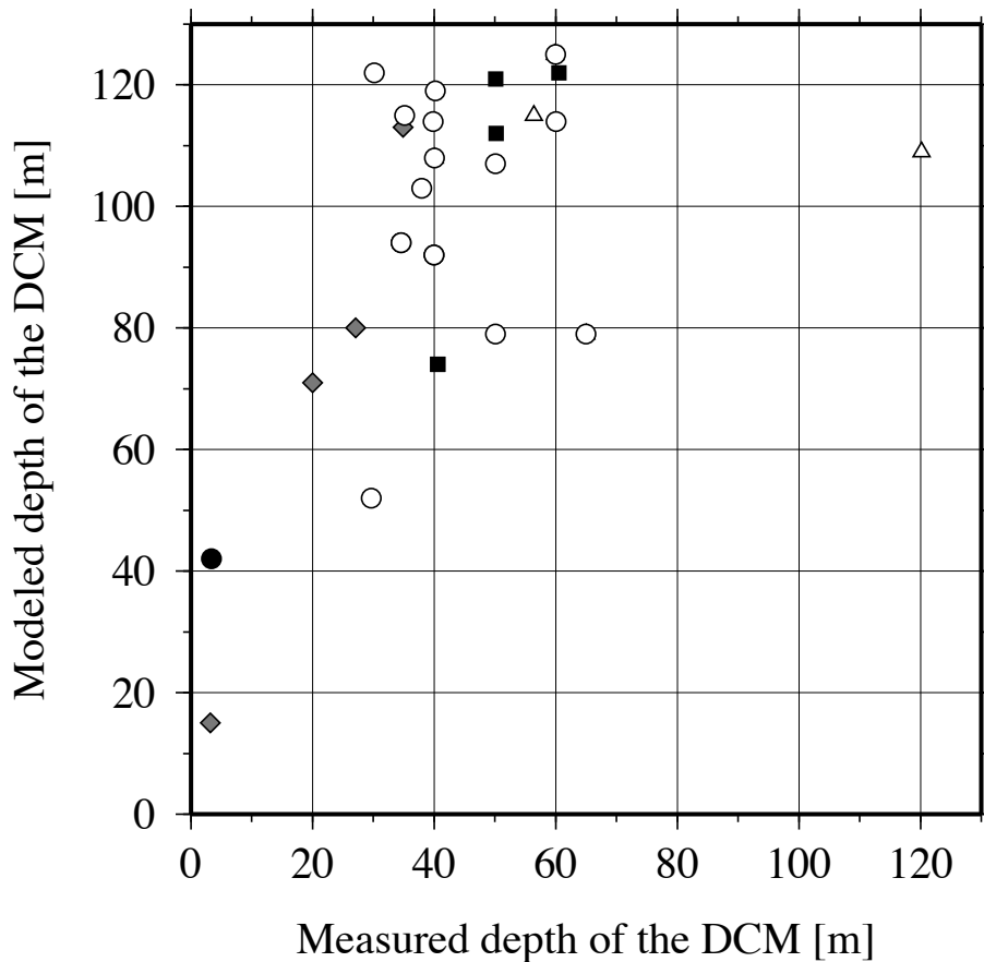
Fig. 10. Predicted versus measured depth of the deep chlorophyll maximum (DCM). Stations from the two river transects are excluded from this comparison because they do not exhibit a DCM (stations 395 to 398, and 691 to 695).
