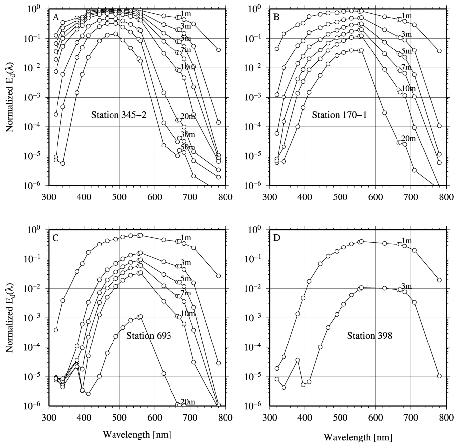
Fig. 3. Example spectra of the downward irradiance at various depths and four stations as indicated. Values are normalized to the maximum E_d found just below the sea surface.
