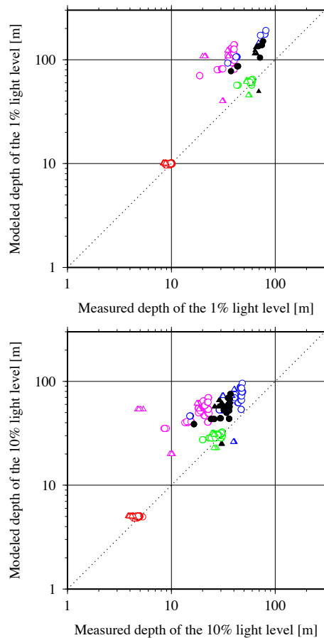
Fig. 12. Predicted (MM01) versus measured depth of the 1% (top) and 10% (bottom) light levels. Symbols are as for previous figures, i.e. circles for open ocean stations and triangles for ice-edge stations. Pink, blue, green, red, and black symbols are for \lambda = 380, 443, 555, 670 nm and PAR, respectively.
