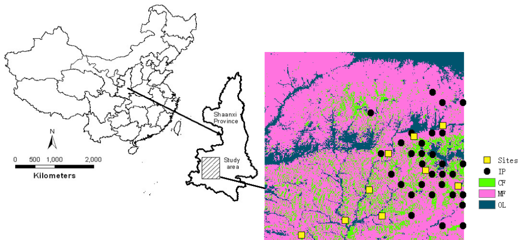
Fig. 2. Study area with the locations of ground sites in Qinling Mountain in southern Shaanxi Province in China.
