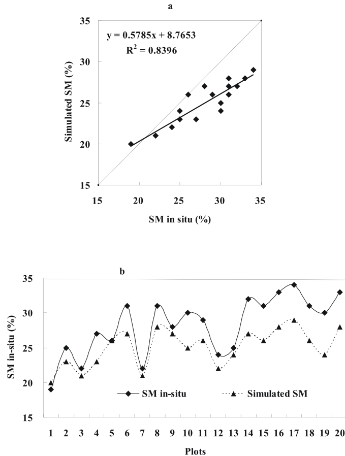
Fig. 5. Simulated soil moisture (SM) at 30 m resolution using BEPS-TerrainLab in comparison with measured SM using TDR during 1 July to 31 August in 2004 (a) ; comparison of BEPS-simulated SM with measured SM at various sites (b) . The solid line is the 1 : 1 line.
