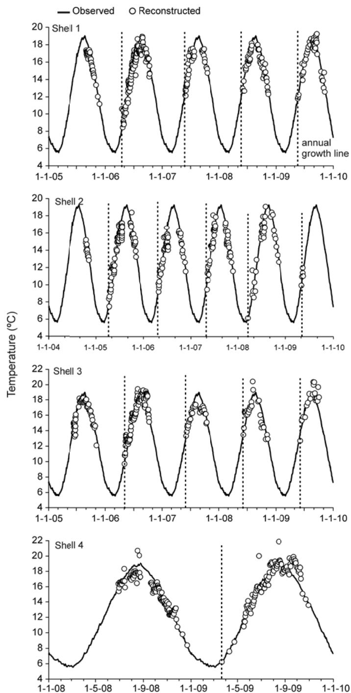
Fig. S2. Comparison of observed and reconstructed water temperatures experienced by E. directus during growth. Open circles represent reconstructed temperatures from measured \delta^{18}\text{O} values using Eq. [5] (see text), line represents observed temperatures in the field (from http://live.waterbase.nl/waterbase ). Vertical dotted lines represent annual growth lines observed on the surface of the shell and in the acetate peels.
