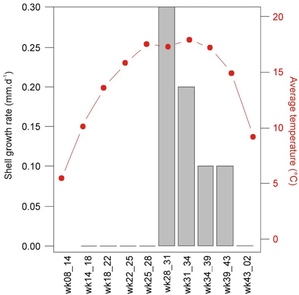
Fig. S3. Shell growth (mm.d -1 ) and water temperature (°C) measured in the field in 2011 (wk08_14: 22-02 to 07-04; wk14_18: 07-04 to 03-05; wk18_22: 03 to 31-05; wk22_25: 31-05 to 24-06; wk25_28: 24-06 to 12-07; wk28_31: 12-07 to 02-08; wk31_34: 02-08 to 23-08; wk34_39: 23-08 to 27-09; wk39_43: 27-09 to 25-10; wk43_02: 25-10 to 11-01-2012) (adapted from Witbaard et al., 2012).
