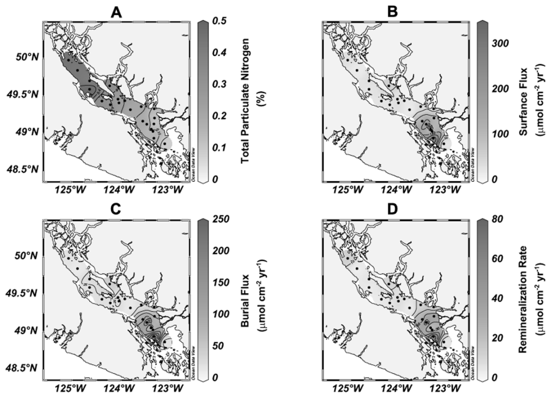
Fig. 3. A contour plot of sediment core data for the Strait of Georgia showing (A) total particulate nitrogen (PN) concentration (%) for surface sediment; (B) surface flux of PN ( 50 \mu\text{mol cm}^{-2} \text{yr}^{-1} interval); (C) burial flux of PN; and (D) remineralization rate of PN.
