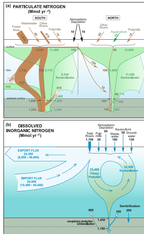
Fig. 4. Schematic diagrams of the nitrogen cycle in the Strait of Georgia showing (a) a budget for particulate nitrogen and (b) a budget for dissolved nitrogen (DIN). Northern and southern regions are presented separately in (a) to highlight the differences in the terrigenous particulate nitrogen contributions and sources. Brown arrows have been used to represent terrigenous ( PN_{Terr} ) fluxes and green arrows marine ( PN_{Mar} ) fluxes. Black arrows were used to represent atmospheric deposition.
