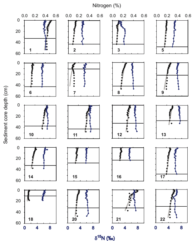
Fig. 2. Depth profiles for total particulate nitrogen concentration [PN] (black solid diamond) and \delta^{15}\text{N} composition of sediment (blue open diamond connected by solid line) for all 20 box cores used in this study. The horizontal dashed line for each sediment profile represents the burial depth (the depth at which the [PN] becomes approximately constant). The solid grey line that follows the [PN] depth profiles represents the theoretical exponential decay curve described in Sect. 2.2.4.
