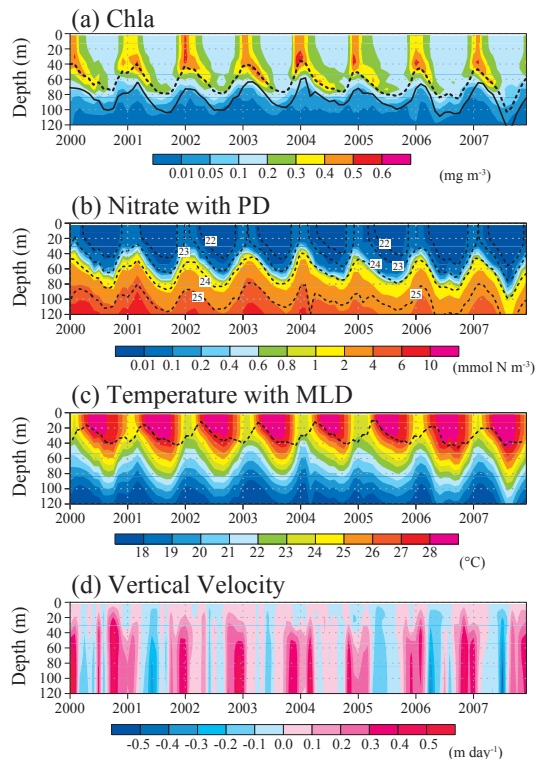
Fig. 5. Time series of simulated vertical distribution of (a) chlorophyll concentration ( \text{mg m}^{-3} ) with nutricline depth ( 1 \text{ mmol N m}^{-3} , dashed line) and thermocline depth ( 20^\circ\text{C} , solid line), (b) nitrate concentration ( \text{mmol N m}^{-3} ) with potential density (dashed line), (c) temperature ( ^\circ\text{C} ) with mixed layer depth (dashed line), and (d) vertical velocity ( \text{m day}^{-1} ) averaged for Box-L (northwestern Luzon, L in Fig. 1) during 2000-2007.
