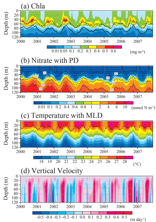
Fig. 6. Same as for Fig. 5, but for Box-V (southeast Vietnam, V in Fig. 1).
