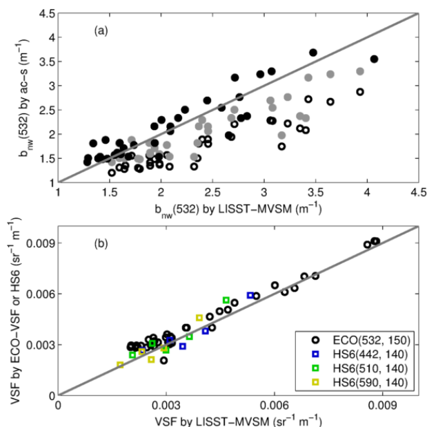
Fig. 3. Intercomparison between different instruments measuring scattering properties. (a) The comparisons of b_{\text{nw}}(532) estimated from the ac-s and LISST-MVSM. Two scattering corrections were progressively applied to (1) a_{\text{nw}}(532) to correct for scattering at angles from 41^\circ to 180^\circ that ac-s a-meter could not measure and (2) the LISST-MVSM based b_{\text{nw}}(532) with integration only down to 0.93^\circ to match the acceptance angle of ac-s c-meter. Open circles: neither correction was applied; grey circles: the 1st correction; black circles: both corrections. (b) The comparison of the LISST-MVSM \beta(\lambda, \theta) with ECO-VSF data measured at 150^\circ at 532 nm and with HydroScat-6 at 140^\circ for three wavelengths of 442, 510 and 590 nm. For comparison with HydroScat-6 data, the spectral VSF values at the corresponding wavelengths were used.
