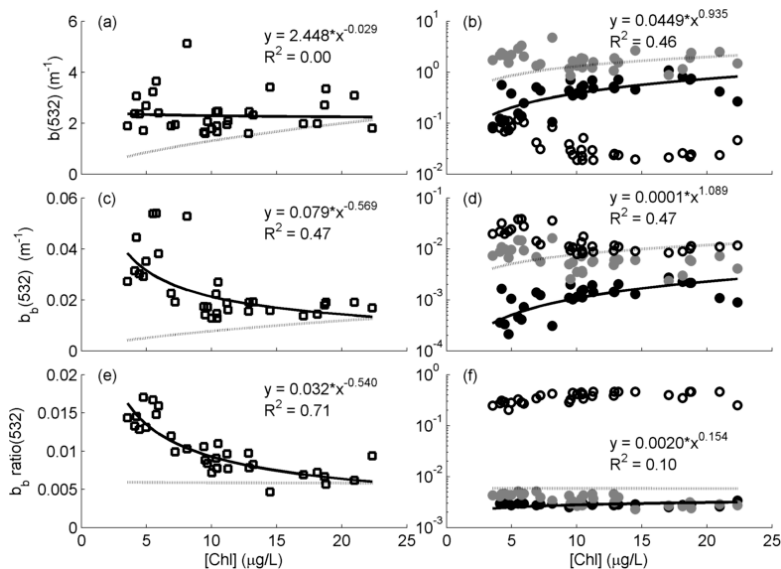
Fig. 6. Relationships of [Chl]_{HPLC} with the scattering coefficient (a and b), the backscattering coefficient (c and d), and the backscattering ratio (e and f). Open squares (left column) are the bulk parameters estimated directly from the measured VSFs. Open circles, grey circles and black circles (right column) are the variables for the particle groups of VSP, NAP and PHY, derived from the VSF-inversion. The dotted gray line in each panel represents the corresponding open ocean water model from Huot et al. (2008). The solid line in each panel represents a power-law regression against [Chl]_{HPLC} of b_{nw}(532) , b_{bnw}(532) or \tilde{b}_{bnw}(532) in (a, c and e) respectively or of b_{PHY}(532) , b_{bPHY}(532) or \tilde{b}_{bPHY}(532) in (b, d and f) respectively. The equation of this power-law regression and the corresponding coefficient of determination ( R^2 ) are also shown in each panel.
