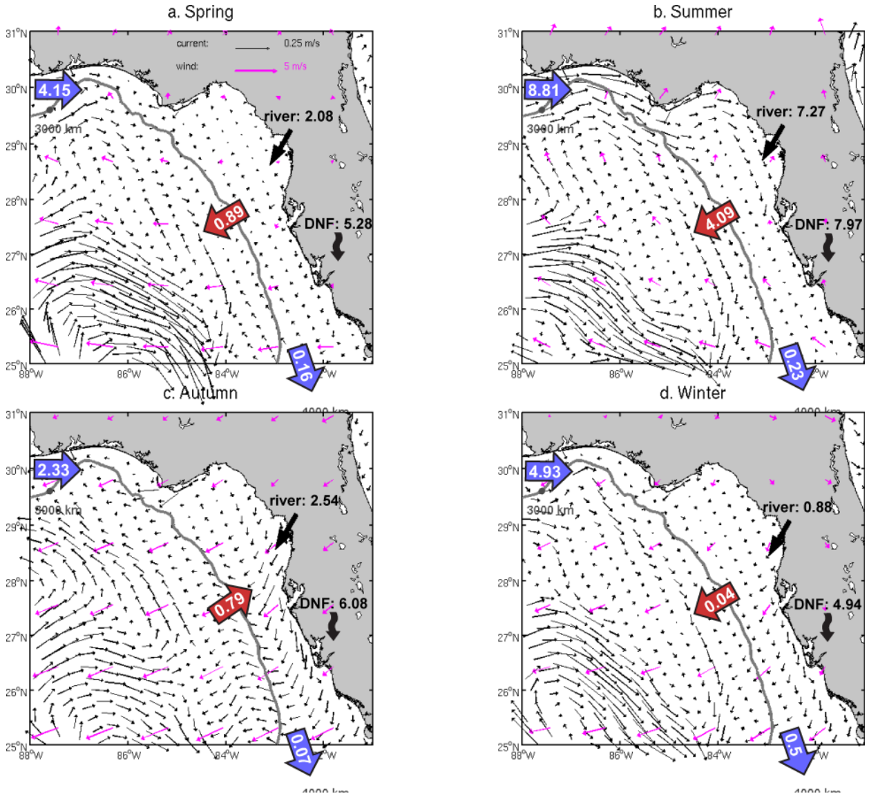
Fig.16 Similar with Fig.13 but for the west Florida shelf.
