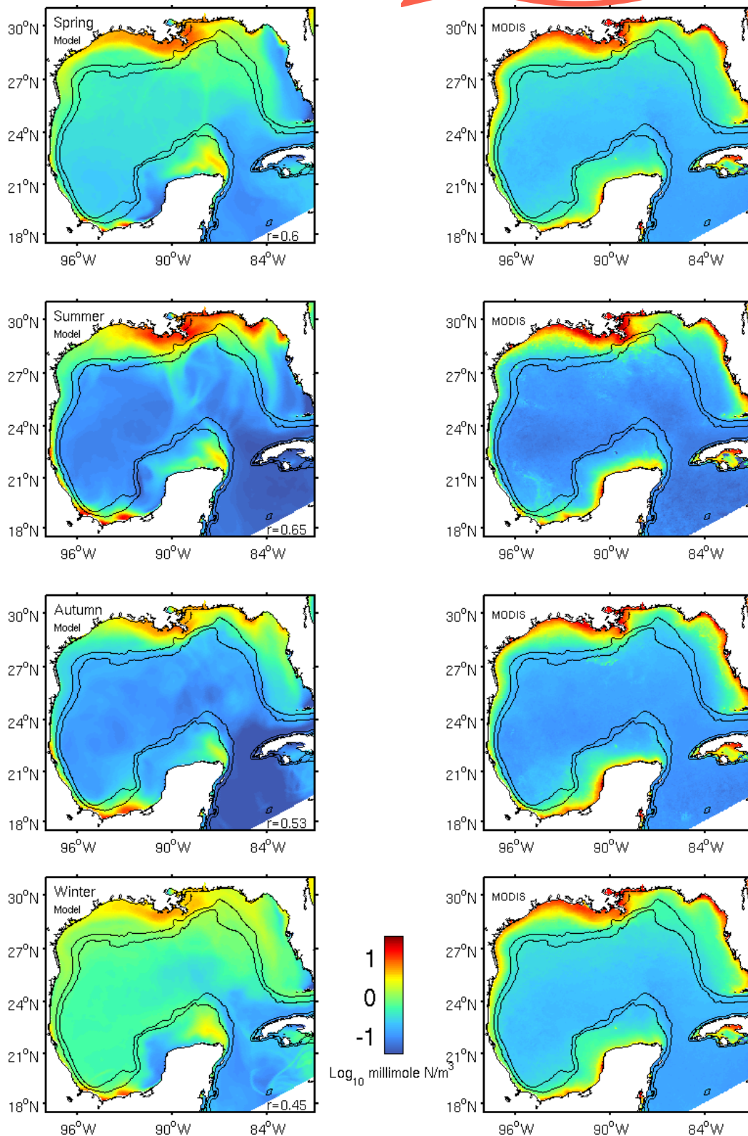
Fig. 8 Comparison of simulated (left panel) and observed (right panel) seasonal mean surface chlorophyll. Also shown are bathymetry contours (200 and 1000 m isobaths shown in black. BUT, since most of the context used the 50m isobath, why not draw that one?)
