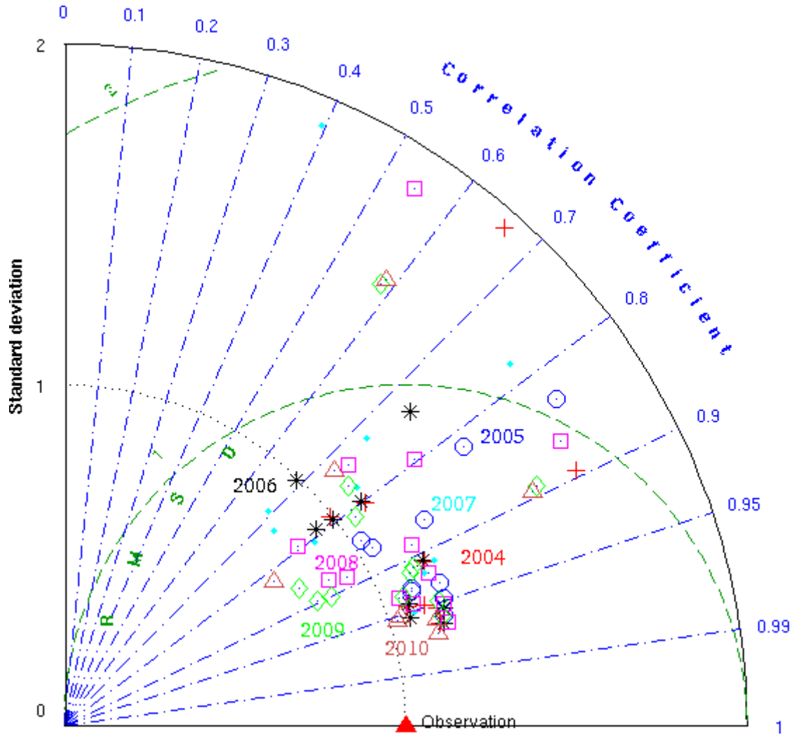
Fig. 4 Taylor Diagram for model simulated and observed sea-level anomaly at 13 tidal stations from 2004 to 2010. Radial distance represents the ratio of simulated to observed standard deviations, and azimuthal angle represents model-data correlation. Green arcs represent centered root mean square difference between model and data.
