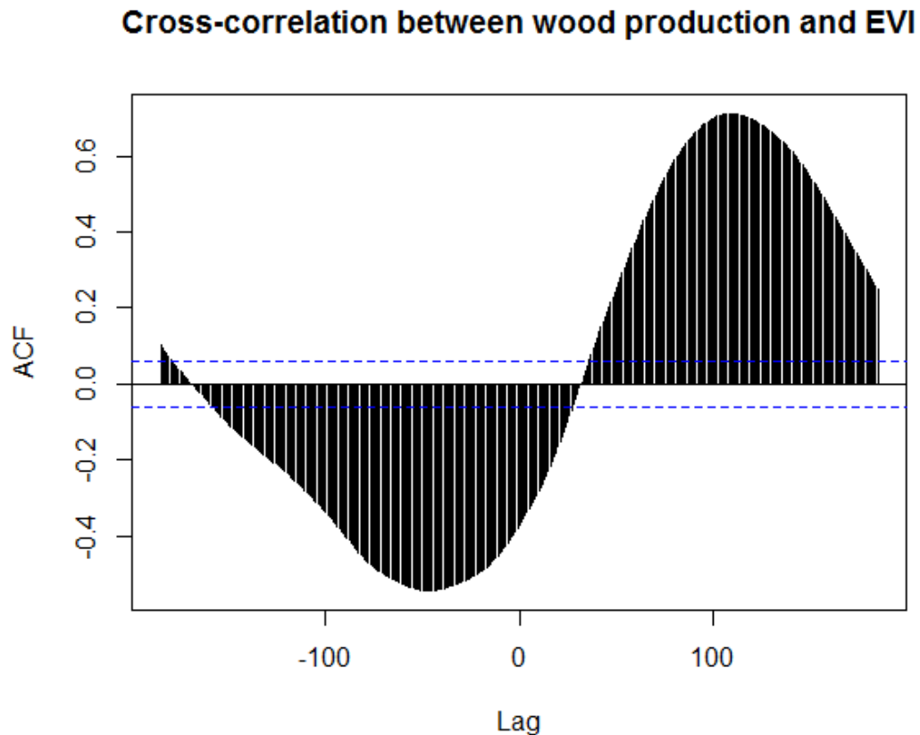
Fig. 5. Cross-correlation between wood production ( \Delta\text{AGB} ) and EVI. In the article we only report the maximum positive and negative coefficient of correlation ( \text{cor}+ and \text{cor}- ). In blue the CI limit.
